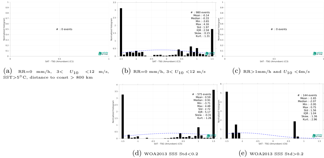
Figure 15: Normalized histogram of \Delta SSS (SMOS SSS L2Q v333 - 0.25 Deg (CATDS-CPDC) - TSG (Amundsen)) for 5 different subdatasets corresponding to: RR=0 mm/h, 3 < U_{10} < 12 m/s, SST>5°C, distance to coast > 800 km (a), RR=0 mm/h, 3 < U_{10} < 12 m/s (b), RR>1mm/h and U_{10} < 4 m/s (c), WOA2013 SSS Std<0.2 (d), WOA2013 SSS Std>0.2 (e).
