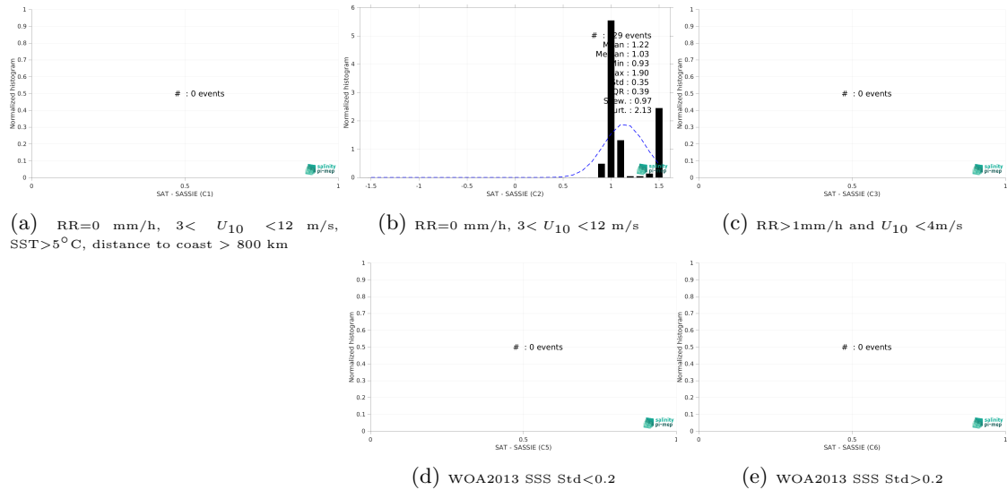
Figure 15: Normalized histogram of \Delta SSS (SMOS SSS L2Q v333 - 0.25 Deg (CATDS-CPDC) - SASSIE) for 5 different subdatasets corresponding to: RR=0 mm/h, 3 < U_{10} < 12 m/s, SST > 5°C, distance to coast > 800 km (a), RR=0 mm/h, 3 < U_{10} < 12 m/s (b), RR > 1mm/h and U_{10} < 4 m/s (c), WOA2013 SSS Std < 0.2 (d), WOA2013 SSS Std > 0.2 (e).
