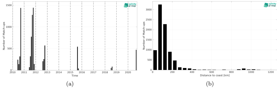
Figure 2: Number of match-ups between TSG (SAMOS) and SMOS SSS L3 v332 - 9 Days (CATDS-CPDC) SSS as a function of time (a) and as function of the distance to coast (b) over the Arctic Ocean Pi-MEP region and for the full satellite product period.
