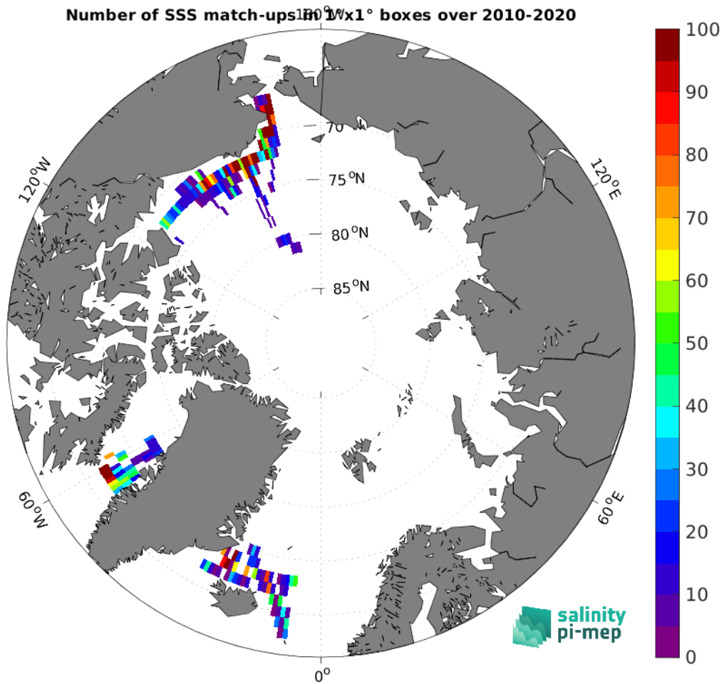
Figure 5: Number of SSS match-ups between TSG (SAMOS) SSS and the SMOS SSS L3 v332 - 9 Days (CATDS-CPDC) SSS product for the Arctic Ocean Pi-MEP region over 1^\circ \times 1^\circ boxes and for the full satellite product period.
