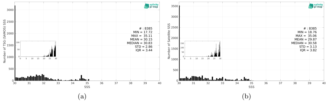
Figure 3: Histograms of SSS from TSG (SAMOS) (a) and SMOS SSS L3 v332 - 9 Days (CATDS-CPDC) (b) considering all match-up pairs per bins of 0.1 over the Arctic Ocean Pi-MEP region and for the full satellite product period.
