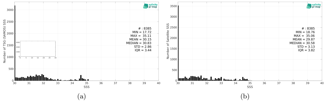
Figure 2: Histograms of SSS from TSG (SAMOS) (a) and SMOS SSS L3 v332 - 9 Days (CATDS-CPDC) (b) considering all match-up pairs per bins of 0.1 over the Arctic Ocean Pi-MEP region and for the full satellite product period.
