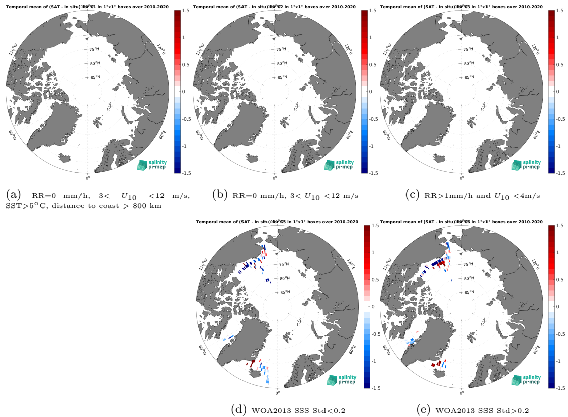
Figure 12: Temporal mean gridded over spatial boxes of size 1^{\circ}\times 1^{\circ} of \Delta\text{SSS} (SMOS SSS L3 v332 - 9 Days (CATDS-CPDC) - TSG (SAMOS)) for 5 different subdatasets corresponding to:RR=0 mm/h, 3 < U_{10} < 12 m/s, SST >5^{\circ}\text{C} , distance to coast > 800 km (a), RR=0 mm/h, 3 < U_{10} < 12 m/s (b), RR >1 mm/h and U_{10} < 4 m/s (c), WOA2013 SSS Std <0.2 (d), WOA2013 SSS Std >0.2 (e).
