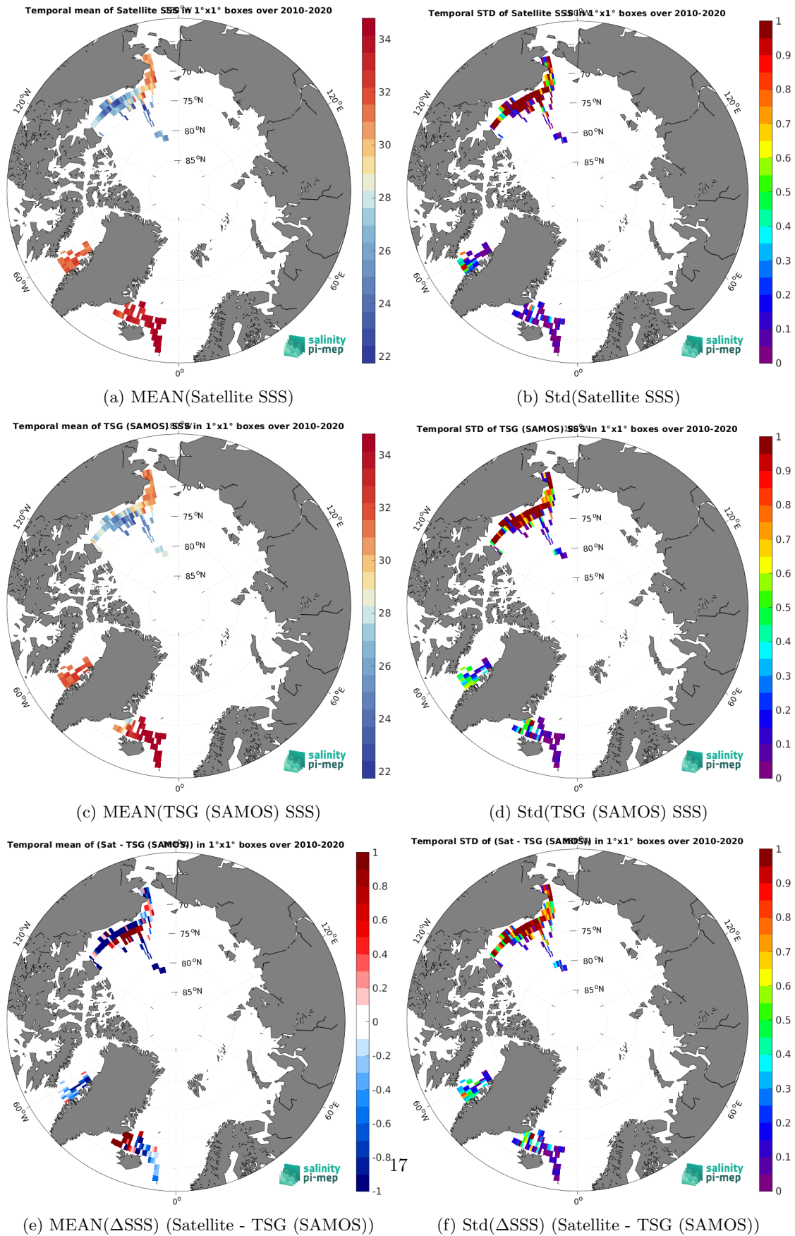
Figure 6: Temporal mean (left) and Std (right) of SSS from SMOS SSS L3 v332 - 9 Days (CATDS-CPDC) (top), TSG (SAMOS) (middle), and of \Delta SSS (Satellite - TSG (SAMOS)). Only match-up pairs are used to generate these maps.
