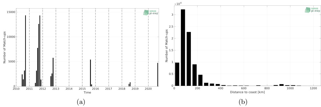
Figure 1: Number of match-ups between TSG (SAMOS) and SMOS SSS L3 v332 - 9 Days (CATDS-CPDC) SSS as a function of time (a) and as function of the distance to coast (b) over the Arctic Ocean Pi-MEP region and for the full satellite product period.
