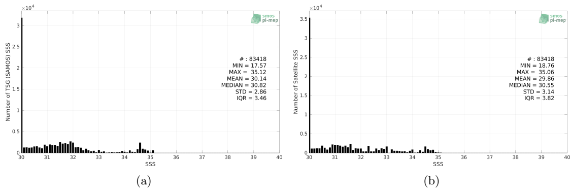
Figure 2: Histograms of SSS from TSG (SAMOS) (a) and SMOS SSS L3 v332 - 9 Days (CATDS-CPDC) (b) considering all match-up pairs per bins of 0.1 over the Arctic Ocean Pi-MEP region and for the full satellite product period.
