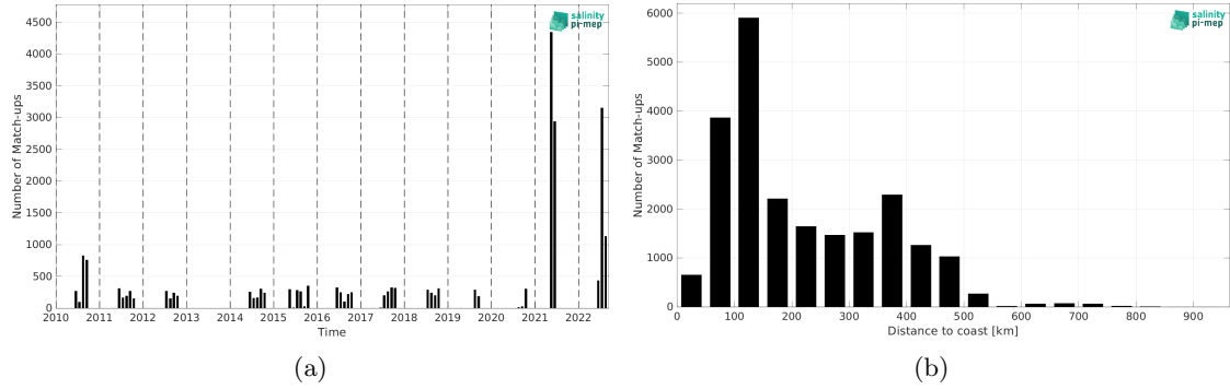
Figure 2: Number of match-ups between TSG (Polarstern) and SMOS SSS L3 v332 - 9 Days (CATDS-CPDC) SSS as a function of time (a) and as function of the distance to coast (b) over the Arctic Ocean Pi-MEP region and for the full satellite product period.
