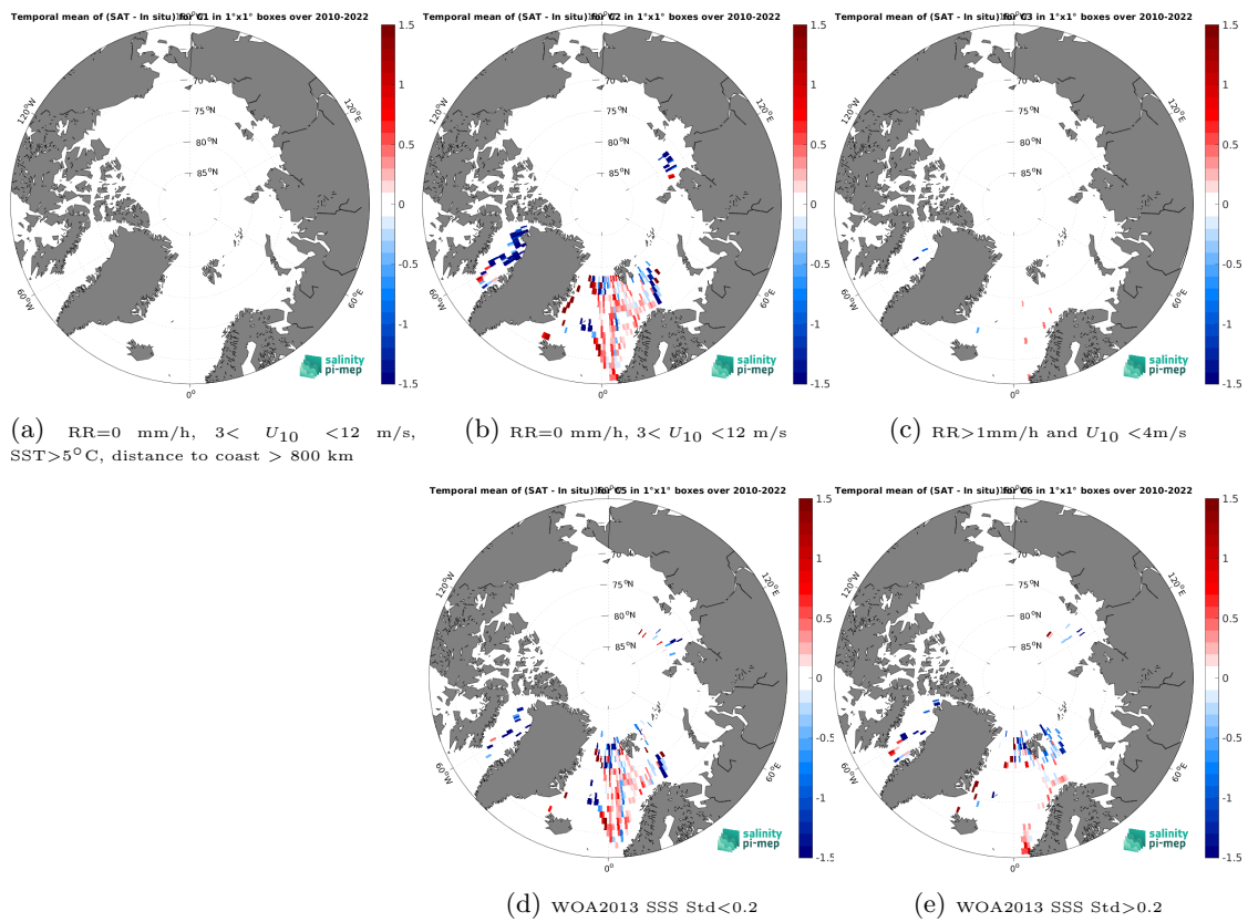
Figure 14: Temporal mean gridded over spatial boxes of size 1^\circ \times 1^\circ of \Delta SSS (SMOS SSS L3 v332 - 9 Days (CATDS-CPDC) - TSG (Polarstern)) for 5 different subdatasets corresponding to: RR=0 mm/h, 3 < U_{10} < 12 m/s, SST > 5°C, distance to coast > 800 km (a), RR=0 mm/h, 3 < U_{10} < 12 m/s (b), RR > 1mm/h and U_{10} < 4 m/s (c), WOA2013 SSS Std < 0.2 (d), WOA2013 SSS Std > 0.2 (e).
