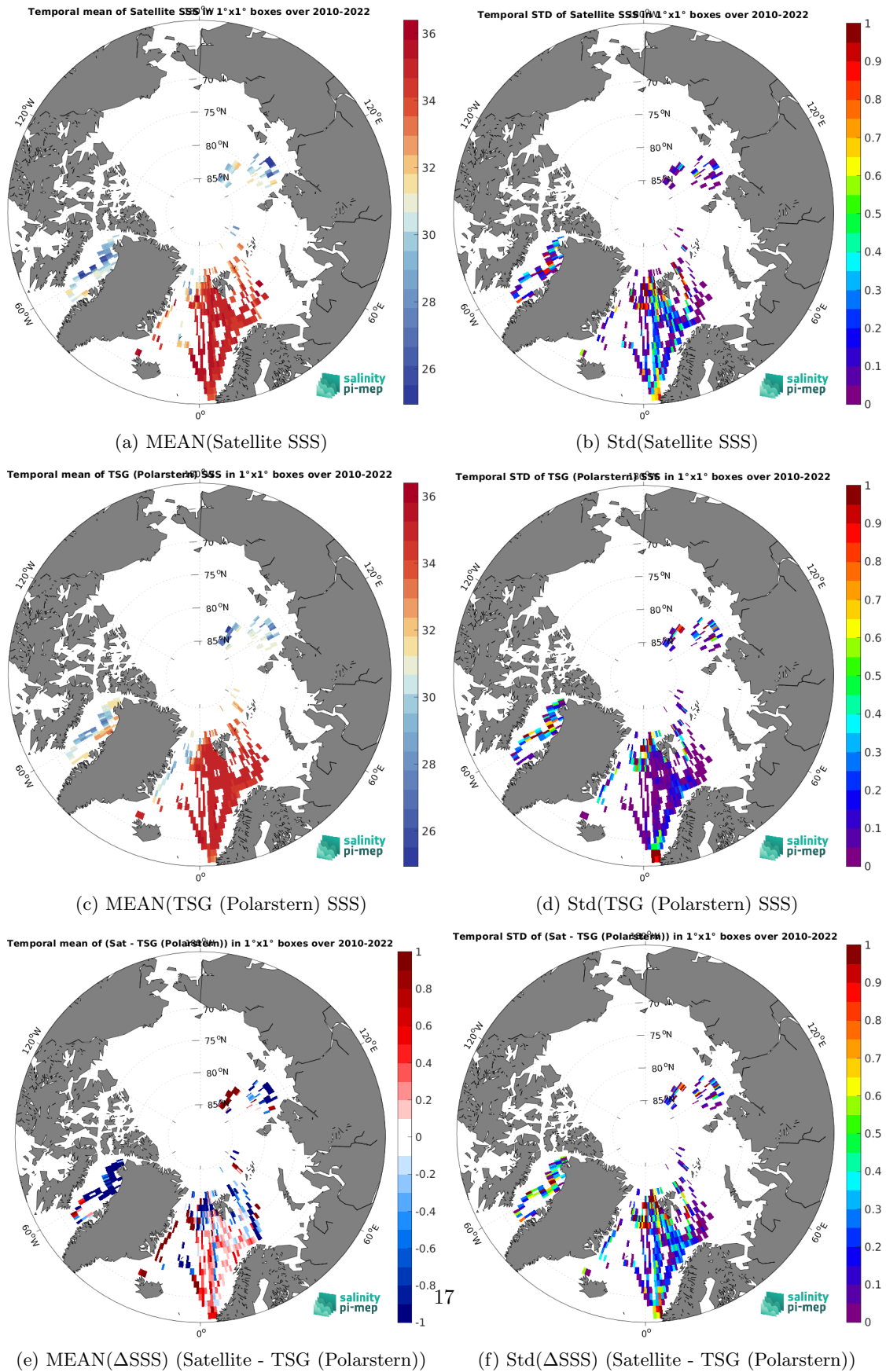
Figure 7: Temporal mean (left) and Std (right) of SSS from SMOS SSS L3 v332 - 9 Days (CATDS-CPDC) (top), TSG (Polarstern) (middle), and of \Delta SSS (Satellite - TSG (Polarstern)). Only match-up pairs are used to generate these maps.
