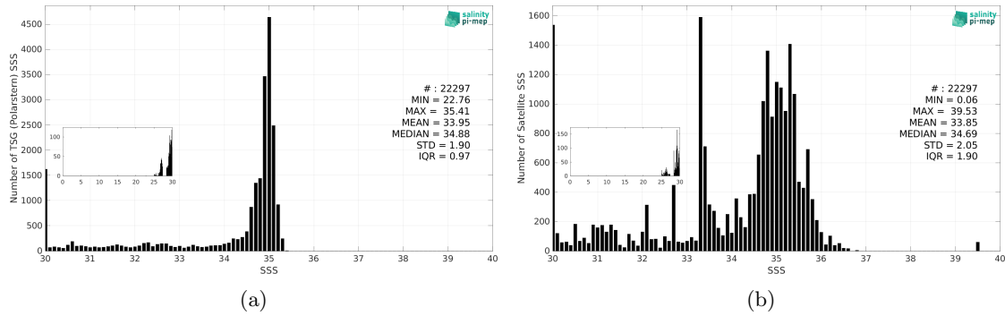
Figure 3: Histograms of SSS from TSG (Polarstern) (a) and SMOS SSS L3 v332 - 9 Days (CATDS-CPDC) (b) considering all match-up pairs per bins of 0.1 over the Arctic Ocean Pi-MEP region and for the full satellite product period.
