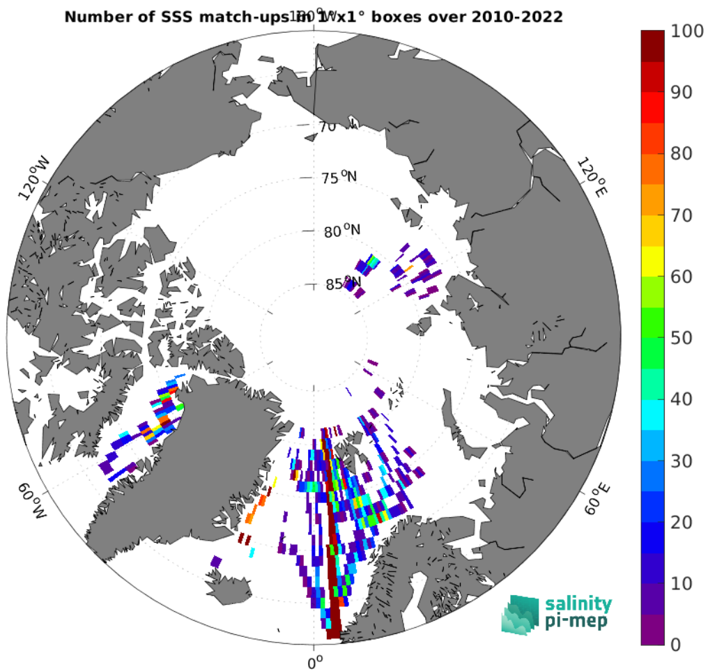
Figure 5: Number of SSS match-ups between TSG (Polarstern) SSS and the SMOS SSS L3 v332 - 9 Days (CATDS-CPDC) SSS product for the Arctic Ocean Pi-MEP region over 1^\circ \times 1^\circ boxes and for the full satellite product period.
