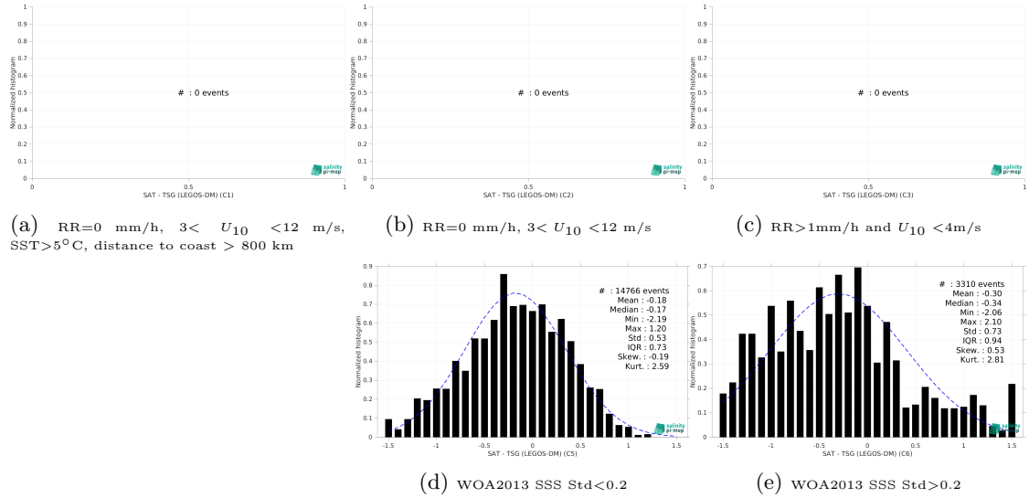
Figure 13: Normalized histogram of \Delta SSS (SMOS SSS L3 v332 - 9 Days (CATDS-CPDC) - TSG (LEGOS-DM)) for 5 different subdatasets corresponding to: RR=0 mm/h, 3 < U_{10} < 12 m/s, SST > 5°C, distance to coast > 800 km (a), RR=0 mm/h, 3 < U_{10} < 12 m/s (b), RR > 1mm/h and U_{10} < 4 m/s (c), WOA2013 SSS Std < 0.2 (d), WOA2013 SSS Std > 0.2 (e).
