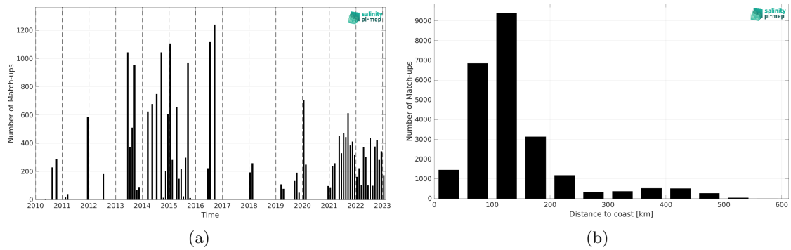
Figure 1: Number of match-ups between TSG (LEGOS-DM) and SMOS SSS L3 v332 - 9 Days (CATDS-CPDC) SSS as a function of time (a) and as function of the distance to coast (b) over the Arctic Ocean Pi-MEP region and for the full satellite product period.
