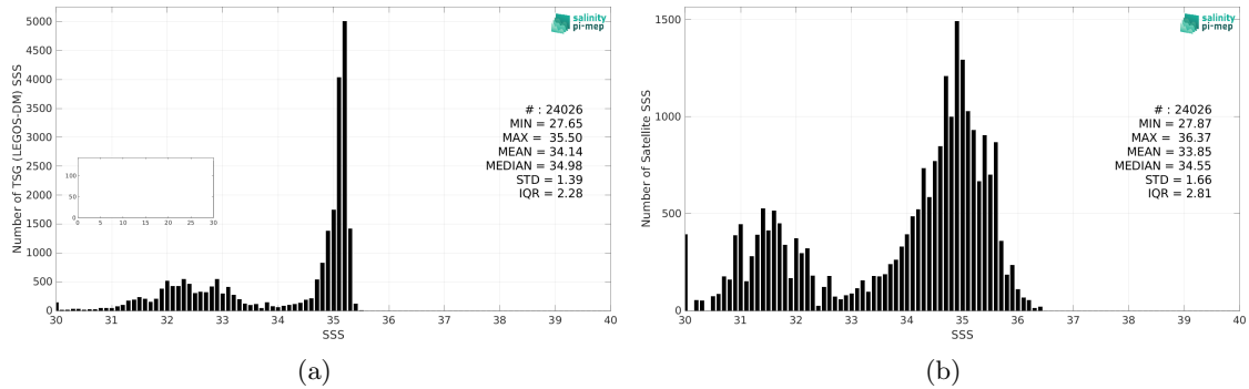
Figure 2: Histograms of SSS from TSG (LEGOS-DM) (a) and SMOS SSS L3 v332 - 9 Days (CATDS-CPDC) (b) considering all match-up pairs per bins of 0.1 over the Arctic Ocean Pi-MEP region and for the full satellite product period.
