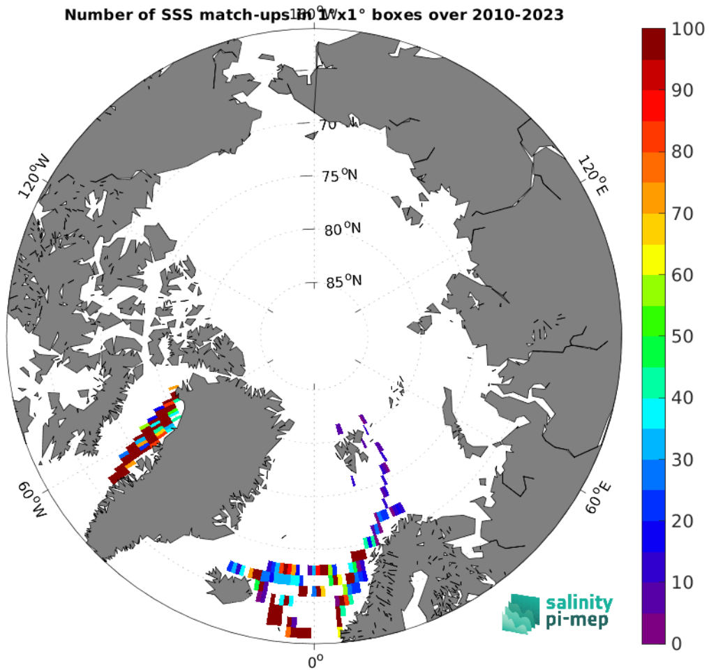
Figure 4: Number of SSS match-ups between TSG (LEGOS-DM) SSS and the SMOS SSS L3 v332 - 9 Days (CATDS-CPDC) SSS product for the Arctic Ocean Pi-MEP region over 1^\circ \times 1^\circ boxes and for the full satellite product period.
