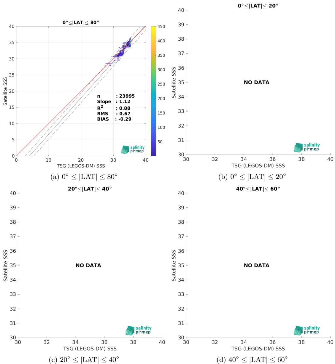
Figure 9: Contour maps of the concentration of SMOS SSS L3 v332 - 9 Days (CATDS-CPDC) SSS (y-axis) versus TSG (LEGOS-DM) SSS (x-axis) at match-up pairs for different latitude bands. For each plot, the red line shows x=y . The black thin and dashed lines indicate a linear fit through the data cloud and the \pm 95\% confidence levels, respectively. The number match-up pairs n , the slope and R^2 coefficient of the linear fit, the root mean square (RMS) and the mean bias between satellite and in situ data are indicated for each latitude band in each plots.
