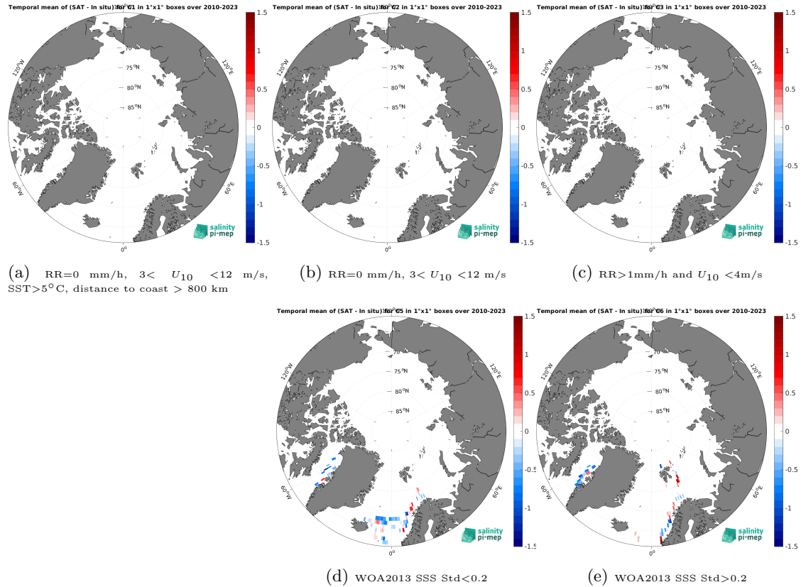
Figure 12: Temporal mean gridded over spatial boxes of size 1^{\circ}\times 1^{\circ} of \Delta\text{SSS} (SMOS SSS L3 v332 - 9 Days (CATDS-CPDC) - TSG (LEGOS-DM)) for 5 different subdatasets corresponding to: RR=0 mm/h, 3 < U_{10} < 12 m/s, SST > 5^{\circ}\text{C} , distance to coast > 800 km (a), RR=0 mm/h, 3 < U_{10} < 12 m/s (b), RR > 1 mm/h and U_{10} < 4 m/s (c), WOA2013 SSS Std < 0.2 (d), WOA2013 SSS Std > 0.2 (e).
