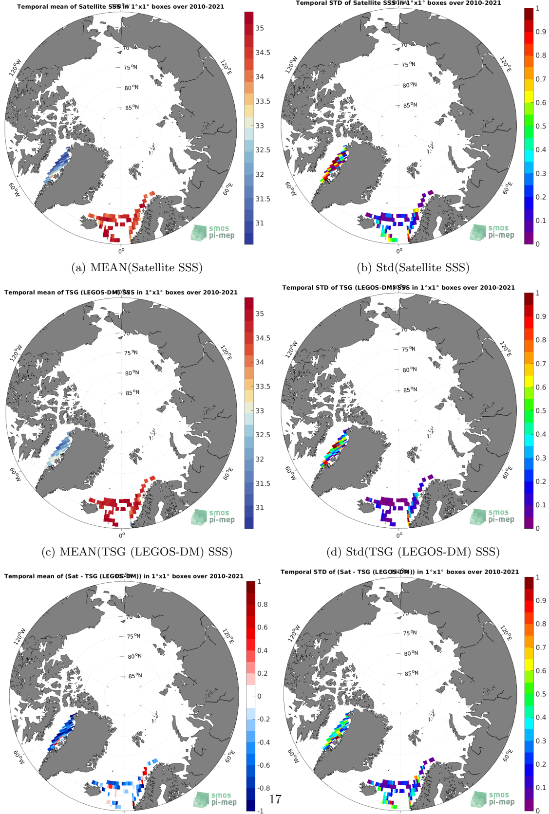
(e) MEAN( \Delta SSS) (Satellite - TSG (LEGOS-DM)) (f) Std( \Delta SSS) (Satellite - TSG (LEGOS-DM)) Figure 6: Temporal mean (left) and Std (right) of SSS from SMOS SSS L3 v332 - 9 Days (CATDS-CPDC) (top), TSG (LEGOS-DM) (middle), and of \Delta SSS (Satellite - TSG (LEGOS-DM)). Only match-up pairs are used to generate these maps.
