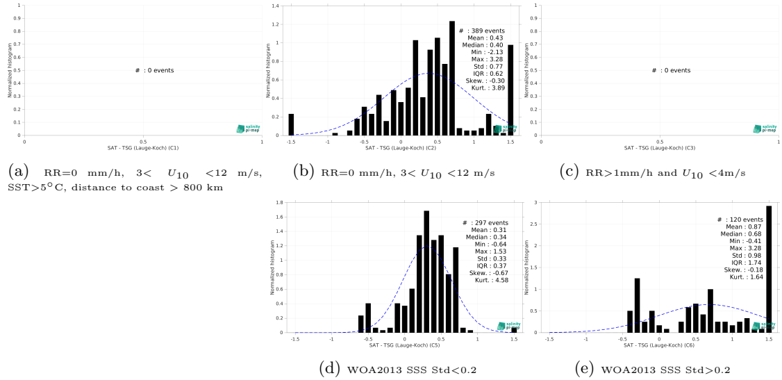
Figure 15: Normalized histogram of \Delta\text{SSS} (SMOS SSS L3 v332 - 9 Days (CATDS-CPDC) - TSG (Lauge-Koch)) for 5 different subdatasets corresponding to: RR=0 mm/h, 3 < U_{10} < 12 m/s, SST >5^{\circ}\text{C} , distance to coast > 800 km (a), RR=0 mm/h, 3 < U_{10} < 12 m/s (b), RR >1 mm/h and U_{10} < 4 m/s (c), WOA2013 SSS Std <0.2 (d), WOA2013 SSS Std >0.2 (e).
