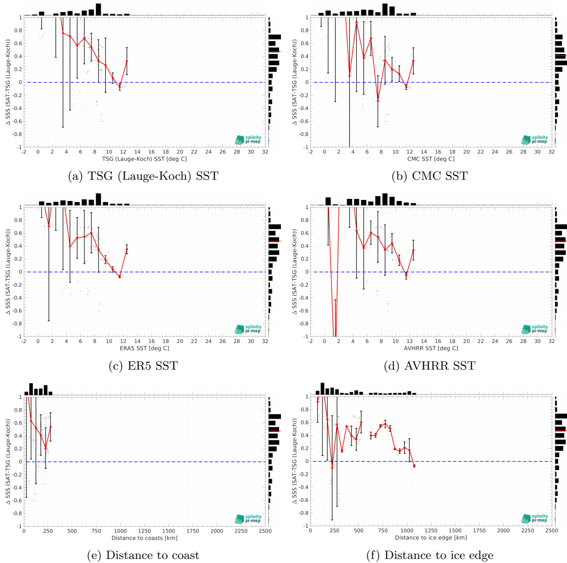
Figure 13: \Delta \text{SSS} (Satellite - TSG (Lauge-Koch)) sorted as function of TSG (Lauge-Koch) SST values (a), CMC SST (b), ERA5 SST (c), AVHRR SST (d), distance to coast (e) and distance to ice edge (f). In all plots the median and Std of \Delta \text{SSS} for each bin is indicated by the red curves and black vertical thick bars ( \pm 1 Std). Links to similar figures sorted as function of Sea ice fraction and in situ measurement depth .
