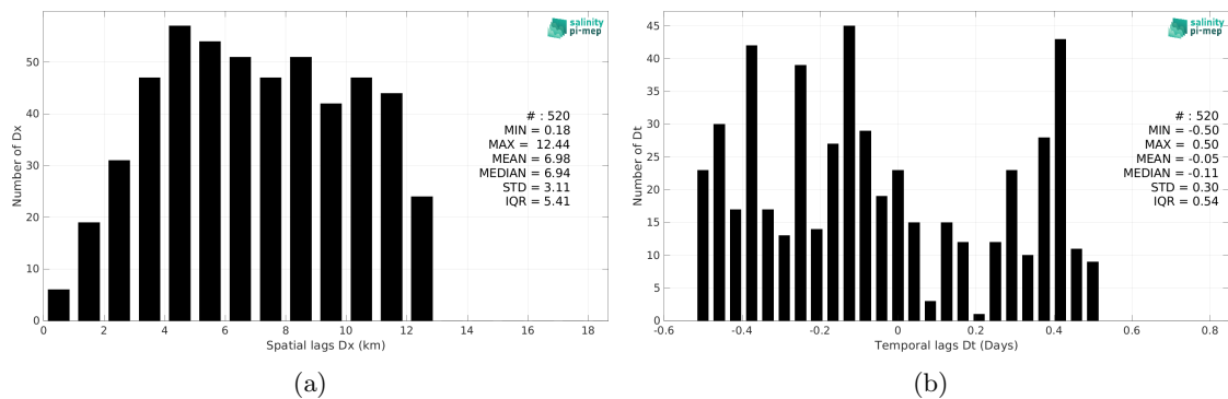
Figure 6: Histograms of the spatial (a) and temporal (b) lags between the location/time of the TSG (Lauge-Koch) measurement and the date of the corresponding SMOS SSS L3 v332 - 9 Days (CATDS-CPDC) SSS pixel.
