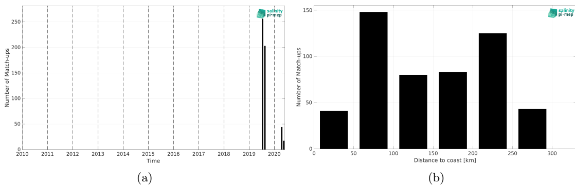
Figure 1: Number of match-ups between TSG (Lauge-Koch) and SMOS SSS L3 v332 - 9 Days (CATDS-CPDC) SSS as a function of time (a) and as function of the distance to coast (b) over the Arctic Ocean Pi-MEP region and for the full satellite product period.
