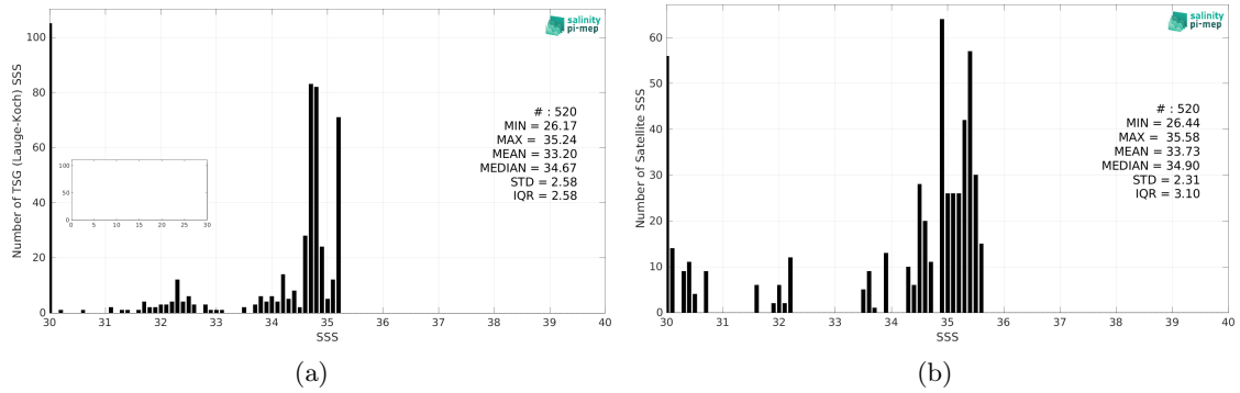
Figure 2: Histograms of SSS from TSG (Lauge-Koch) (a) and SMOS SSS L3 v332 - 9 Days (CATDS-CPDC) (b) considering all match-up pairs per bins of 0.1 over the Arctic Ocean Pi-MEP region and for the full satellite product period.
