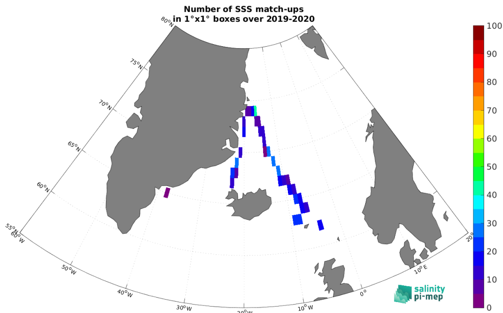
Figure 4: Number of SSS match-ups between TSG (Lauge-Koch) SSS and the SMOS SSS L3 v332 - 9 Days (CATDS-CPDC) SSS product for the Arctic Ocean Pi-MEP region over 1^\circ \times 1^\circ boxes and for the full satellite product period.
