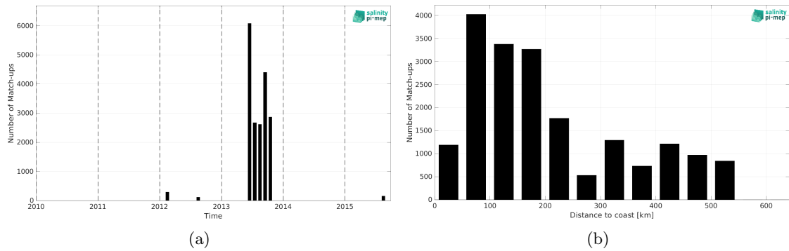
Figure 2: Number of match-ups between TSG (GOSUD-Sailing-ship) and SMOS SSS L3 v332 - 9 Days (CATDS-CPDC) SSS as a function of time (a) and as function of the distance to coast (b) over the Arctic Ocean Pi-MEP region and for the full satellite product period.
