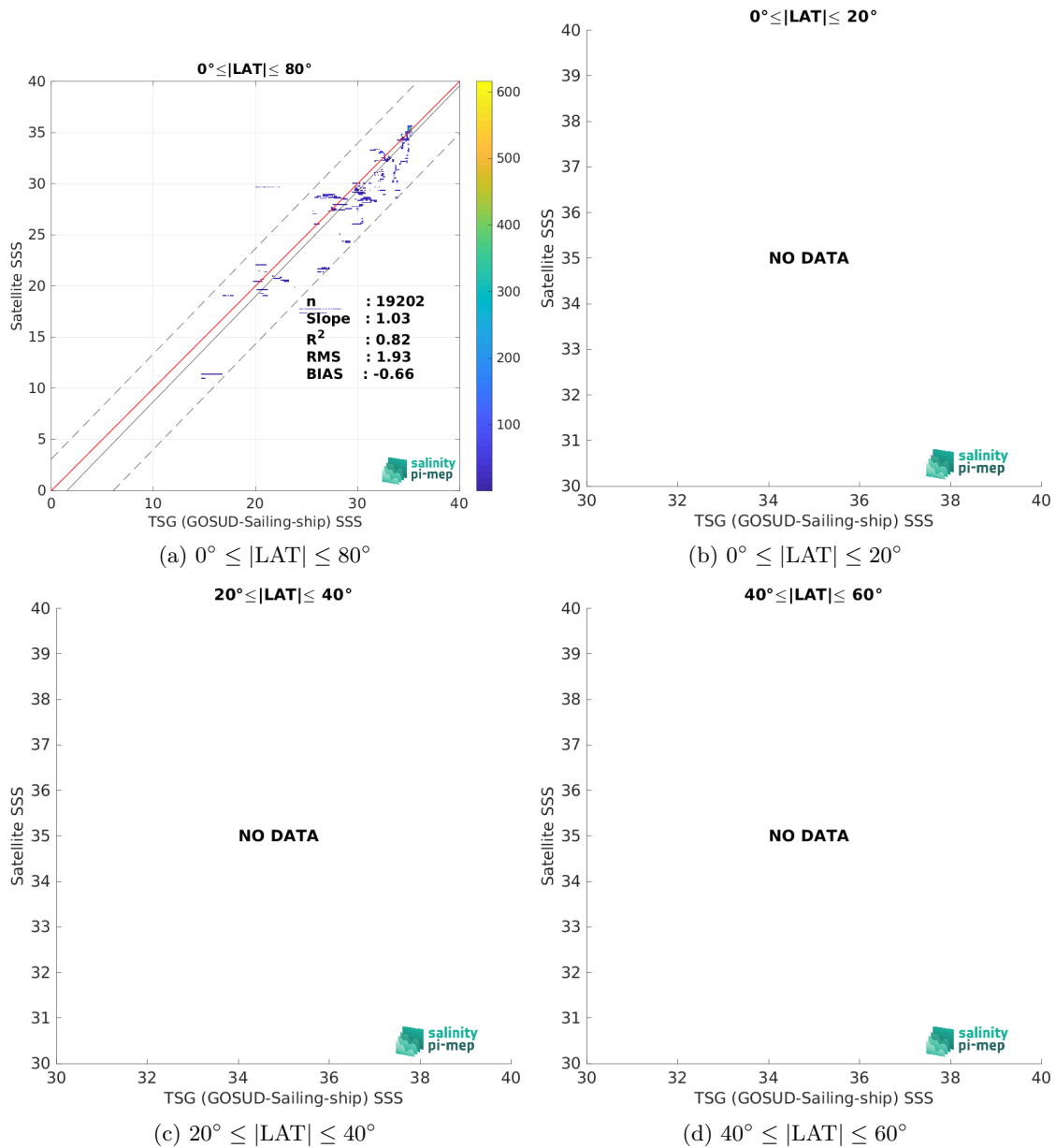
Figure 10: Contour maps of the concentration of SMOS SSS L3 v332 - 9 Days (CATDS-CPDC) SSS (y-axis) versus TSG (GOSUD-Sailing-ship) SSS (x-axis) at match-up pairs for different latitude bands. For each plot, the red line shows x=y . The black thin and dashed lines indicate a linear fit through the data cloud and the \pm 95\% confidence levels, respectively. The number match-up pairs n , the slope and R^2 coefficient of the linear fit, the root mean square (RMS) and the mean bias between satellite and in situ data are indicated for each latitude band in each plots.
