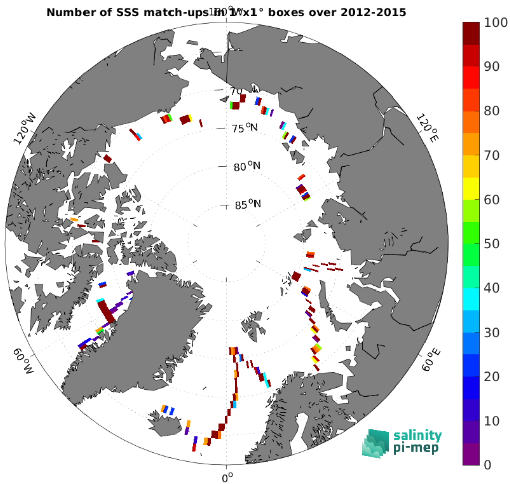
Figure 5: Number of SSS match-ups between TSG (GOSUD-Sailing-ship) SSS and the SMOS SSS L3 v332 - 9 Days (CATDS-CPDC) SSS product for the Arctic Ocean Pi-MEP region over 1^\circ \times 1^\circ boxes and for the full satellite product period.
