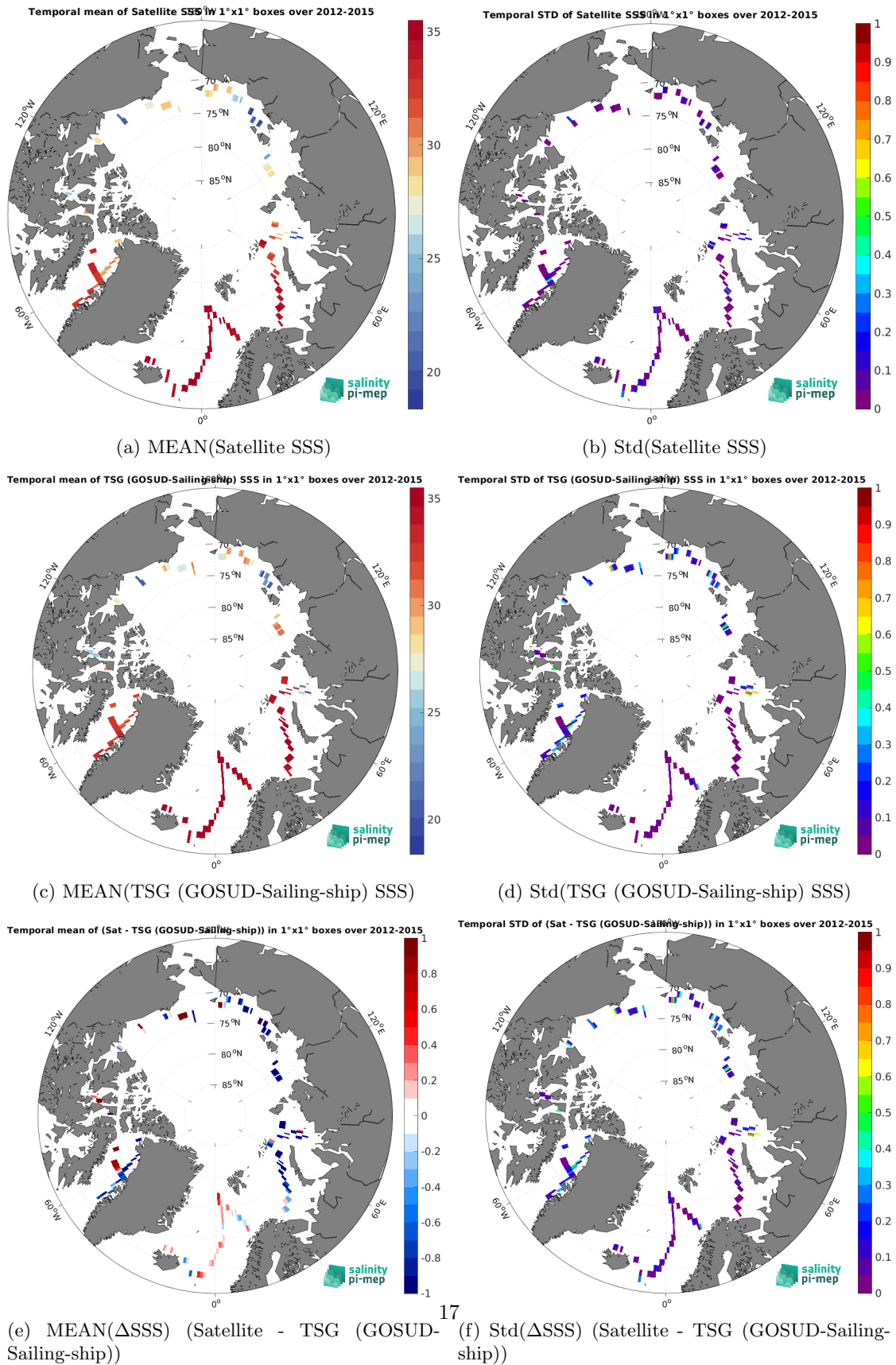
Figure 7: Temporal mean (left) and Std (right) of SSS from SMOS SSS L3 v332 - 9 Days (CATDS-CPDC) (top), TSG (GOSUD-Sailing-ship) (middle), and of \Delta SSS (Satellite - TSG (GOSUD-Sailing-ship)). Only match-up pairs are used to generate these maps.
