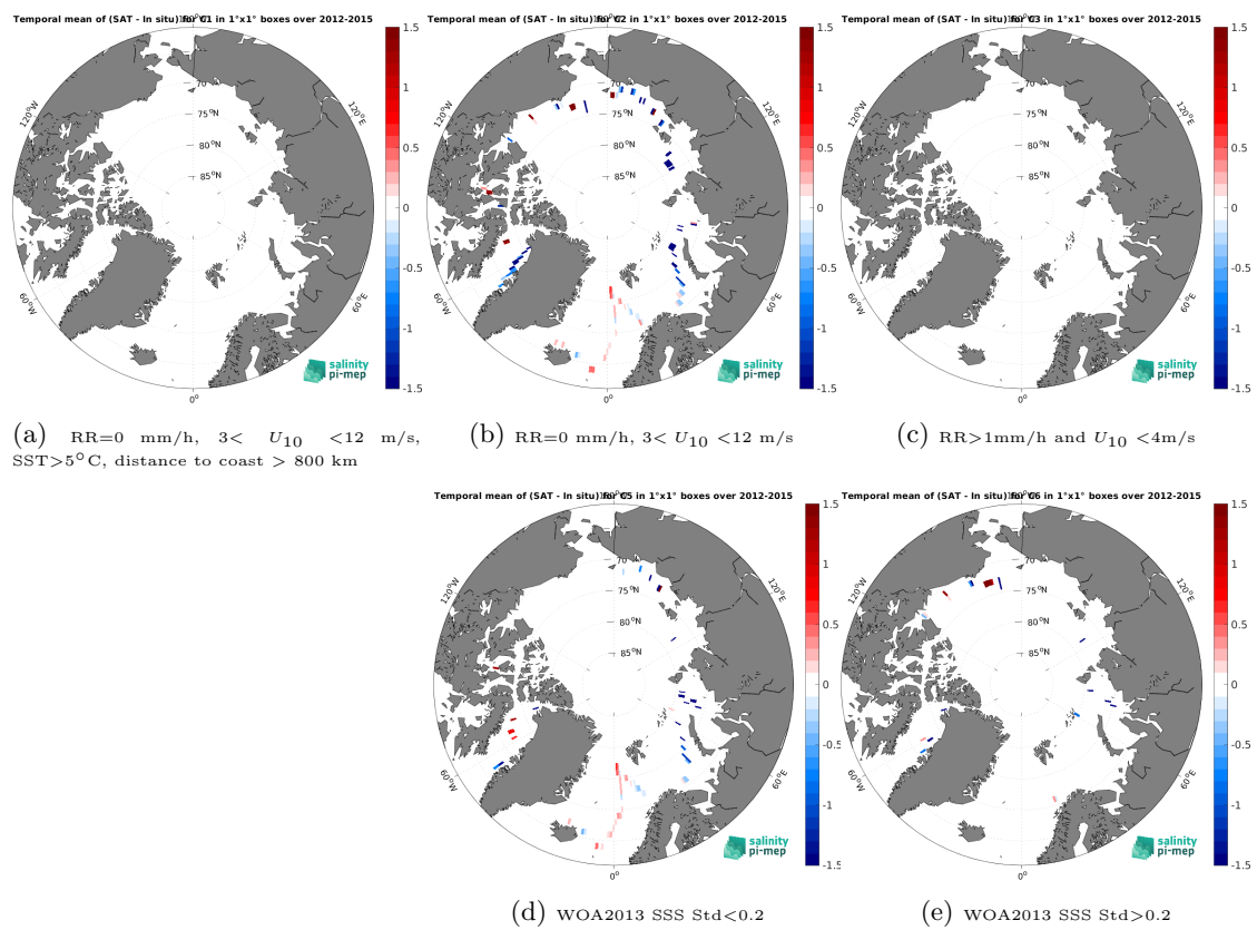
Figure 14: Temporal mean gridded over spatial boxes of size 1^\circ \times 1^\circ of \Delta SSS (SMOS SSS L3 v332 - 9 Days (CATDS-CPDC) - TSG (GOSUD-Sailing-ship)) for 5 different subdatasets corresponding to: RR=0 mm/h, 3 < U_{10} < 12 m/s, SST > 5°C, distance to coast > 800 km (a), RR=0 mm/h, 3 < U_{10} < 12 m/s (b), RR > 1mm/h and U_{10} < 4 m/s (c), WOA2013 SSS Std < 0.2 (d), WOA2013 SSS Std > 0.2 (e).
