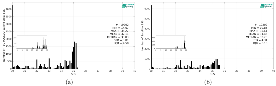
Figure 3: Histograms of SSS from TSG (GOSUD-Sailing-ship) (a) and SMOS SSS L3 v332 - 9 Days (CATDS-CPDC) (b) considering all match-up pairs per bins of 0.1 over the Arctic Ocean Pi-MEP region and for the full satellite product period.
