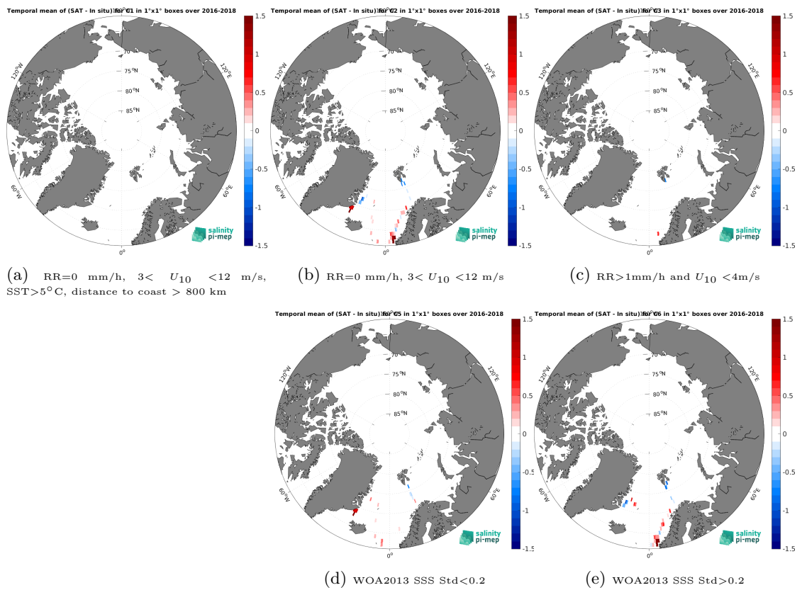
Figure 14: Temporal mean gridded over spatial boxes of size 1^\circ \times 1^\circ of \Delta SSS (SMOS SSS L3 v332 - 9 Days (CATDS-CPDC) - TSG (GOSUD-Research-vessel)) for 5 different subdatasets corresponding to:RR=0 mm/h, 3 < U_{10} < 12 m/s, SST>5°C, distance to coast > 800 km (a), RR=0 mm/h, 3 < U_{10} < 12 m/s (b), RR>1mm/h and U_{10} < 4 m/s (c), WOA2013 SSS Std<0.2 (d), WOA2013 SSS Std>0.2 (e).
