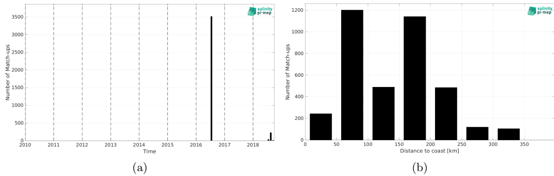
Figure 2: Number of match-ups between TSG (GOSUD-Research-vessel) and SMOS SSS L3 v332 - 9 Days (CATDS-CPDC) SSS as a function of time (a) and as function of the distance to coast (b) over the Arctic Ocean Pi-MEP region and for the full satellite product period.
