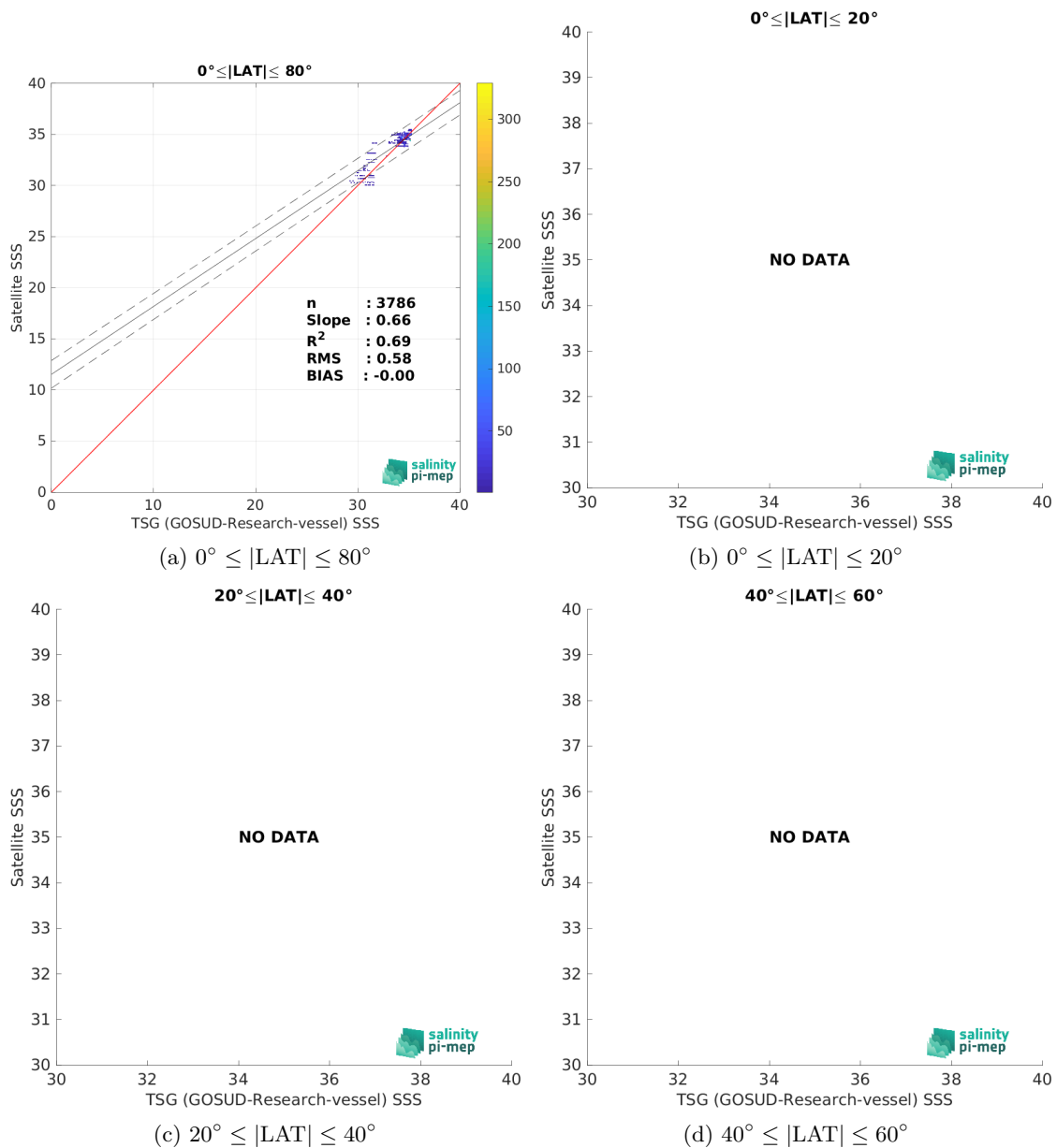
Figure 10: Contour maps of the concentration of SMOS SSS L3 v332 - 9 Days (CATDS-CPDC) SSS (y-axis) versus TSG (GOSUD-Research-vessel) SSS (x-axis) at match-up pairs for different latitude bands. For each plot, the red line shows x=y . The black thin and dashed lines indicate a linear fit through the data cloud and the \pm 95\% confidence levels, respectively. The number match-up pairs n , the slope and R^2 coefficient of the linear fit, the root mean square (RMS) and the mean bias between satellite and in situ data are indicated for each latitude band in each plots.
