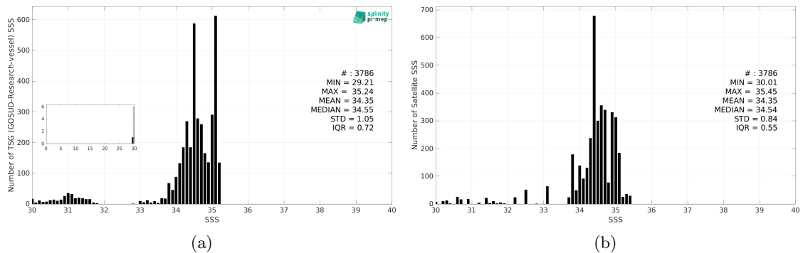
Figure 3: Histograms of SSS from TSG (GOSUD-Research-vessel) (a) and SMOS SSS L3 v332 - 9 Days (CATDS-CPDC) (b) considering all match-up pairs per bins of 0.1 over the Arctic Ocean Pi-MEP region and for the full satellite product period.
