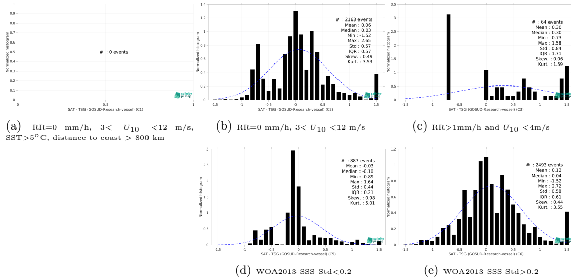
Figure 15: Normalized histogram of \Delta SSS (SMOS SSS L3 v332 - 9 Days (CATDS-CPDC) - TSG (GOSUD-Research-vessel)) for 5 different subdatasets corresponding to: RR=0 mm/h, 3 < U_{10} < 12 m/s, SST > 5°C, distance to coast > 800 km (a), RR=0 mm/h, 3 < U_{10} < 12 m/s (b), RR > 1mm/h and U_{10} < 4 m/s (c), WOA2013 SSS Std < 0.2 (d), WOA2013 SSS Std > 0.2 (e).
