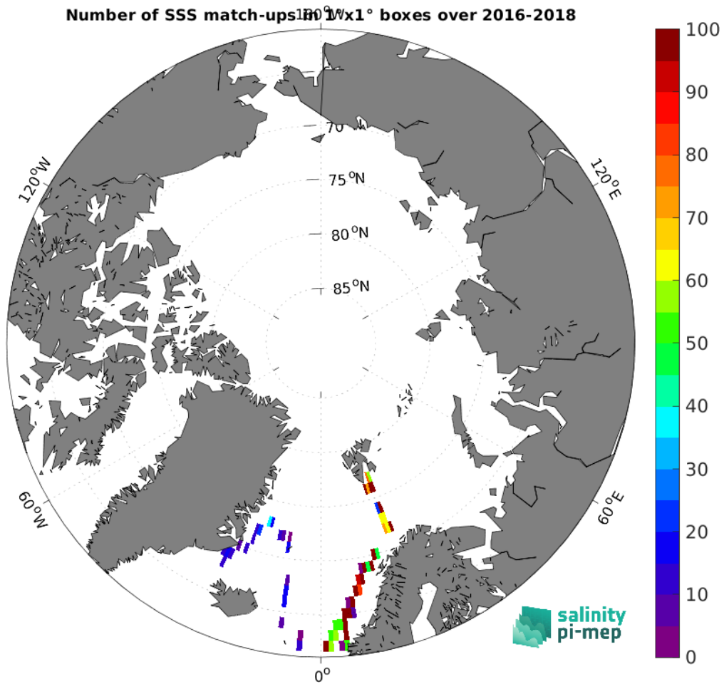
Figure 5: Number of SSS match-ups between TSG (GOSUD-Research-vessel) SSS and the SMOS SSS L3 v332 - 9 Days (CATDS-CPDC) SSS product for the Arctic Ocean Pi-MEP region over 1^\circ \times 1^\circ boxes and for the full satellite product period.
