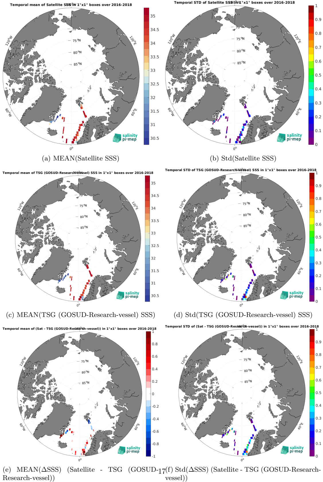
Figure 7: Temporal mean (left) and Std (right) of SSS from SMOS SSS L3 v332 - 9 Days (CATDS-CPDC) (top), TSG (GOSUD-Research-vessel) (middle), and of \Delta SSS (Satellite - TSG (GOSUD-Research-vessel)). Only match-up pairs are used to generate these maps.
