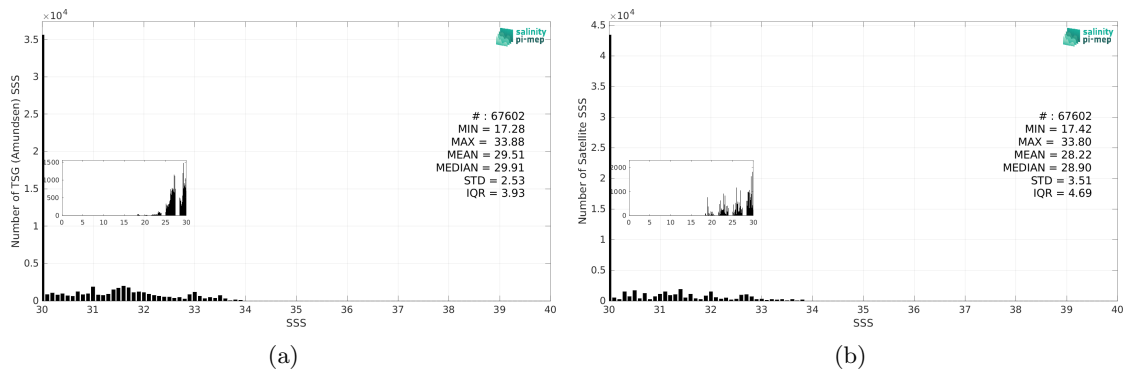
Figure 3: Histograms of SSS from TSG (Amundsen) (a) and SMOS SSS L3 v332 - 9 Days (CATDS-CPDC) (b) considering all match-up pairs per bins of 0.1 over the Arctic Ocean Pi-MEP region and for the full satellite product period.
