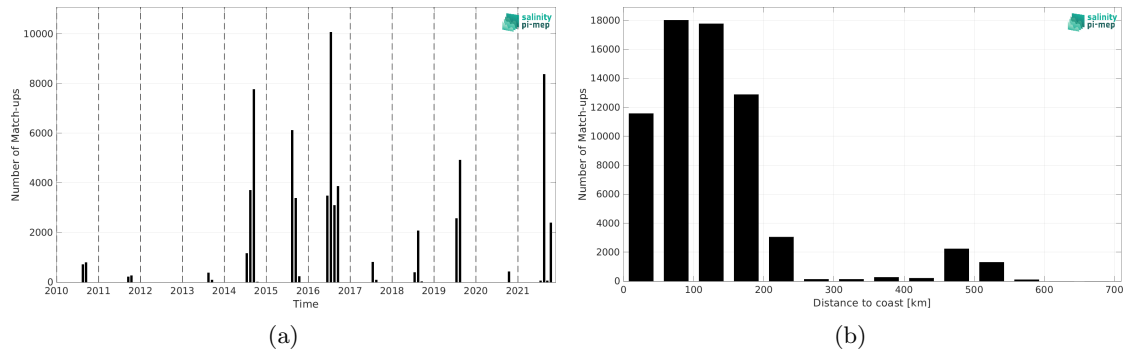
Figure 2: Number of match-ups between TSG (Amundsen) and SMOS SSS L3 v332 - 9 Days (CATDS-CPDC) SSS as a function of time (a) and as function of the distance to coast (b) over the Arctic Ocean Pi-MEP region and for the full satellite product period.
