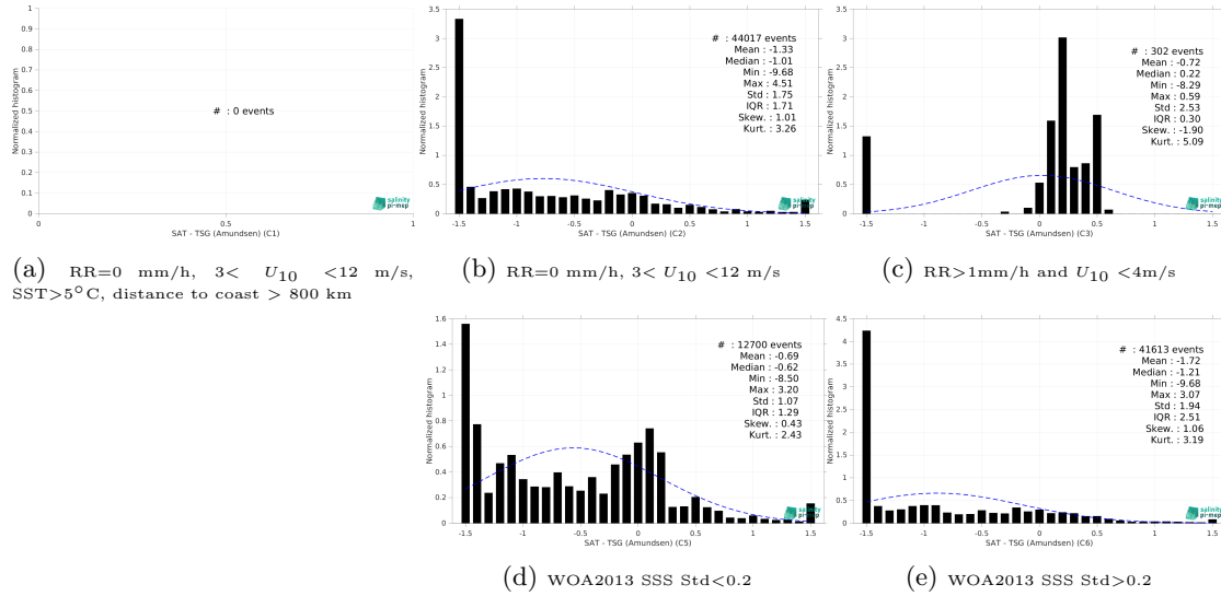
Figure 15: Normalized histogram of \Delta SSS (SMOS SSS L3 v332 - 9 Days (CATDS-CPDC) - TSG (Amundsen)) for 5 different subdatasets corresponding to: RR=0 mm/h, 3 < U_{10} < 12 m/s, SST>5°C, distance to coast > 800 km (a), RR=0 mm/h, 3 < U_{10} < 12 m/s (b), RR>1mm/h and U_{10} < 4 m/s (c), WOA2013 SSS Std<0.2 (d), WOA2013 SSS Std>0.2 (e).
