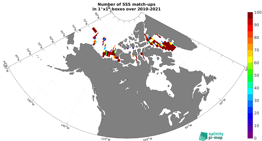
Figure 5: Number of SSS match-ups between TSG (Amundsen) SSS and the SMOS SSS L3 v332 - 9 Days (CATDS-CPDC) SSS product for the Arctic Ocean Pi-MEP region over 1^\circ \times 1^\circ boxes and for the full satellite product period.
