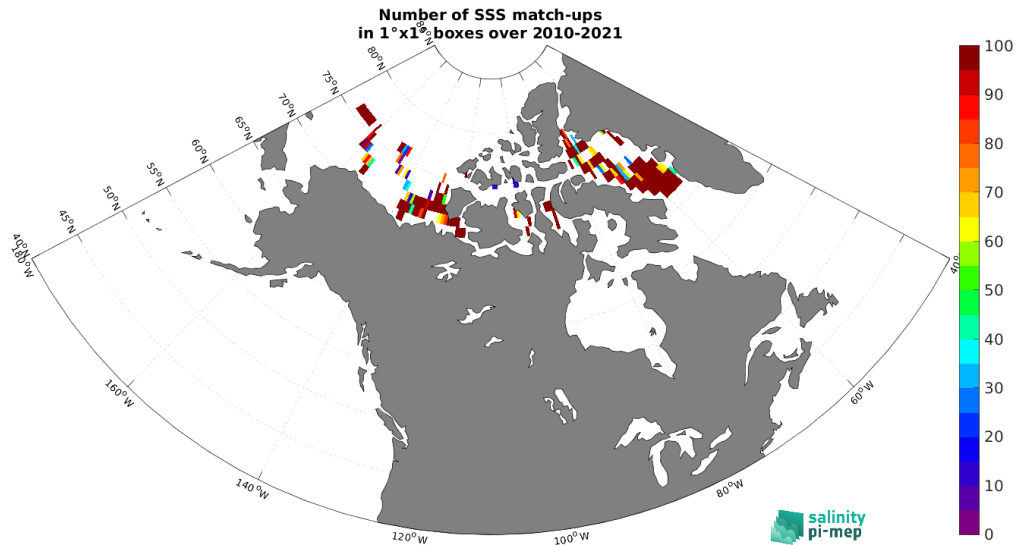
Figure 4: Number of SSS match-ups between TSG (Amundsen) SSS and the SMOS SSS L3 v332 - 9 Days (CATDS-CPDC) SSS product for the Arctic Ocean Pi-MEP region over 1^\circ \times 1^\circ boxes and for the full satellite product period.
