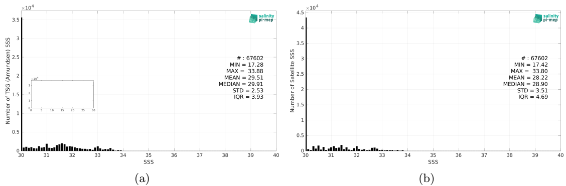
Figure 2: Histograms of SSS from TSG (Amundsen) (a) and SMOS SSS L3 v332 - 9 Days (CATDS-CPDC) (b) considering all match-up pairs per bins of 0.1 over the Arctic Ocean Pi-MEP region and for the full satellite product period.
