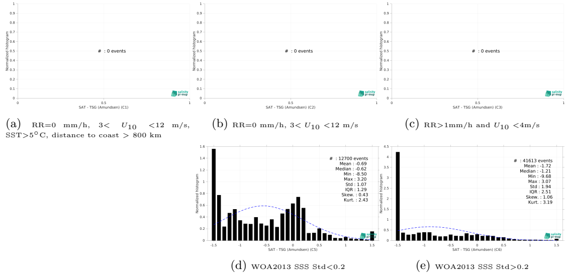
Figure 13: Normalized histogram of \Delta SSS (SMOS SSS L3 v332 - 9 Days (CATDS-CPDC) - TSG (Amundsen)) for 5 different subdatasets corresponding to: RR=0 mm/h, 3 < U_{10} < 12 m/s, SST>5°C, distance to coast > 800 km (a), RR=0 mm/h, 3 < U_{10} < 12 m/s (b), RR>1mm/h and U_{10} < 4 m/s (c), WOA2013 SSS Std<0.2 (d), WOA2013 SSS Std>0.2 (e).
