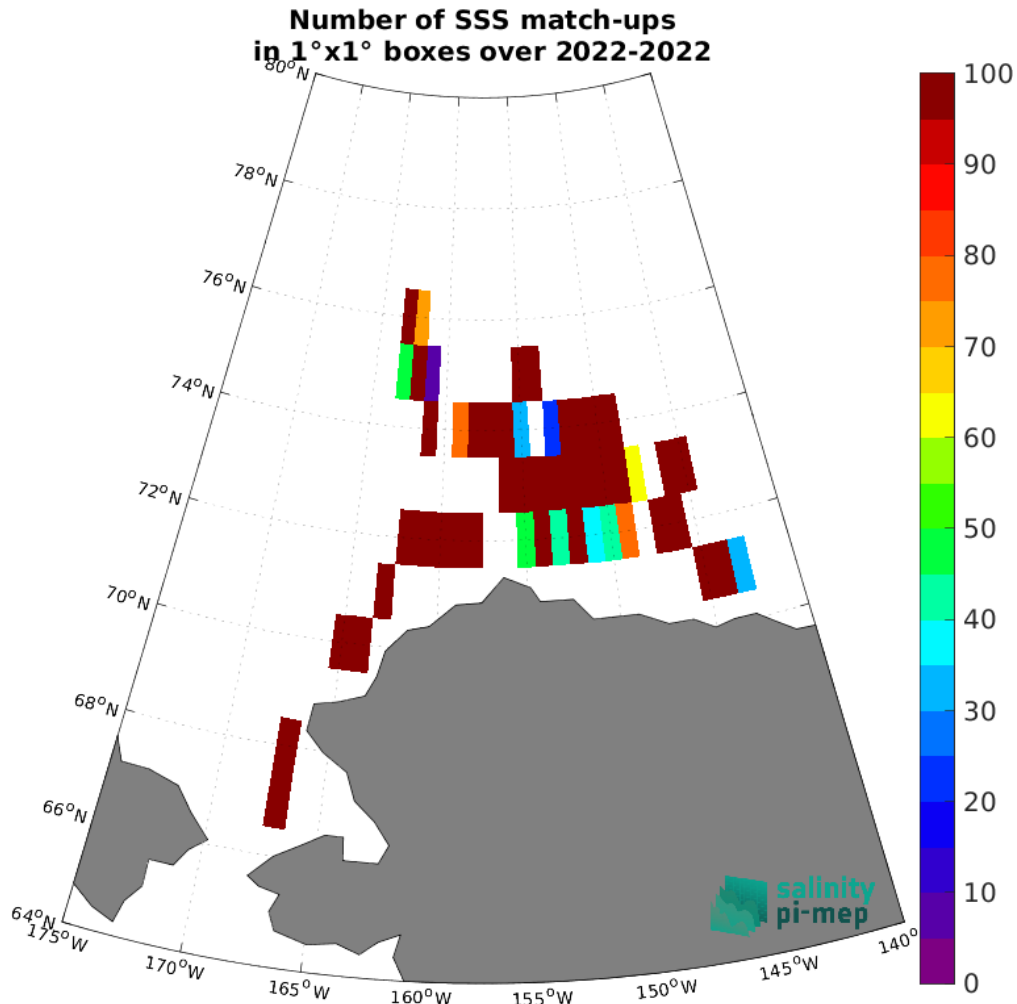
Figure 5: Number of SSS match-ups between SASSIE SSS and the SMOS SSS L3 v332 - 9 Days (CATDS-CPDC) SSS product for the Arctic Ocean Pi-MEP region over 1^\circ \times 1^\circ boxes and for the full satellite product period.
