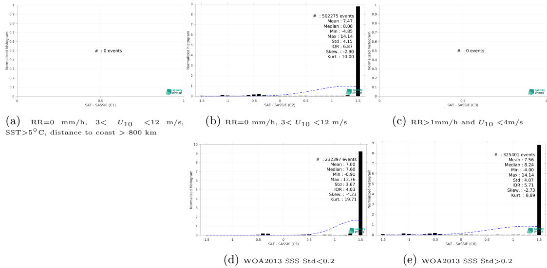
Figure 15: Normalized histogram of \Delta SSS (SMOS SSS L3 v332 - 9 Days (CATDS-CPDC) - SASSIE) for 5 different subdatasets corresponding to: RR=0 mm/h, 3 < U_{10} < 12 m/s, SST > 5°C, distance to coast > 800 km (a), RR=0 mm/h, 3 < U_{10} < 12 m/s (b), RR > 1mm/h and U_{10} < 4 m/s (c), WOA2013 SSS Std < 0.2 (d), WOA2013 SSS Std > 0.2 (e).
