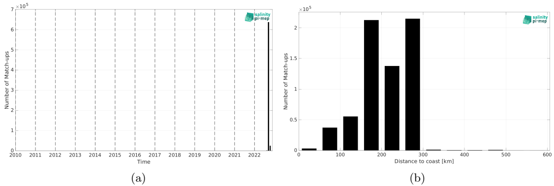
Figure 2: Number of match-ups between SASSIE and SMOS SSS L3 v332 - 9 Days (CATDS-CPDC) SSS as a function of time (a) and as function of the distance to coast (b) over the Arctic Ocean Pi-MEP region and for the full satellite product period.
