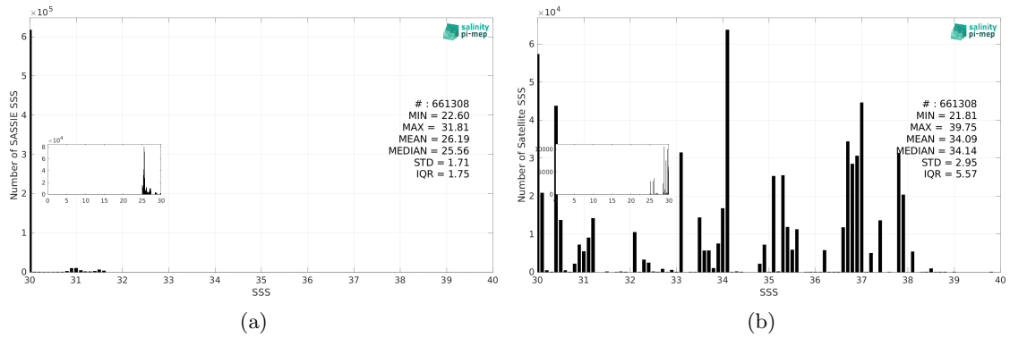
Figure 3: Histograms of SSS from SASSIE (a) and SMOS SSS L3 v332 - 9 Days (CATDS-CPDC) (b) considering all match-up pairs per bins of 0.1 over the Arctic Ocean Pi-MEP region and for the full satellite product period.
