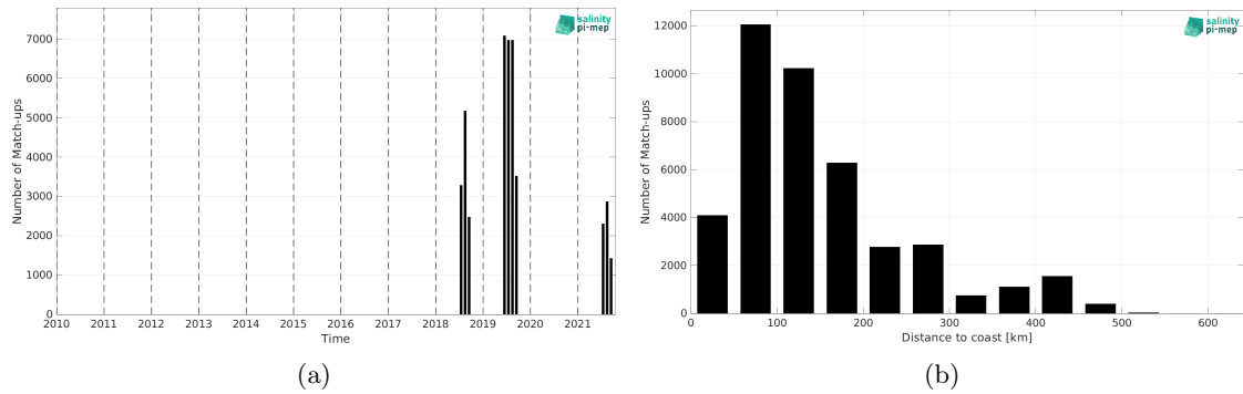
Figure 2: Number of match-ups between Saildrone and SMOS SSS L3 v332 - 9 Days (CATDS-CPDC) SSS as a function of time (a) and as function of the distance to coast (b) over the Arctic Ocean Pi-MEP region and for the full satellite product period.
