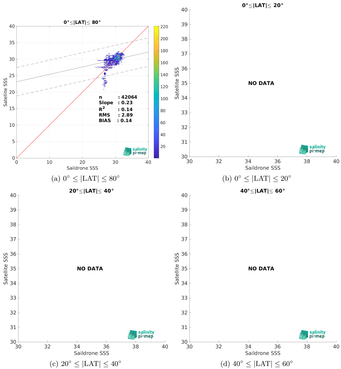
Figure 10: Contour maps of the concentration of SMOS SSS L3 v332 - 9 Days (CATDS-CPDC) SSS (y-axis) versus Saildrone SSS (x-axis) at match-up pairs for different latitude bands. For each plot, the red line shows x=y . The black thin and dashed lines indicate a linear fit through the data cloud and the \pm 95\% confidence levels, respectively. The number match-up pairs n , the slope and R^2 coefficient of the linear fit, the root mean square (RMS) and the mean bias between satellite and in situ data are indicated for each latitude band in each plots.
