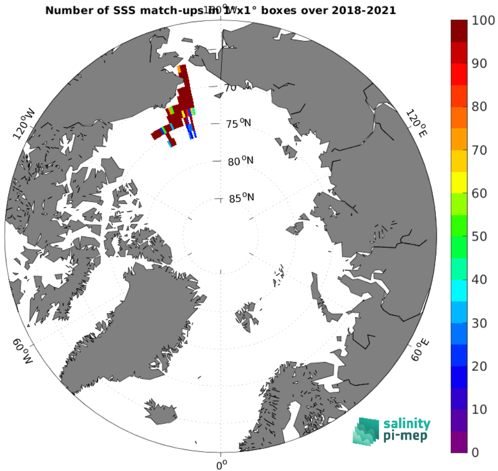
Figure 5: Number of SSS match-ups between Saildrone SSS and the SMOS SSS L3 v332 - 9 Days (CATDS-CPDC) SSS product for the Arctic Ocean Pi-MEP region over 1^\circ \times 1^\circ boxes and for the full satellite product period.
