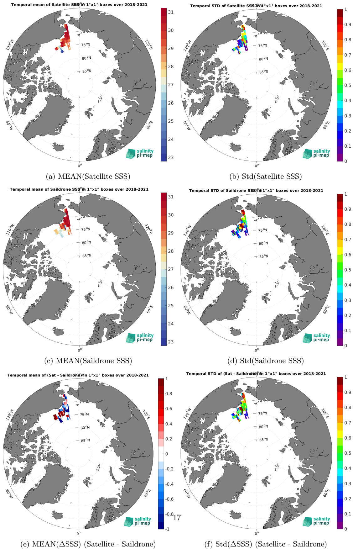
Figure 7: Temporal mean (left) and Std (right) of SSS from SMOS SSS L3 v332 - 9 Days (CATDS-CPDC) (top), Saildrone (middle), and of \Delta SSS (Satellite - Saildrone). Only match-up pairs are used to generate these maps.
