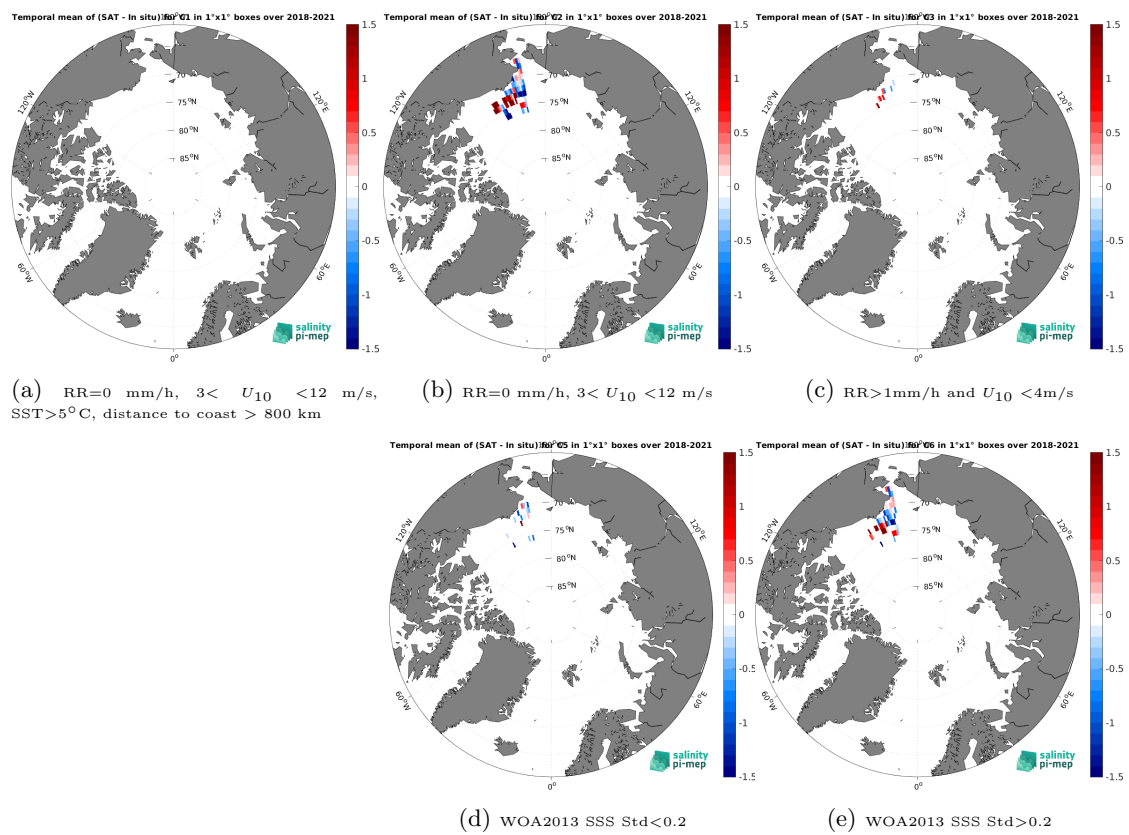
Figure 14: Temporal mean gridded over spatial boxes of size 1^\circ \times 1^\circ of \Delta\text{SSS} (SMOS SSS L3 v332 - 9 Days (CATDS-CPDC) - Saildrone) for 5 different subdatasets corresponding to:RR=0 mm/h, 3 < U_{10} < 12 m/s, SST > 5°C, distance to coast > 800 km (a), RR=0 mm/h, 3 < U_{10} < 12 m/s (b), RR > 1mm/h and U_{10} < 4 m/s (c), WOA2013 SSS Std < 0.2 (d), WOA2013 SSS Std > 0.2 (e).
