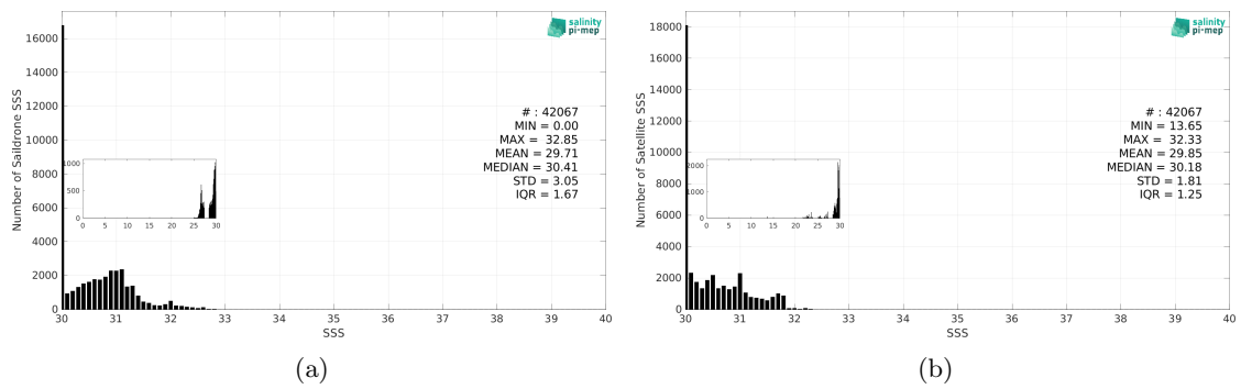
Figure 3: Histograms of SSS from Saildrone (a) and SMOS SSS L3 v332 - 9 Days (CATDS-CPDC) (b) considering all match-up pairs per bins of 0.1 over the Arctic Ocean Pi-MEP region and for the full satellite product period.
