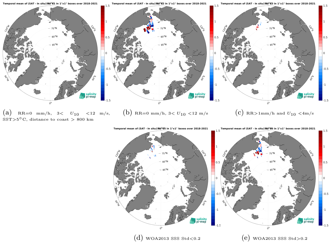
Figure 14: Temporal mean gridded over spatial boxes of size 1^\circ \times 1^\circ of \Delta SSS (SMOS SSS L3 v332 - 9 Days (CATDS-CPDC) - Saildrone) for 5 different subdatasets corresponding to:RR=0 mm/h, 3 < U_{10} < 12 m/s, SST>5°C, distance to coast > 800 km (a), RR=0 mm/h, 3 < U_{10} < 12 m/s (b), RR>1mm/h and U_{10} < 4 m/s (c), WOA2013 SSS Std<0.2 (d), WOA2013 SSS Std>0.2 (e).
