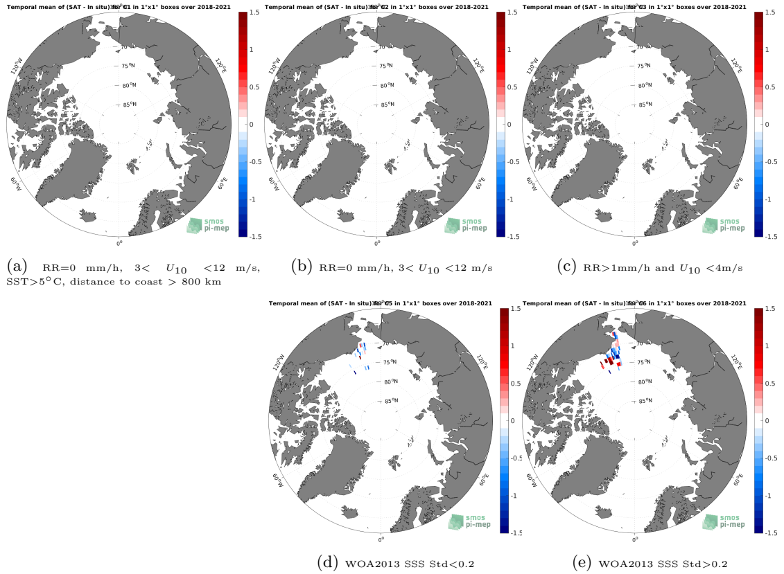
Figure 12: Temporal mean gridded over spatial boxes of size 1^{\circ}\times 1^{\circ} of \Delta\text{SSS} (SMOS SSS L3 v332 - 9 Days (CATDS-CPDC) - Sairdrone) for 5 different subdatasets corresponding to:RR=0 mm/h, 3 < U_{10} < 12 m/s, SST > 5^{\circ}\text{C} , distance to coast > 800 km (a), RR=0 mm/h, 3 < U_{10} < 12 m/s (b), RR > 1 mm/h and U_{10} < 4 m/s (c), WOA2013 SSS Std < 0.2 (d), WOA2013 SSS Std > 0.2 (e).
