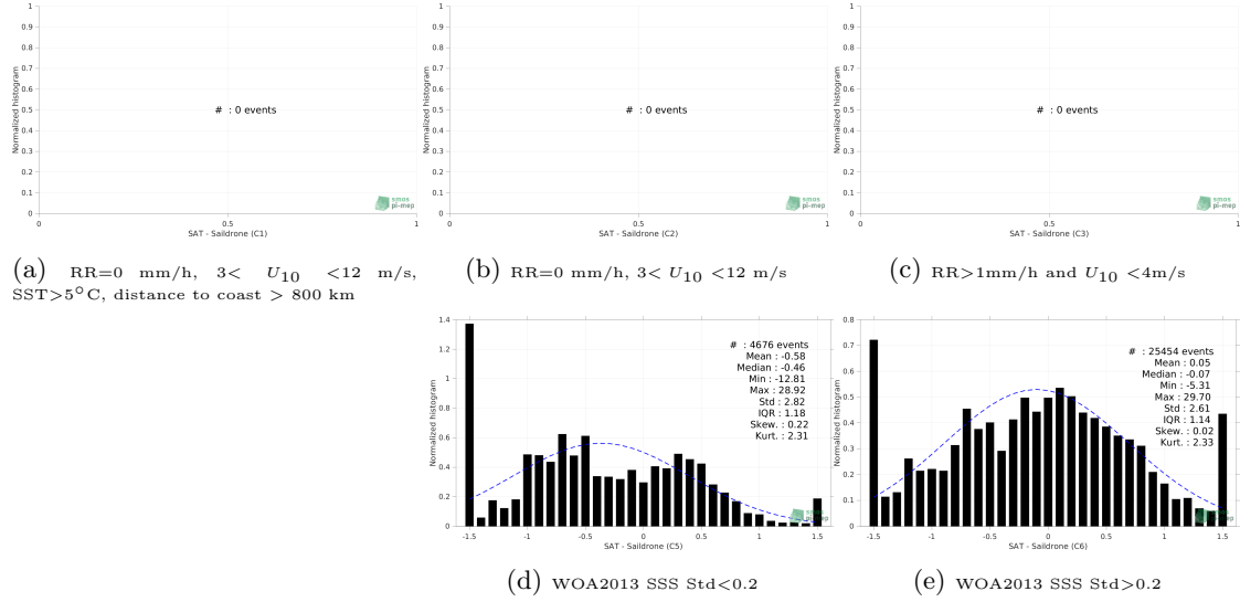
Figure 13: Normalized histogram of \Delta SSS (SMOS SSS L3 v332 - 9 Days (CATDS-CPDC) - Saldrone) for 5 different subdatasets corresponding to: RR=0 mm/h, 3 < U_{10} < 12 m/s, SST>5°C, distance to coast > 800 km (a), RR=0 mm/h, 3 < U_{10} < 12 m/s (b), RR>1mm/h and U_{10} < 4 m/s (c), WOA2013 SSS Std<0.2 (d), WOA2013 SSS Std>0.2 (e).
