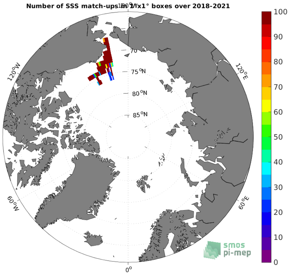
Figure 4: Number of SSS match-ups between Saifdrone SSS and the SMOS SSS L3 v332 - 9 Days (CATDS-CPDC) SSS product for the Arctic Ocean Pi-MEP region over 1^{\circ} \times 1^{\circ} boxes and for the full satellite product period.
