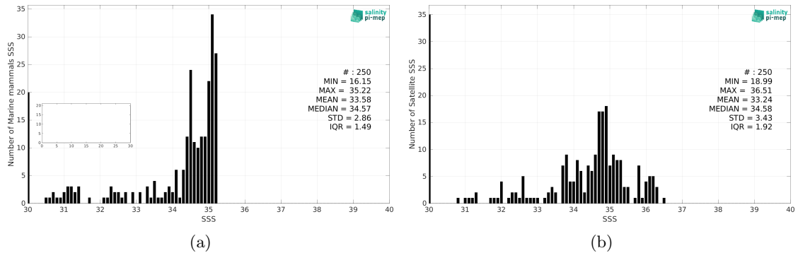
Figure 2: Histograms of SSS from Marine mammals (a) and SMOS SSS L3 v332 - 9 Days (CATDS-CPDC) (b) considering all match-up pairs per bins of 0.1 over the Arctic Ocean Pi-MEP region and for the full satellite product period.
