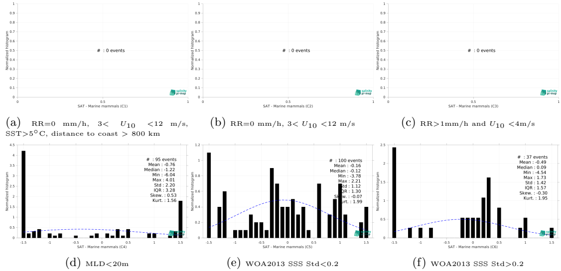
Figure 13: Normalized histogram of \Delta SSS (SMOS SSS L3 v332 - 9 Days (CATDS-CPDC) - Marine mammals) for 6 different subdatasets corresponding to: RR=0 mm/h, 3 < U_{10} < 12 m/s, SST>5°C, distance to coast > 800 km (a), RR=0 mm/h, 3 < U_{10} < 12 m/s (b), RR>1mm/h and U_{10} < 4 m/s (c), MLD<20m (d), WOA2013 SSS Std<0.2 (e), WOA2013 SSS Std>0.2 (f).
