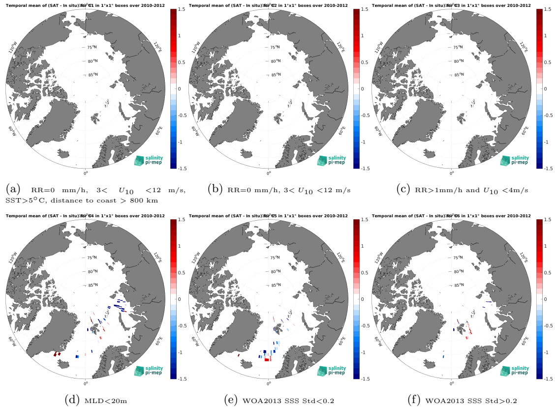
Figure 12: Temporal mean gridded over spatial boxes of size 1^{\circ}\times 1^{\circ} of \Delta\text{SSS} (SMOS SSS L3 v332 - 9 Days (CATDS-CPDC) - Marine mammals) for 6 different subdatasets corresponding to: RR=0 mm/h, 3 < U_{10} < 12 m/s, SST > 5^{\circ}\text{C} , distance to coast > 800 km (a), RR=0 mm/h, 3 < U_{10} < 12 m/s (b), RR > 1\text{mm/h} and U_{10} < 4\text{m/s} (c), MLD < 20\text{m} (d), WOA2013 SSS Std < 0.2 (e), WOA2013 SSS Std > 0.2 (f).
