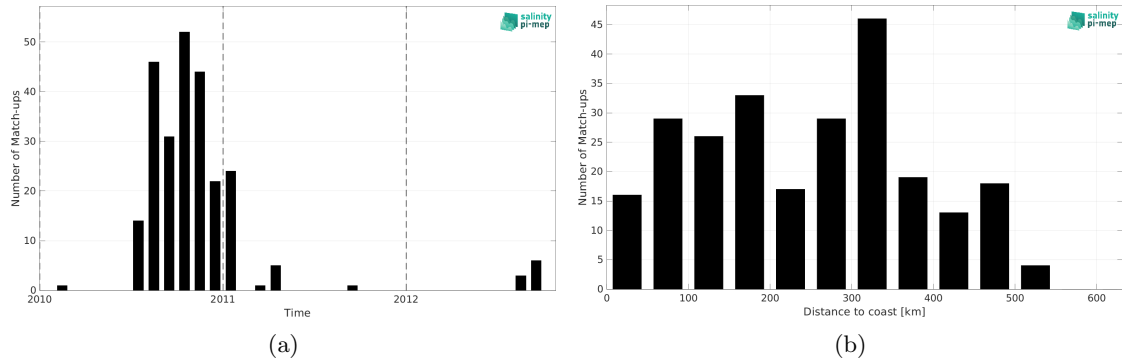
Figure 1: Number of match-ups between Marine mammals and SMOS SSS L3 v332 - 9 Days (CATDS-CPDC) SSS as a function of time (a) and as function of the distance to coast (b) over the Arctic Ocean Pi-MEP region and for the full satellite product period.
