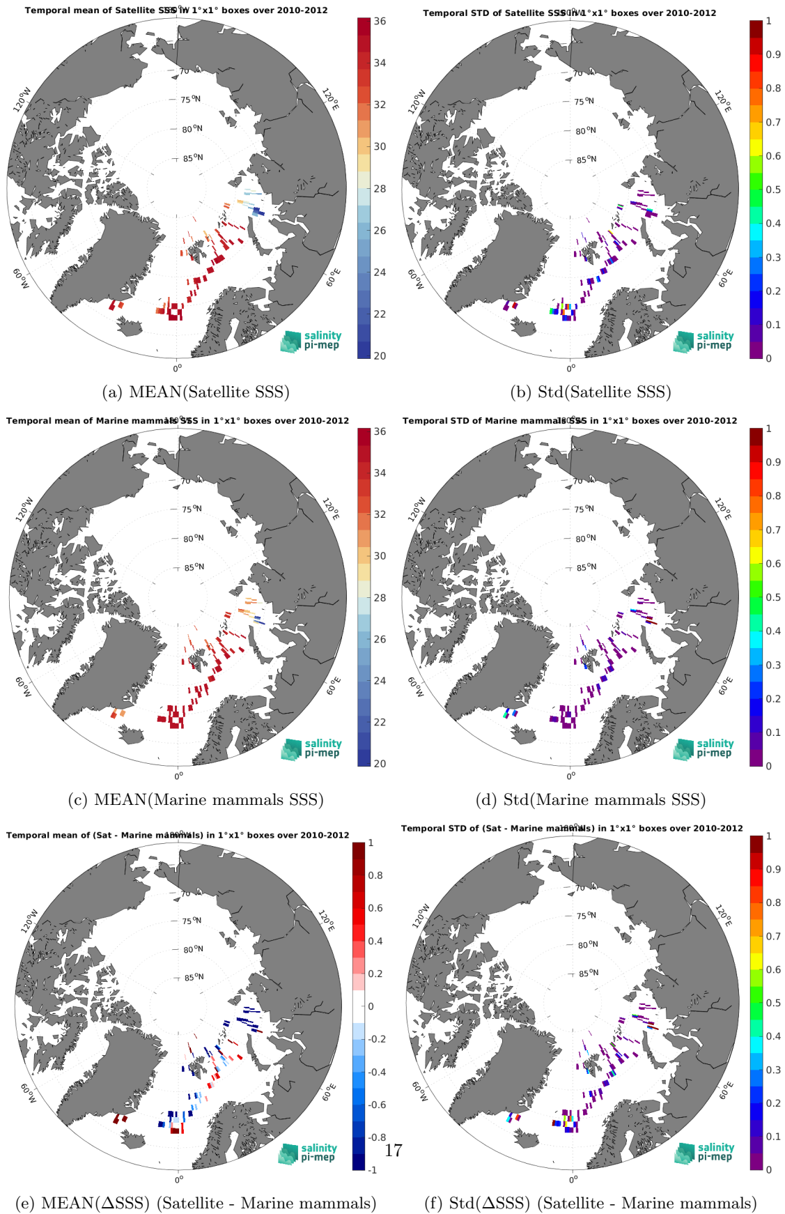
Figure 6: Temporal mean (left) and Std (right) of SSS from SMOS SSS L3 v332 - 9 Days (CATDS-CPDC) (top), Marine mammals (middle), and of \Delta SSS (Satellite - Marine mammals). Only match-up pairs are used to generate these maps.
