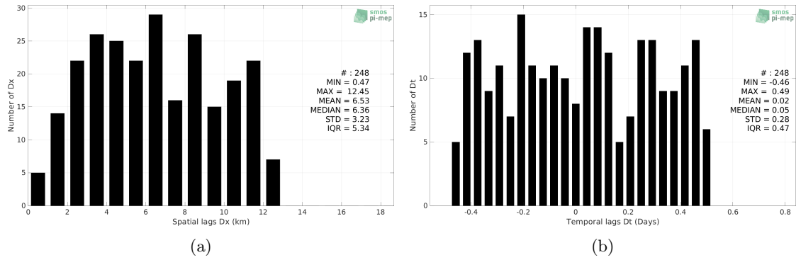
Figure 5: Histograms of the spatial (a) and temporal (b) lags between the location/time of the Marine mammals measurement and the date of the corresponding SMOS SSS L3 v332 - 9 Days (CATDS-CPDC) SSS pixel.
