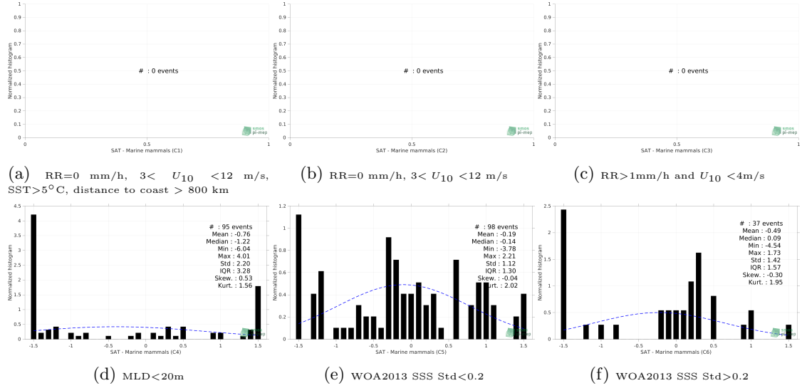
Figure 13: Normalized histogram of \Delta SSS (SMOS SSS L3 v332 - 9 Days (CATDS-CPDC) - Marine mammals) for 6 different subdatasets corresponding to: RR=0 mm/h, 3 < U_{10} < 12 m/s, SST > 5°C, distance to coast > 800 km (a), RR=0 mm/h, 3 < U_{10} < 12 m/s (b), RR > 1mm/h and U_{10} < 4 m/s (c), MLD < 20m (d), WOA2013 SSS Std < 0.2 (e), WOA2013 SSS Std > 0.2 (f).
