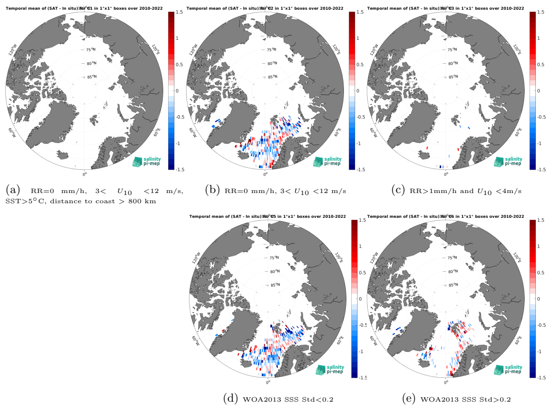
Figure 14: Temporal mean gridded over spatial boxes of size 1^\circ \times 1^\circ of \Delta\text{SSS} (SMOS SSS L3 v332 - 9 Days (CATDS-CPDC) - ICES) for 5 different subdatasets corresponding to:RR=0 mm/h, 3 < U_{10} < 12 m/s, SST>5°C, distance to coast > 800 km (a), RR=0 mm/h, 3 < U_{10} < 12 m/s (b), RR>1mm/h and U_{10} < 4 m/s (c), WOA2013 SSS Std<0.2 (d), WOA2013 SSS Std>0.2 (e).
