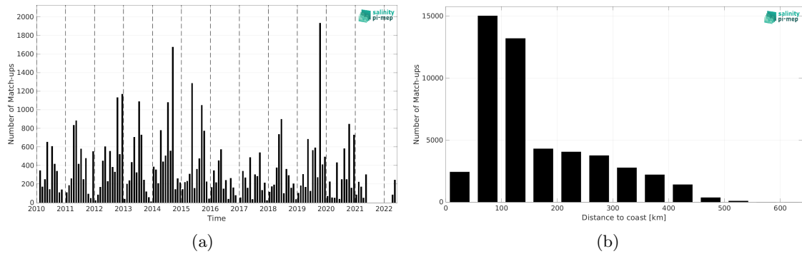
Figure 2: Number of match-ups between ICES and SMOS SSS L3 v332 - 9 Days (CATDS-CPDC) SSS as a function of time (a) and as function of the distance to coast (b) over the Arctic Ocean Pi-MEP region and for the full satellite product period.
