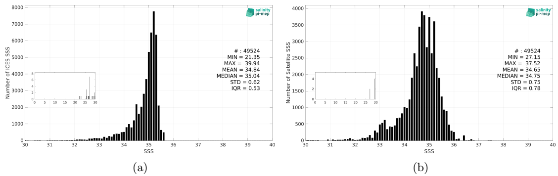
Figure 3: Histograms of SSS from ICES (a) and SMOS SSS L3 v332 - 9 Days (CATDS-CPDC) (b) considering all match-up pairs per bins of 0.1 over the Arctic Ocean Pi-MEP region and for the full satellite product period.
