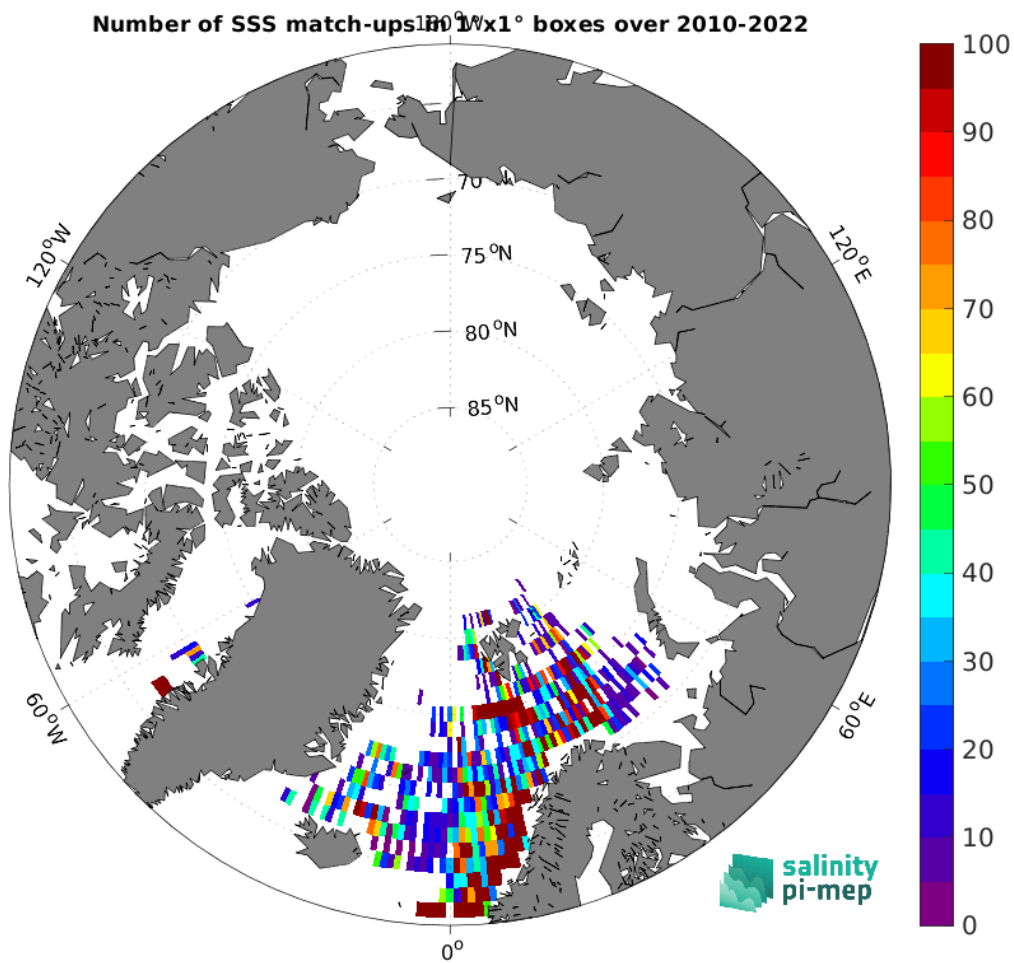
Figure 5: Number of SSS match-ups between ICES SSS and the SMOS SSS L3 v332 - 9 Days (CATDS-CPDC) SSS product for the Arctic Ocean Pi-MEP region over 1^\circ \times 1^\circ boxes and for the full satellite product period.
