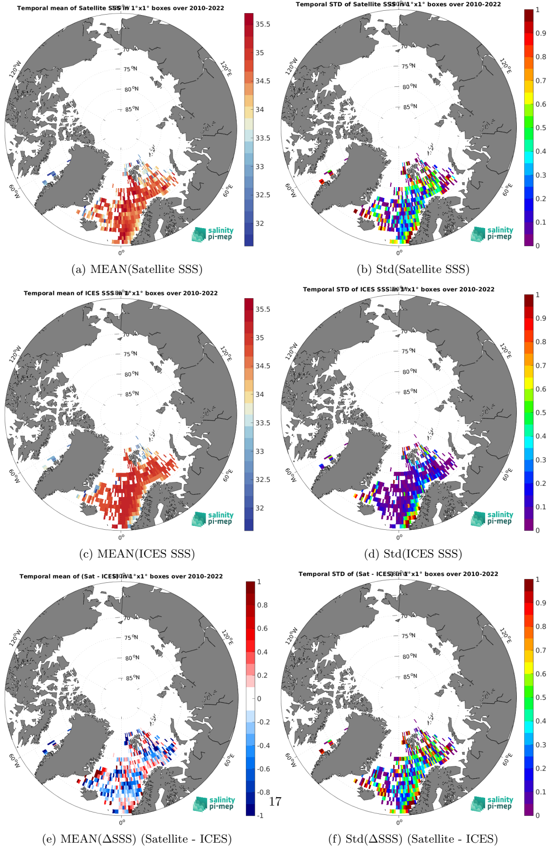
Figure 7: Temporal mean (left) and Std (right) of SSS from SMOS SSS L3 v332 - 9 Days (CATDS-CPDC) (top), ICES (middle), and of \Delta SSS (Satellite - ICES). Only match-up pairs are used to generate these maps.
