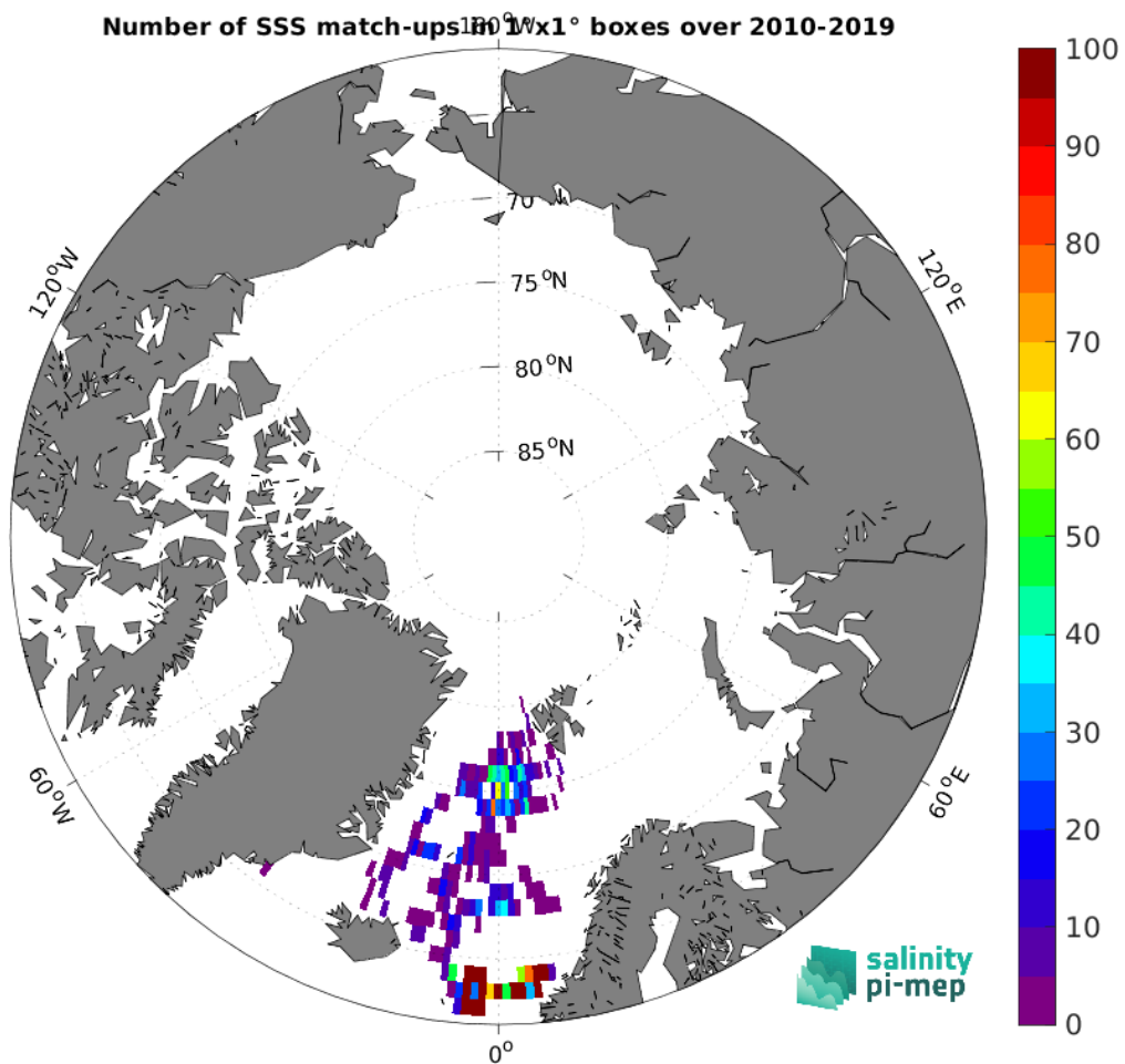
Figure 4: Number of SSS match-ups between Surface drifters SSS and the SMOS SSS L3 v332 - 9 Days (CATDS-CPDC) SSS product for the Arctic Ocean Pi-MEP region over 1^\circ \times 1^\circ boxes and for the full satellite product period.
