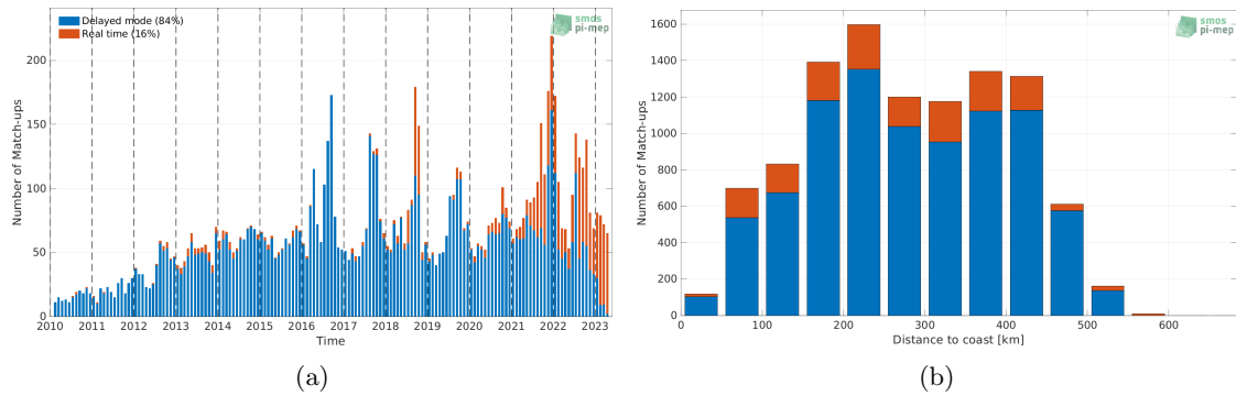
Figure 1: Number of match-ups between Argo and SMOS SSS L3 v332 - 9 Days (CATDS-CPDC) SSS as a function of time (a) and as function of the distance to coast (b) over the Arctic Ocean Pi-MEP region and for the full satellite product period.
