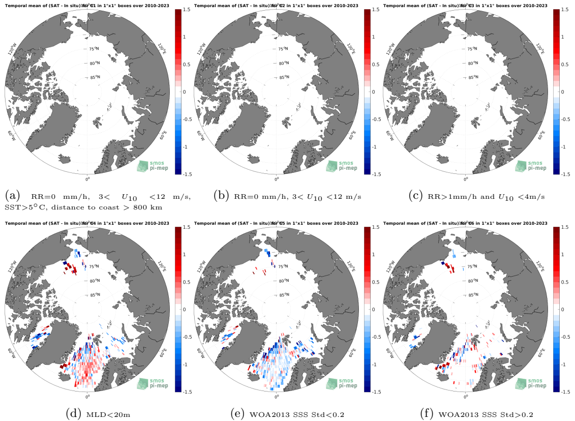
Figure 12: Temporal mean gridded over spatial boxes of size 1^{\circ}\times 1^{\circ} of \Delta\text{SSS} (SMOS SSS L3 v332 - 9 Days (CATDS-CPDC) - Argo) for 6 different subdatasets corresponding to:RR=0 mm/h, 3 < U_{10} < 12 m/s, SST > 5^{\circ}\text{C} , distance to coast > 800 km (a), RR=0 mm/h, 3 < U_{10} < 12 m/s (b), RR > 1\text{mm/h} and U_{10} < 4\text{m/s} (c),MLD < 20\text{m} (d),WOA2013 SSS Std < 0.2 (e),WOA2013 SSS Std > 0.2 (f).
