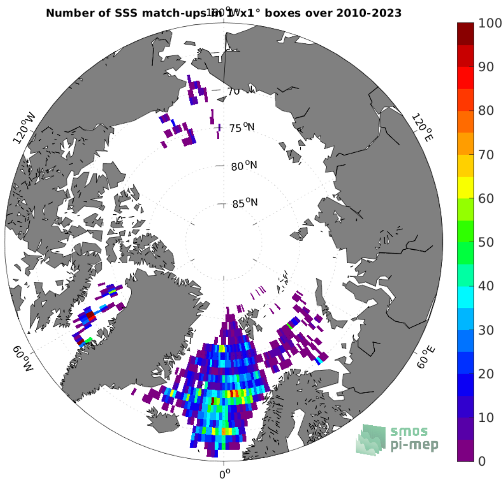
Figure 4: Number of SSS match-ups between Argo SSS and the SMOS SSS L3 v332 - 9 Days (CATDS-CPDC) SSS product for the Arctic Ocean Pi-MEP region over 1^\circ \times 1^\circ boxes and for the full satellite product period.
