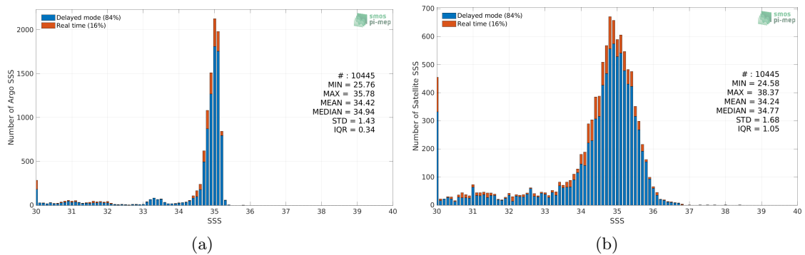
Figure 2: Histograms of SSS from Argo (a) and SMOS SSS L3 v332 - 9 Days (CATDS-CPDC) (b) considering all match-up pairs per bins of 0.1 over the Arctic Ocean Pi-MEP region and for the full satellite product period.
