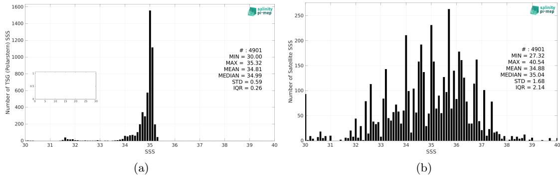
Figure 2: Histograms of SSS from TSG (Polarstern) (a) and SMOS SSS L2Q v331 - 0.25 Deg (CATDS-CPDC) (b) considering all match-up pairs per bins of 0.1 over the Arctic Ocean Pi-MEP region and for the full satellite product period.
