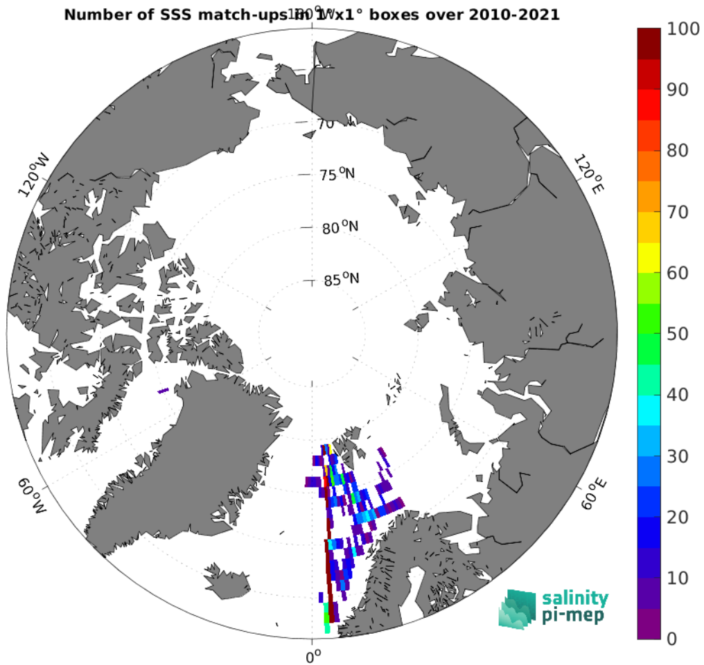
Figure 4: Number of SSS match-ups between TSG (Polarstern) SSS and the SMOS SSS L2Q v331 - 0.25 Deg (CATDS-CPDC) SSS product for the Arctic Ocean Pi-MEP region over 1^\circ \times 1^\circ boxes and for the full satellite product period.
