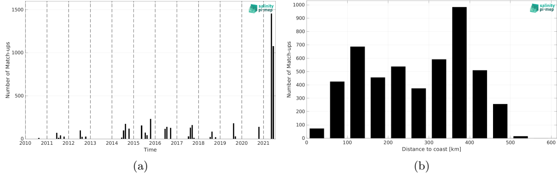
Figure 1: Number of match-ups between TSG (Polarstern) and SMOS SSS L2Q v331 - 0.25 Deg (CATDS-CPDC) SSS as a function of time (a) and as function of the distance to coast (b) over the Arctic Ocean Pi-MEP region and for the full satellite product period.
