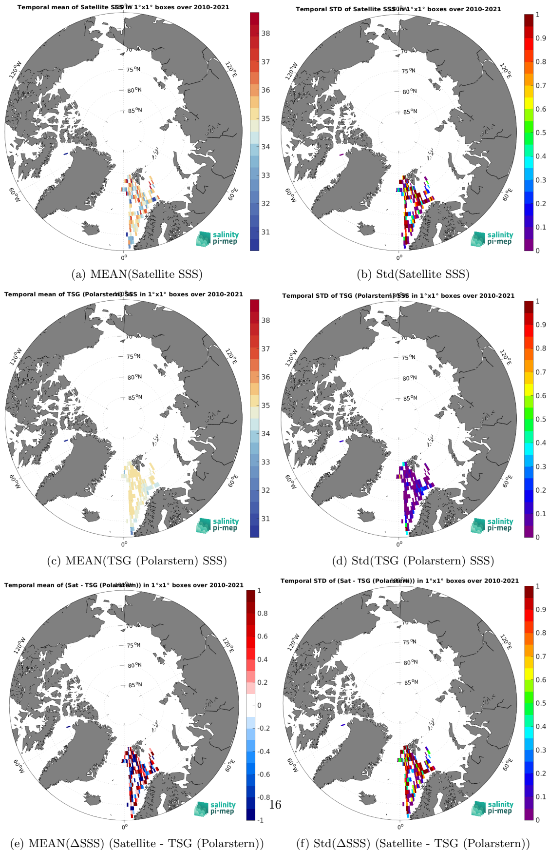
Figure 6: Temporal mean (left) and Std (right) of SSS from SMOS SSS L2Q v331 - 0.25 Deg (CATDS-CPDC) (top), TSG (Polarstern) (middle), and of \Delta SSS (Satellite - TSG (Polarstern)). Only match-up pairs are used to generate these maps.
