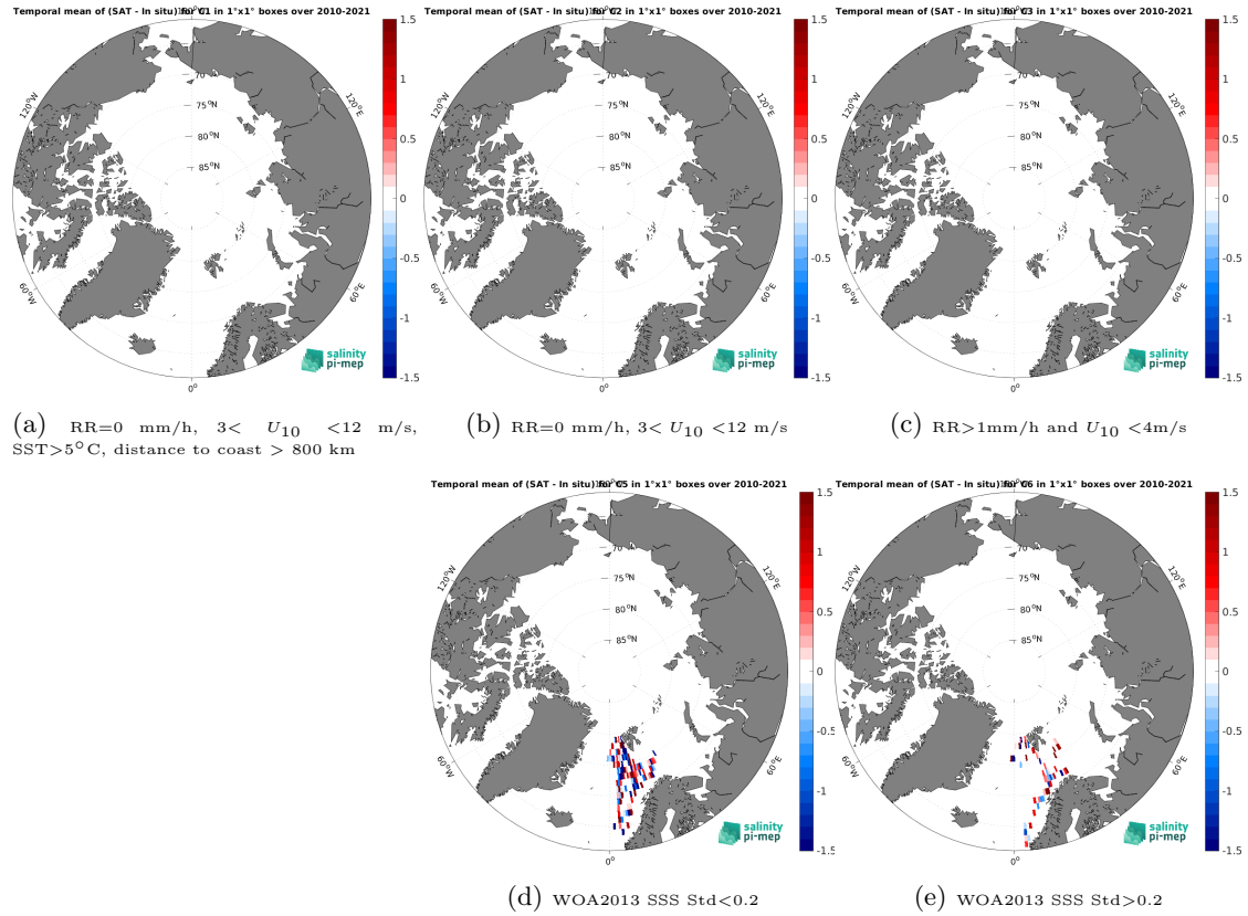
Figure 12: Temporal mean gridded over spatial boxes of size 1^{\circ}\times 1^{\circ} of \Delta\text{SSS} (SMOS SSS L2Q v331 - 0.25 Deg (CATDS-CPDC) - TSG (Polarstern)) for 5 different subdatasets corresponding to:RR=0 mm/h, 3 < U_{10} < 12 m/s, SST >5^{\circ}\text{C} , distance to coast > 800 km (a), RR=0 mm/h, 3 < U_{10} < 12 m/s (b), RR >1 mm/h and U_{10} < 4 m/s (c), WOA2013 SSS Std <0.2 (d), WOA2013 SSS Std >0.2 (e).
