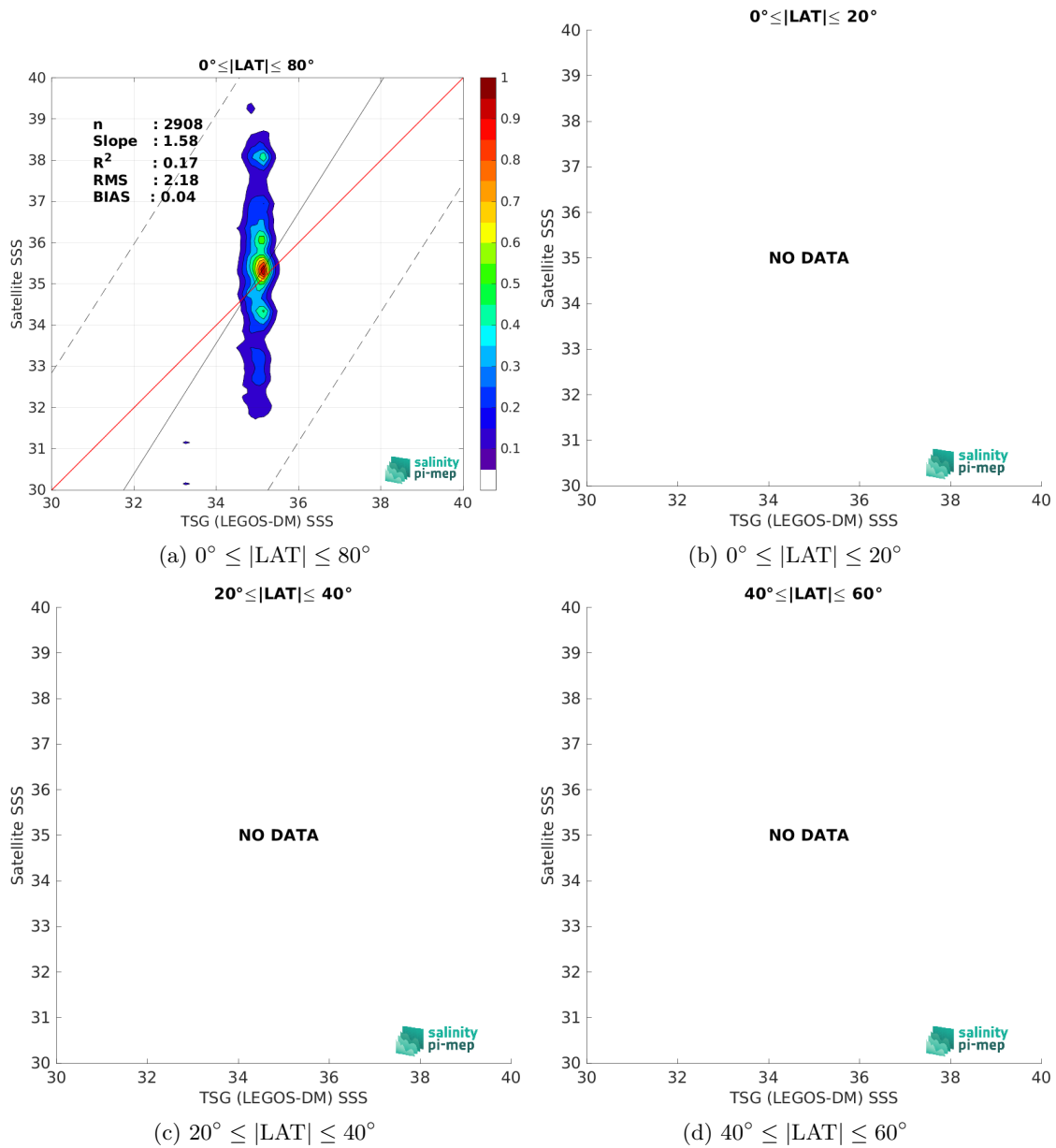
Figure 9: Contour maps of the concentration of SMOS SSS L2Q v331 - 0.25 Deg (CATDS-CPDC) SSS (y-axis) versus TSG (LEGOS-DM) SSS (x-axis) at match-up pairs for different latitude bands. For each plot, the red line shows x=y . The black thin and dashed lines indicate a linear fit through the data cloud and the \pm 95\% confidence levels, respectively. The number match-up pairs n , the slope and R^2 coefficient of the linear fit, the root mean square (RMS) and the mean bias between satellite and in situ data are indicated for each latitude band in each plots.
