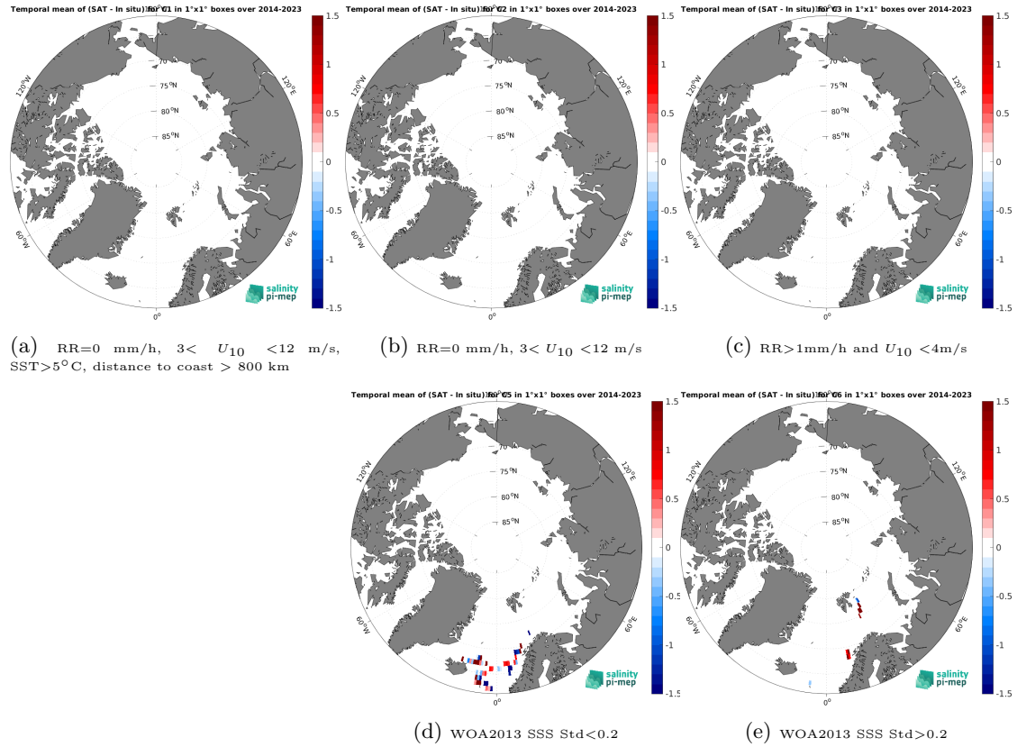
Figure 12: Temporal mean gridded over spatial boxes of size 1^{\circ}\times 1^{\circ} of \Delta\text{SSS} (SMOS SSS L2Q v331 - 0.25 Deg (CATDS-CPDC) - TSG (LEGOS-DM)) for 5 different subdatasets corresponding to: RR=0 mm/h, 3 < U_{10} < 12 m/s, SST > 5^{\circ}\text{C} , distance to coast > 800 km (a), RR=0 mm/h, 3 < U_{10} < 12 m/s (b), RR > 1 mm/h and U_{10} < 4 m/s (c), WOA2013 SSS Std < 0.2 (d), WOA2013 SSS Std > 0.2 (e).
