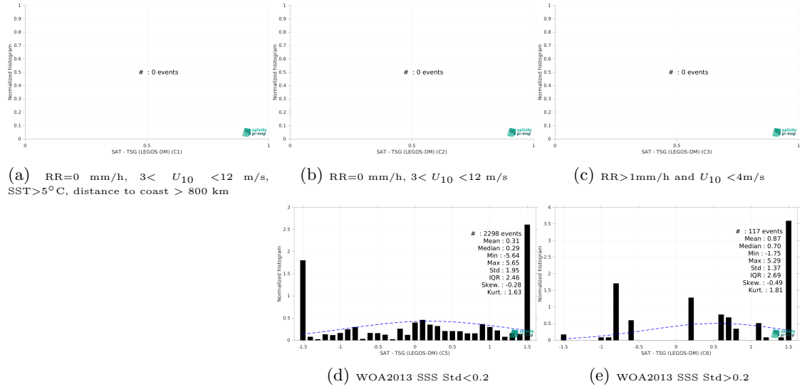
Figure 13: Normalized histogram of \Delta SSS (SMOS SSS L2Q v331 - 0.25 Deg (CATDS-CPDC) - TSG (LEGOS-DM)) for 5 different subdatasets corresponding to: RR=0 mm/h, 3 < U_{10} < 12 m/s, SST>5°C, distance to coast > 800 km (a), RR=0 mm/h, 3 < U_{10} < 12 m/s (b), RR>1mm/h and U_{10} < 4 m/s (c), WOA2013 SSS Std<0.2 (d), WOA2013 SSS Std>0.2 (e).
