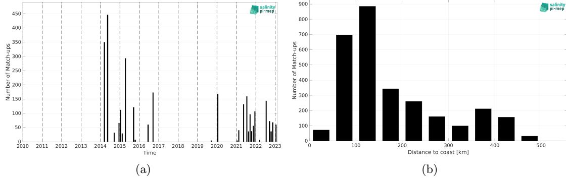
Figure 1: Number of match-ups between TSG (LEGOS-DM) and SMOS SSS L2Q v331 - 0.25 Deg (CATDS-CPDC) SSS as a function of time (a) and as function of the distance to coast (b) over the Arctic Ocean Pi-MEP region and for the full satellite product period.
