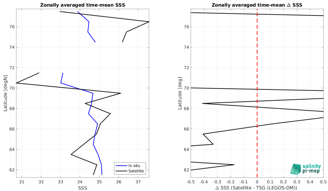
Figure 8: Left panel: Zonal mean SSS from SMOS SSS L2Q v331 - 0.25 Deg (CATDS-CPDC) satellite product (black) and from TSG (LEGOS-DM) (blue). Right panel: Zonal mean of \Delta SSS (Satellite - TSG (LEGOS-DM)) for all the collected Pi-MEP match-up pairs estimated over the full satellite product period.
