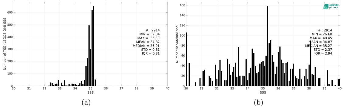
Figure 2: Histograms of SSS from TSG (LEGOS-DM) (a) and SMOS SSS L2Q v331 - 0.25 Deg (CATDS-CPDC) (b) considering all match-up pairs per bins of 0.1 over the Arctic Ocean Pi-MEP region and for the full satellite product period.
