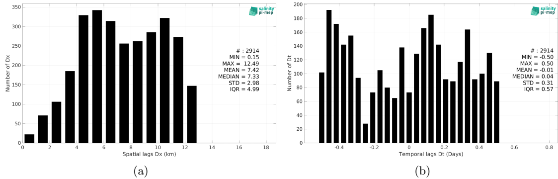
Figure 5: Histograms of the spatial (a) and temporal (b) lags between the location/time of the TSG (LEGOS-DM) measurement and the date of the corresponding SMOS SSS L2Q v331 - 0.25 Deg (CATDS-CPDC) SSS pixel.
