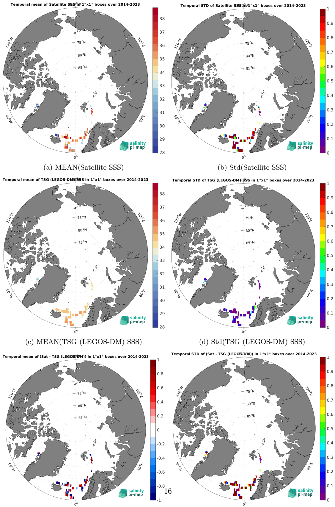
Figure 6: Temporal mean (left) and Std (right) of SSS from SMOS SSS L2Q v331 - 0.25 Deg (CATDS-CPDC) (top), TSG (LEGOS-DM) (middle), and of \Delta SSS (Satellite - TSG (LEGOS-DM)). Only match-up pairs are used to generate these maps.
