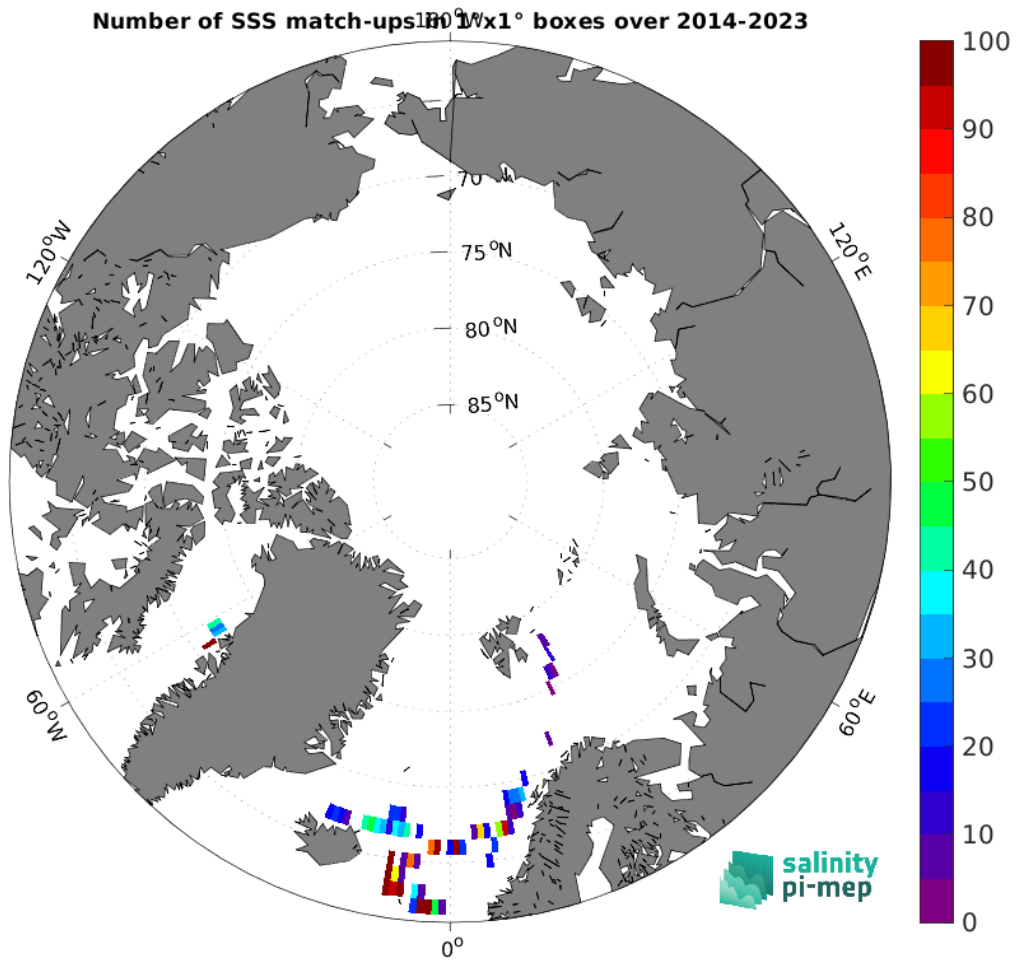
Figure 4: Number of SSS match-ups between TSG (LEGOS-DM) SSS and the SMOS SSS L2Q v331 - 0.25 Deg (CATDS-CPDC) SSS product for the Arctic Ocean Pi-MEP region over 1^\circ \times 1^\circ boxes and for the full satellite product period.
