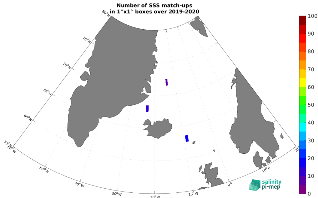
Figure 4: Number of SSS match-ups between TSG (Lauge-Koch) SSS and the SMOS SSS L2Q v331 - 0.25 Deg (CATDS-CPDC) SSS product for the Arctic Ocean Pi-MEP region over 1^\circ \times 1^\circ boxes and for the full satellite product period.
