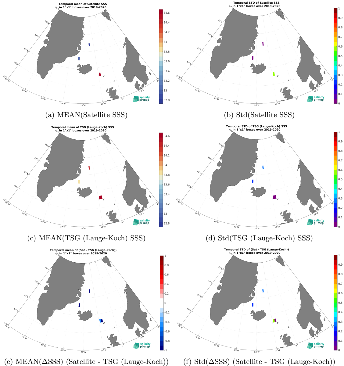
Figure 6: Temporal mean (left) and Std (right) of SSS from SMOS SSS L2Q v331 - 0.25 Deg (CATDS-CPDC) (top), TSG (Lauge-Koch) (middle), and of \Delta SSS (Satellite - TSG (Lauge-Koch)). Only match-up pairs are used to generate these maps.
