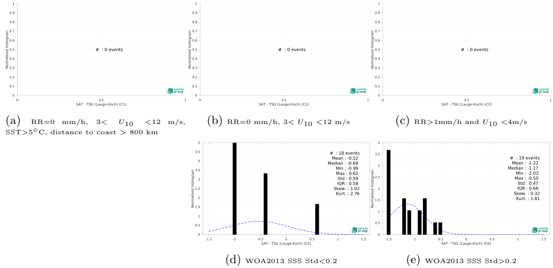
Figure 13: Normalized histogram of \Delta SSS (SMOS SSS L2Q v331 - 0.25 Deg (CATDS-CPDC) - TSG (Lauge-Koch)) for 5 different subdatasets corresponding to: RR=0 mm/h, 3 < U_{10} < 12 m/s, SST > 5°C, distance to coast > 800 km (a), RR=0 mm/h, 3 < U_{10} < 12 m/s (b), RR > 1mm/h and U_{10} < 4 m/s (c), WOA2013 SSS Std < 0.2 (d), WOA2013 SSS Std > 0.2 (e).
