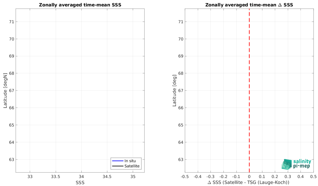
Figure 8: Left panel: Zonal mean SSS from SMOS SSS L2Q v331 - 0.25 Deg (CATDS-CPDC) satellite product (black) and from TSG (Lauge-Koch) (blue). Right panel: Zonal mean of \Delta SSS (Satellite - TSG (Lauge-Koch)) for all the collected Pi-MEP match-up pairs estimated over the full satellite product period.
