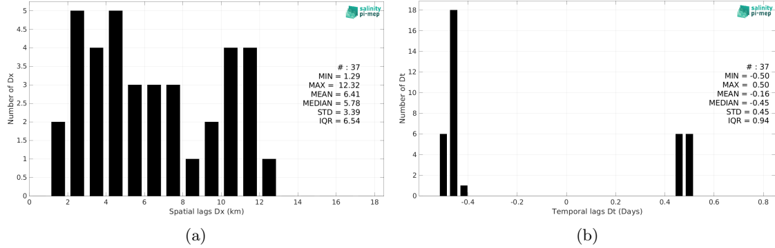
Figure 5: Histograms of the spatial (a) and temporal (b) lags between the location/time of the TSG (Lauge-Koch) measurement and the date of the corresponding SMOS SSS L2Q v331 - 0.25 Deg (CATDS-CPDC) SSS pixel.
