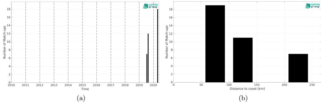
Figure 1: Number of match-ups between TSG (Lauge-Koch) and SMOS SSS L2Q v331 - 0.25 Deg (CATDS-CPDC) SSS as a function of time (a) and as function of the distance to coast (b) over the Arctic Ocean Pi-MEP region and for the full satellite product period.
