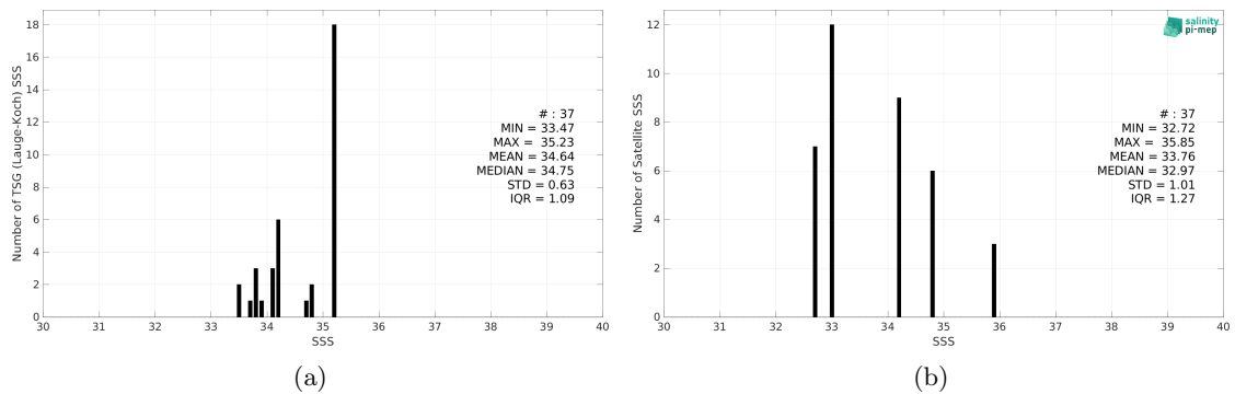
Figure 2: Histograms of SSS from TSG (Lauge-Koch) (a) and SMOS SSS L2Q v331 - 0.25 Deg (CATDS-CPDC) (b) considering all match-up pairs per bins of 0.1 over the Arctic Ocean Pi-MEP region and for the full satellite product period.
