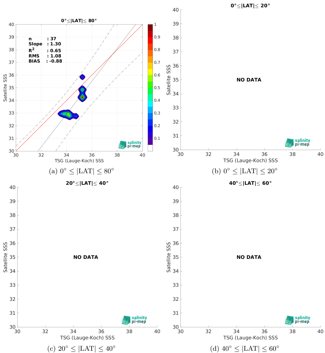
Figure 9: Contour maps of the concentration of SMOS SSS L2Q v331 - 0.25 Deg (CATDS-CPDC) SSS (y-axis) versus TSG (Lauge-Koch) SSS (x-axis) at match-up pairs for different latitude bands. For each plot, the red line shows x=y . The black thin and dashed lines indicate a linear fit through the data cloud and the \pm 95\% confidence levels, respectively. The number match-up pairs n , the slope and R^2 coefficient of the linear fit, the root mean square (RMS) and the mean bias between satellite and in situ data are indicated for each latitude band in each plots.
