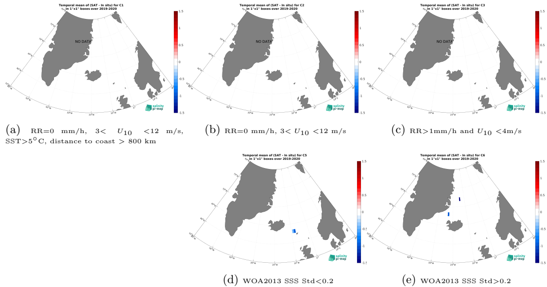
Figure 12: Temporal mean gridded over spatial boxes of size 1^{\circ}\times 1^{\circ} of \Delta\text{SSS} (SMOS SSS L2Q v331 - 0.25 Deg (CATDS-CPDC) - TSG (Lauge-Koch)) for 5 different subdatasets corresponding to:RR=0 mm/h, 3 < U_{10} < 12 m/s, SST > 5^{\circ}\text{C} , distance to coast > 800 km (a), RR=0 mm/h, 3 < U_{10} < 12 m/s (b), RR > 1 mm/h and U_{10} < 4 m/s (c), WOA2013 SSS Std < 0.2 (d), WOA2013 SSS Std > 0.2 (e).
