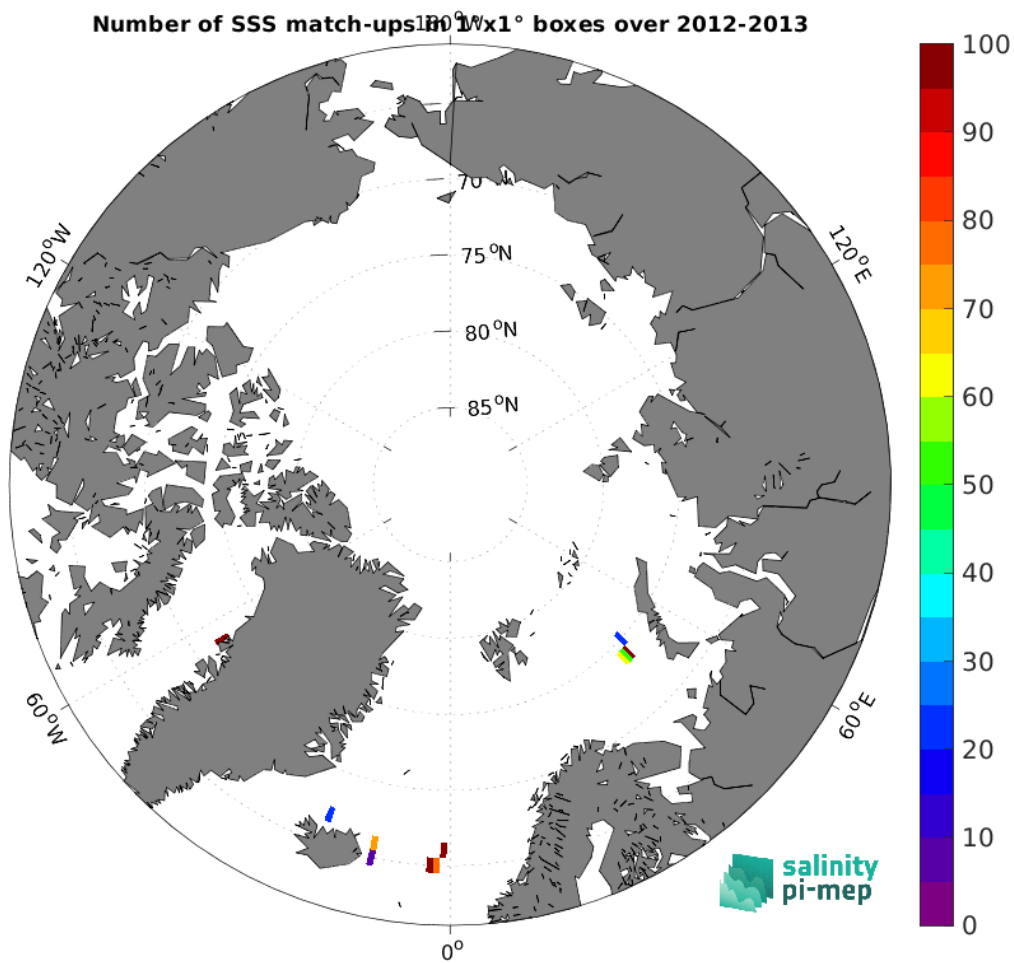
Figure 4: Number of SSS match-ups between TSG (GOSUD-Sailing-ship) SSS and the SMOS SSS L2Q v331 - 0.25 Deg (CATDS-CPDC) SSS product for the Arctic Ocean Pi-MEP region over 1^\circ \times 1^\circ boxes and for the full satellite product period.
