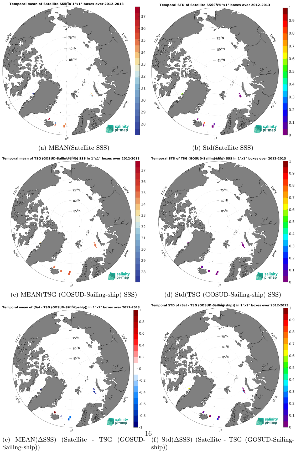
Figure 6: Temporal mean (left) and Std (right) of SSS from SMOS SSS L2Q v331 - 0.25 Deg (CATDS-CPDC) (top), TSG (GOSUD-Sailing-ship) (middle), and of \Delta SSS (Satellite - TSG (GOSUD-Sailing-ship)). Only match-up pairs are used to generate these maps.
