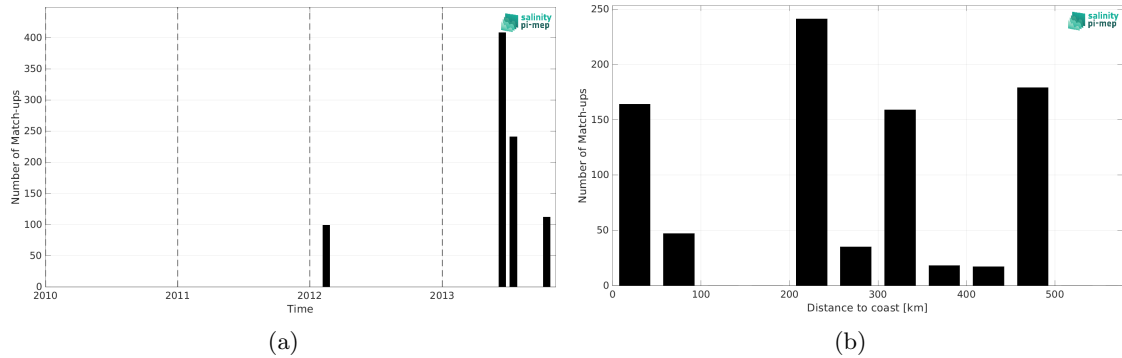
Figure 1: Number of match-ups between TSG (GOSUD-Sailing-ship) and SMOS SSS L2Q v331 - 0.25 Deg (CATDS-CPDC) SSS as a function of time (a) and as function of the distance to coast (b) over the Arctic Ocean Pi-MEP region and for the full satellite product period.
