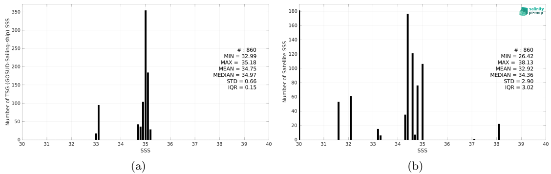
Figure 2: Histograms of SSS from TSG (GOSUD-Sailing-ship) (a) and SMOS SSS L2Q v331 - 0.25 Deg (CATDS-CPDC) (b) considering all match-up pairs per bins of 0.1 over the Arctic Ocean Pi-MEP region and for the full satellite product period.
