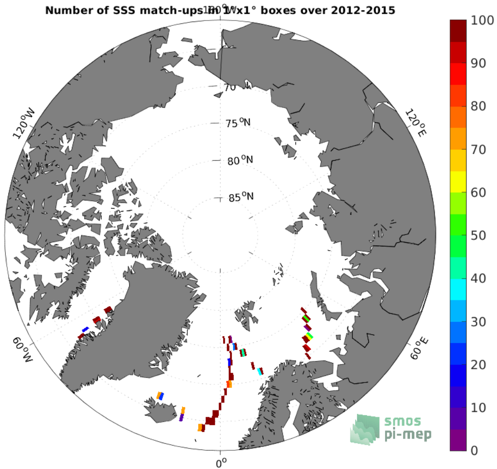
Figure 4: Number of SSS match-ups between TSG (GOSUD-Sailing-ship) SSS and the SMOS SSS L2Q v331 - 0.25 Deg (CATDS-CPDC) SSS product for the Arctic Ocean Pi-MEP region over 1^{\circ} \times 1^{\circ} boxes and for the full satellite product period.
