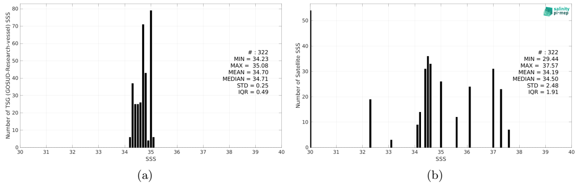
Figure 2: Histograms of SSS from TSG (GOSUD-Research-vessel) (a) and SMOS SSS L2Q v331 - 0.25 Deg (CATDS-CPDC) (b) considering all match-up pairs per bins of 0.1 over the Arctic Ocean Pi-MEP region and for the full satellite product period.
