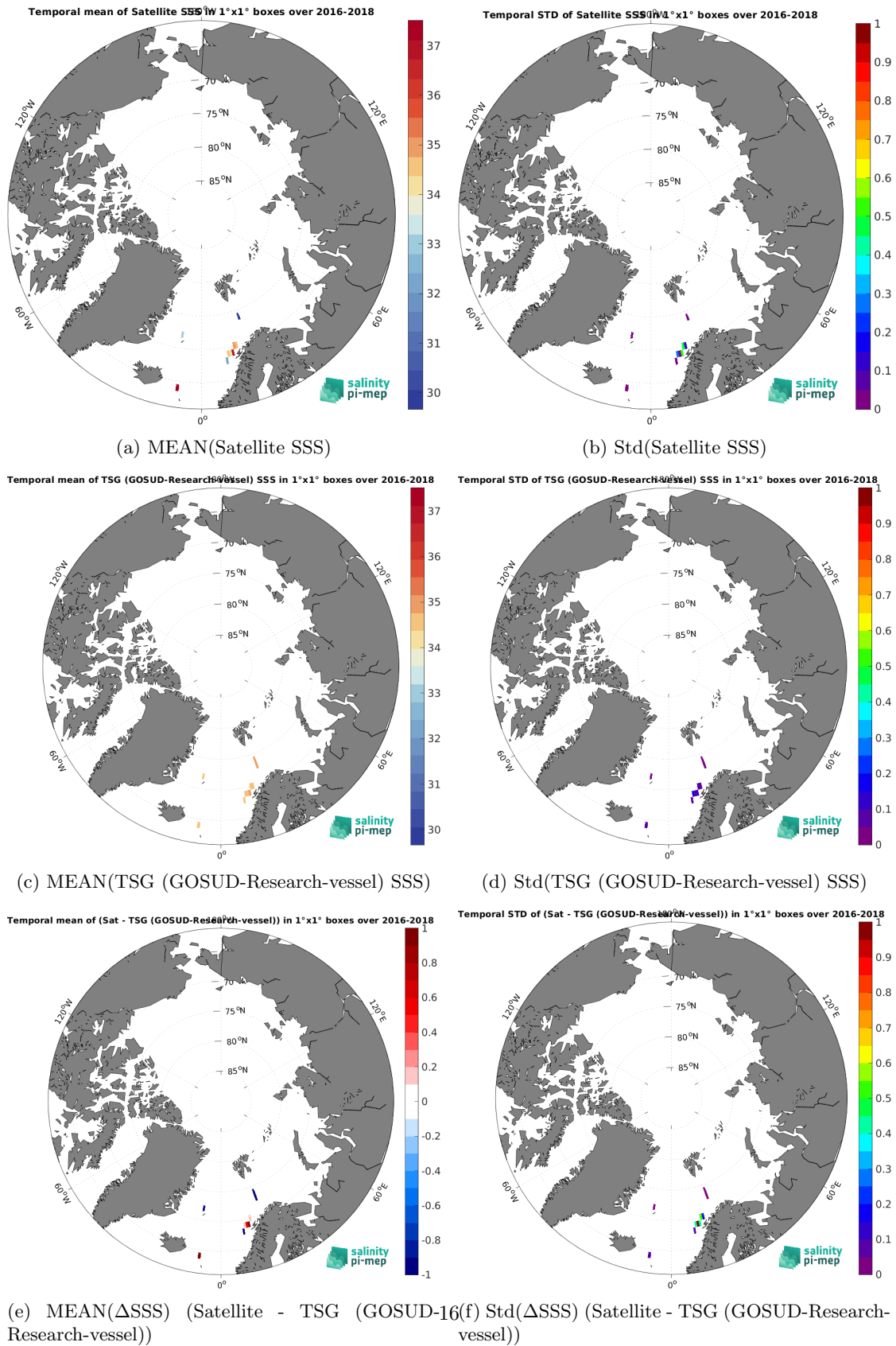
Figure 6: Temporal mean (left) and Std (right) of SSS from SMOS SSS L2Q v331 - 0.25 Deg (CATDS-CPDC) (top), TSG (GOSUD-Research-vessel) (middle), and of \Delta SSS (Satellite - TSG (GOSUD-Research-vessel)). Only match-up pairs are used to generate these maps.
