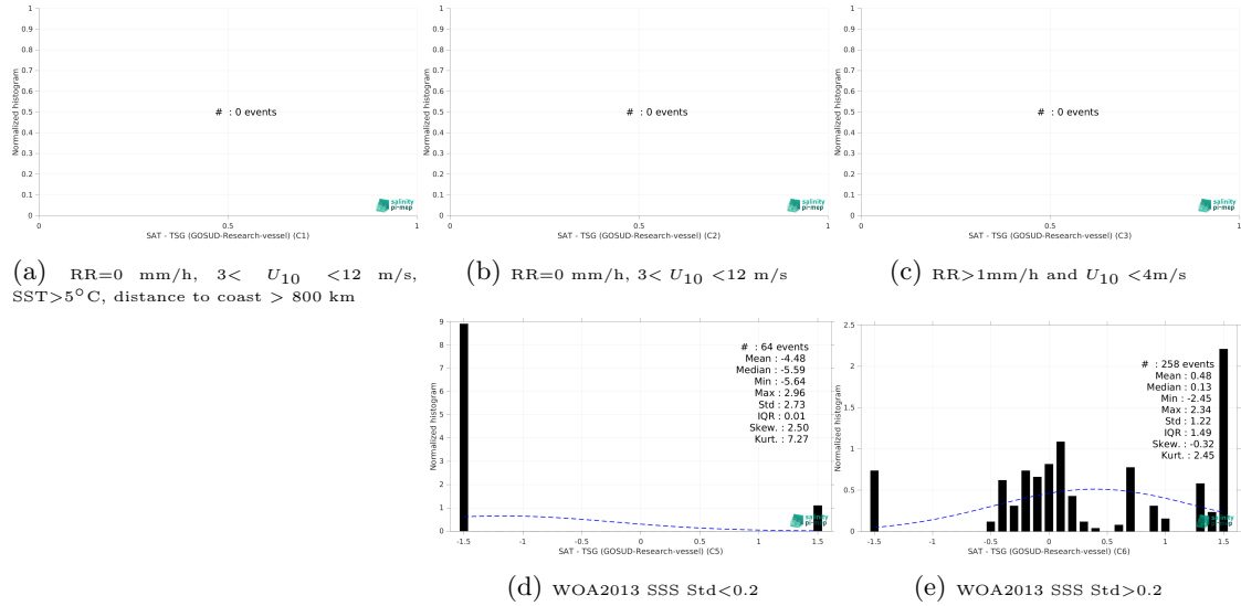
Figure 13: Normalized histogram of \Delta\text{SSS} (SMOS SSS L2Q v331 - 0.25 Deg (CATDS-CPDC) - TSG (GOSUD-Research-vessel)) for 5 different subdatasets corresponding to: RR=0 mm/h, 3 < U_{10} < 12 m/s, SST > 5^\circ\text{C} , distance to coast > 800 km (a), RR=0 mm/h, 3 < U_{10} < 12 m/s (b), RR > 1\text{mm/h} and U_{10} < 4\text{m/s} (c), WOA2013 SSS Std < 0.2 (d), WOA2013 SSS Std > 0.2 (e).
