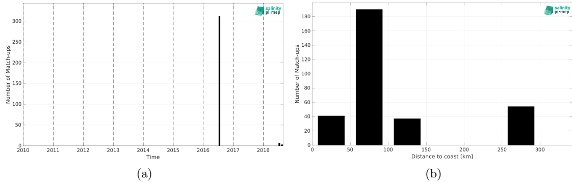
Figure 1: Number of match-ups between TSG (GOSUD-Research-vessel) and SMOS SSS L2Q v331 - 0.25 Deg (CATDS-CPDC) SSS as a function of time (a) and as function of the distance to coast (b) over the Arctic Ocean Pi-MEP region and for the full satellite product period.
