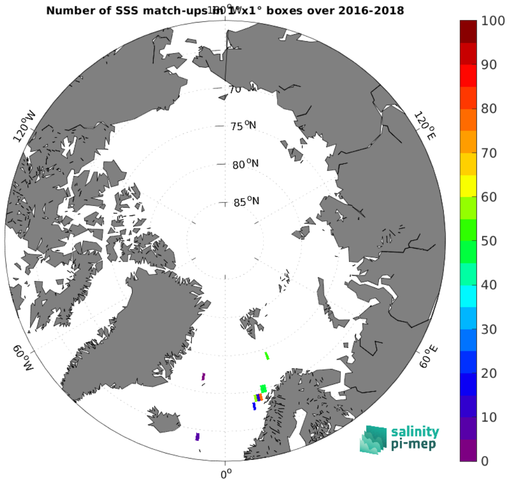
Figure 4: Number of SSS match-ups between TSG (GOSUD-Research-vessel) SSS and the SMOS SSS L2Q v331 - 0.25 Deg (CATDS-CPDC) SSS product for the Arctic Ocean Pi-MEP region over 1^{\circ} \times 1^{\circ} boxes and for the full satellite product period.
