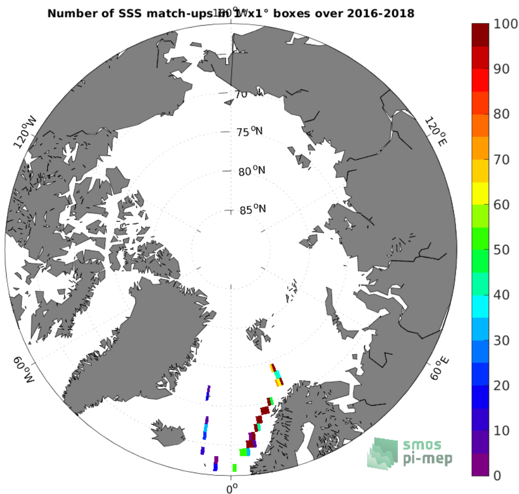
Figure 4: Number of SSS match-ups between TSG (GOSUD-Research-vessel) SSS and the SMOS SSS L2Q v331 - 0.25 Deg (CATDS-CPDC) SSS product for the Arctic Ocean Pi-MEP region over 1^\circ \times 1^\circ boxes and for the full satellite product period.
