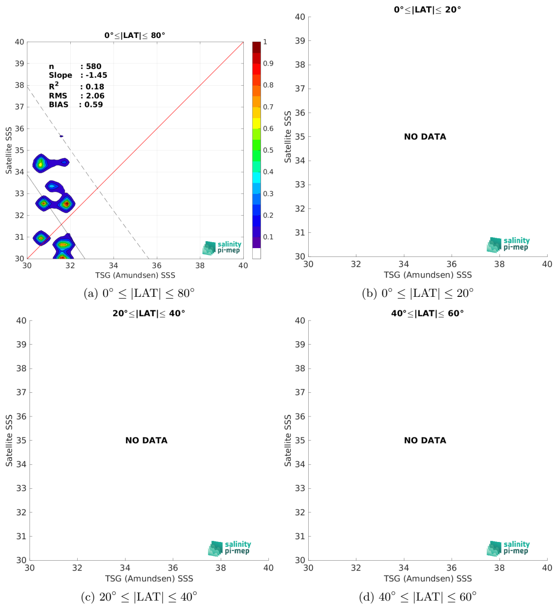
Figure 9: Contour maps of the concentration of SMOS SSS L2Q v331 - 0.25 Deg (CATDS-CPDC) SSS (y-axis) versus TSG (Amundsen) SSS (x-axis) at match-up pairs for different latitude bands. For each plot, the red line shows x=y . The black thin and dashed lines indicate a linear fit through the data cloud and the \pm 95\% confidence levels, respectively. The number match-up pairs n , the slope and R^2 coefficient of the linear fit, the root mean square (RMS) and the mean bias between satellite and in situ data are indicated for each latitude band in each plots.
