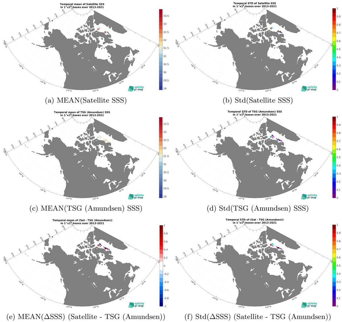
Figure 6: Temporal mean (left) and Std (right) of SSS from SMOS SSS L2Q v331 - 0.25 Deg (CATDS-CPDC) (top), TSG (Amundsen) (middle), and of \Delta SSS (Satellite - TSG (Amundsen)). Only match-up pairs are used to generate these maps.
