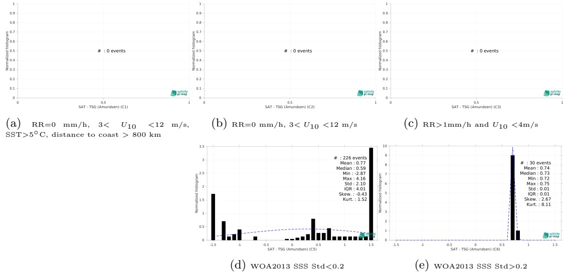
Figure 13: Normalized histogram of \Delta SSS (SMOS SSS L2Q v331 - 0.25 Deg (CATDS-CPDC) - TSG (Amundsen)) for 5 different subdatasets corresponding to: RR=0 mm/h, 3 < U_{10} < 12 m/s, SST > 5°C, distance to coast > 800 km (a), RR=0 mm/h, 3 < U_{10} < 12 m/s (b), RR > 1mm/h and U_{10} < 4 m/s (c), WOA2013 SSS Std < 0.2 (d), WOA2013 SSS Std > 0.2 (e).
