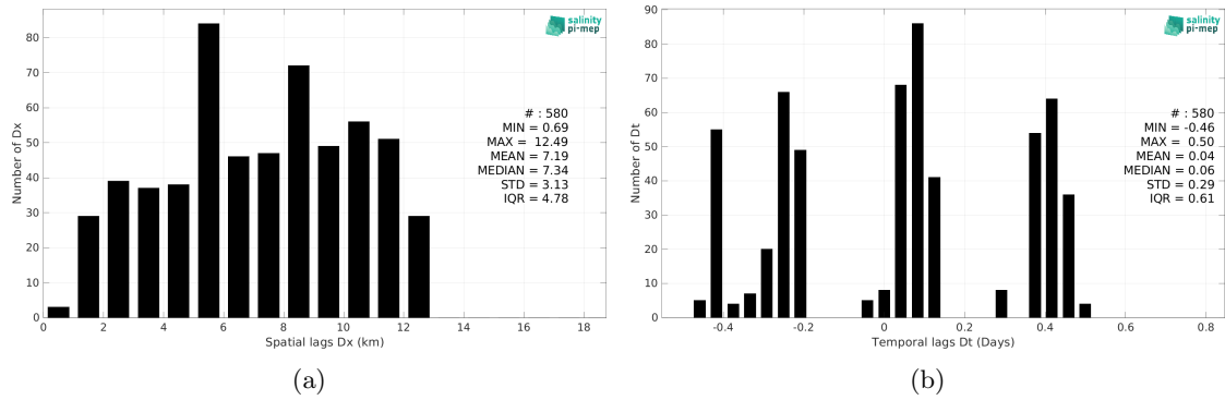
Figure 5: Histograms of the spatial (a) and temporal (b) lags between the location/time of the TSG (Amundsen) measurement and the date of the corresponding SMOS SSS L2Q v331 - 0.25 Deg (CATDS-CPDC) SSS pixel.
