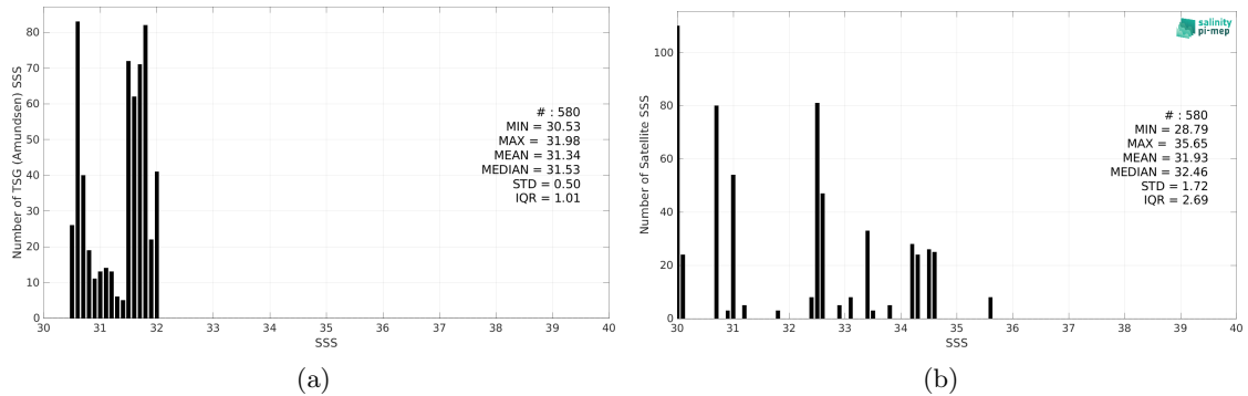
Figure 2: Histograms of SSS from TSG (Amundsen) (a) and SMOS SSS L2Q v331 - 0.25 Deg (CATDS-CPDC) (b) considering all match-up pairs per bins of 0.1 over the Arctic Ocean Pi-MEP region and for the full satellite product period.
