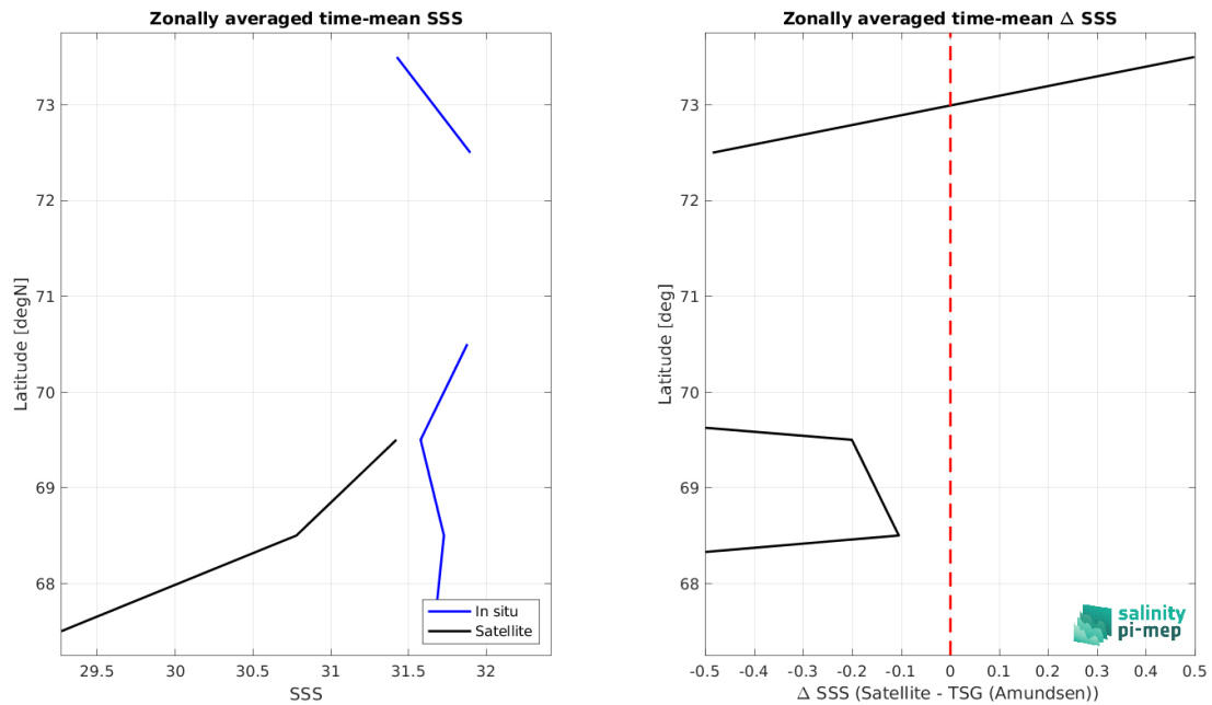
Figure 8: Left panel: Zonal mean SSS from SMOS SSS L2Q v331 - 0.25 Deg (CATDS-CPDC) satellite product (black) and from TSG (Amundsen) (blue). Right panel: Zonal mean of \Delta SSS (Satellite - TSG (Amundsen)) for all the collected Pi-MEP match-up pairs estimated over the full satellite product period.
