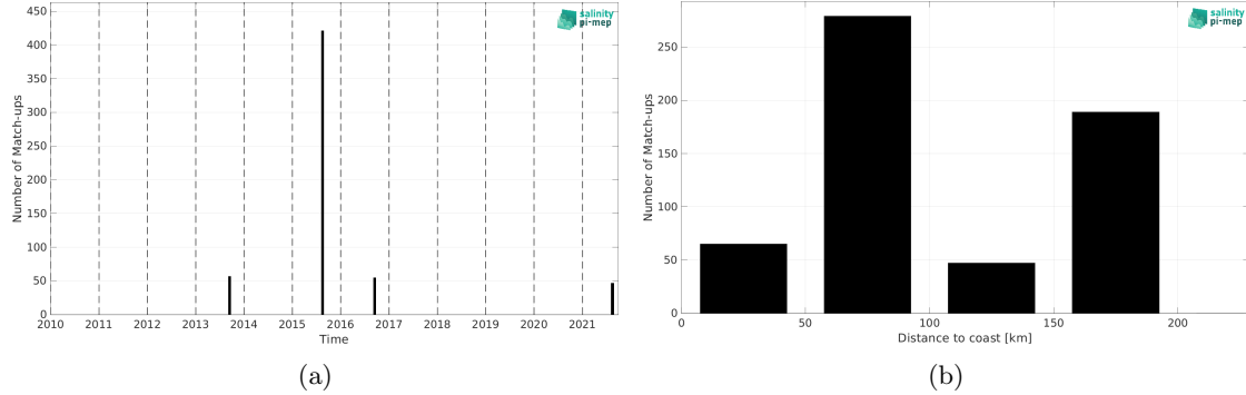
Figure 1: Number of match-ups between TSG (Amundsen) and SMOS SSS L2Q v331 - 0.25 Deg (CATDS-CPDC) SSS as a function of time (a) and as function of the distance to coast (b) over the Arctic Ocean Pi-MEP region and for the full satellite product period.
