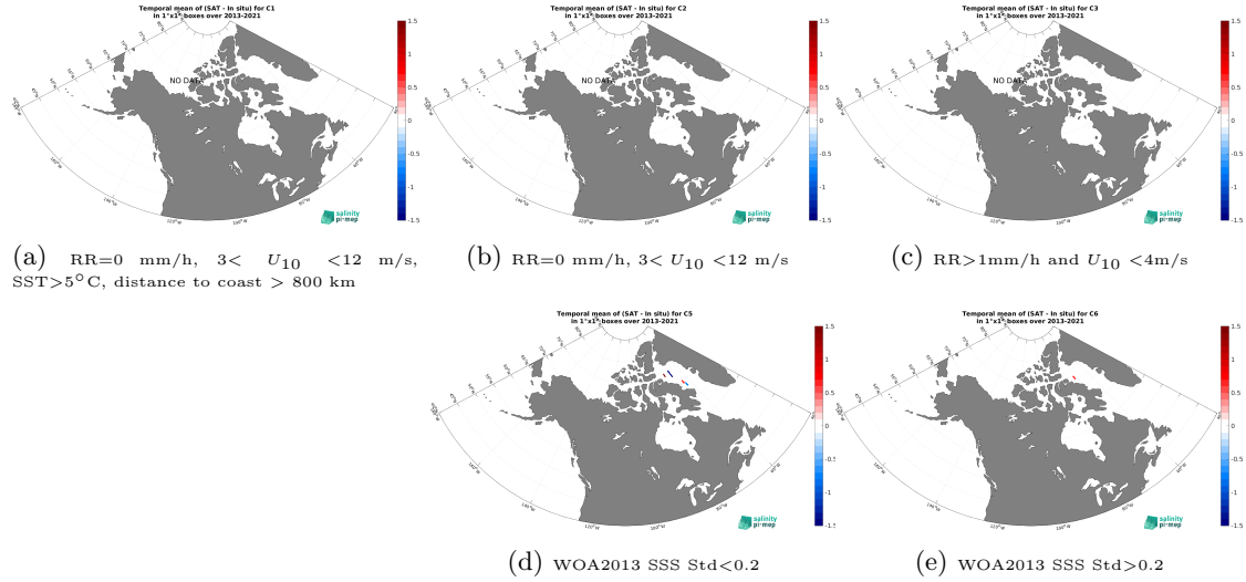
Figure 12: Temporal mean gridded over spatial boxes of size 1^{\circ}\times 1^{\circ} of \Delta\text{SSS} (SMOS SSS L2Q v331 - 0.25 Deg (CATDS-CPDC) - TSG (Amundsen)) for 5 different subdatasets corresponding to:RR=0 mm/h, 3 < U_{10} < 12 m/s, SST >5^{\circ}\text{C} , distance to coast > 800 km (a), RR=0 mm/h, 3 < U_{10} < 12 m/s (b), RR >1 mm/h and U_{10} < 4 m/s (c), WOA2013 SSS Std <0.2 (d), WOA2013 SSS Std >0.2 (e).
