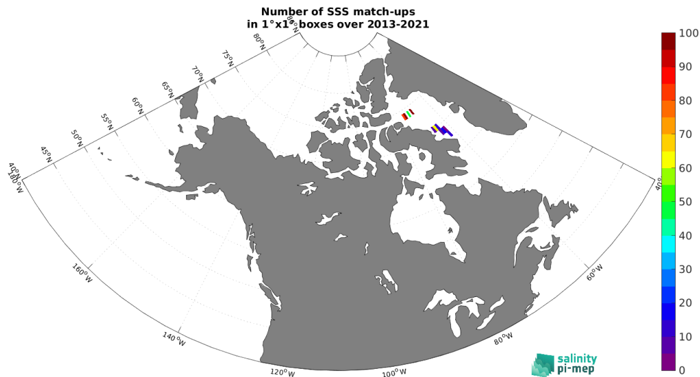
Figure 4: Number of SSS match-ups between TSG (Amundsen) SSS and the SMOS SSS L2Q v331 - 0.25 Deg (CATDS-CPDC) SSS product for the Arctic Ocean Pi-MEP region over 1^\circ \times 1^\circ boxes and for the full satellite product period.
