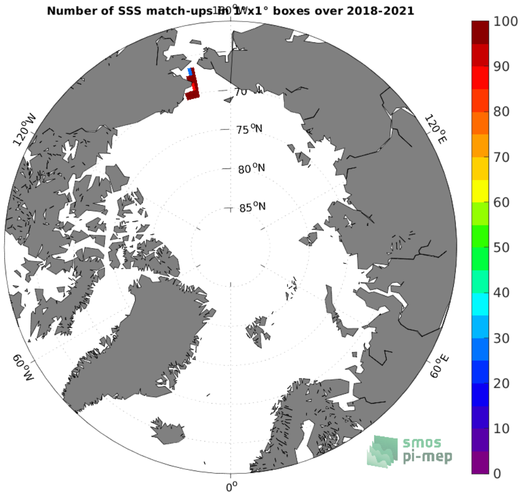
Figure 4: Number of SSS match-ups between Sairdrone SSS and the SMOS SSS L2Q v331 - 0.25 Deg (CATDS-CPDC) SSS product for the Arctic Ocean Pi-MEP region over 1^\circ \times 1^\circ boxes and for the full satellite product period.
