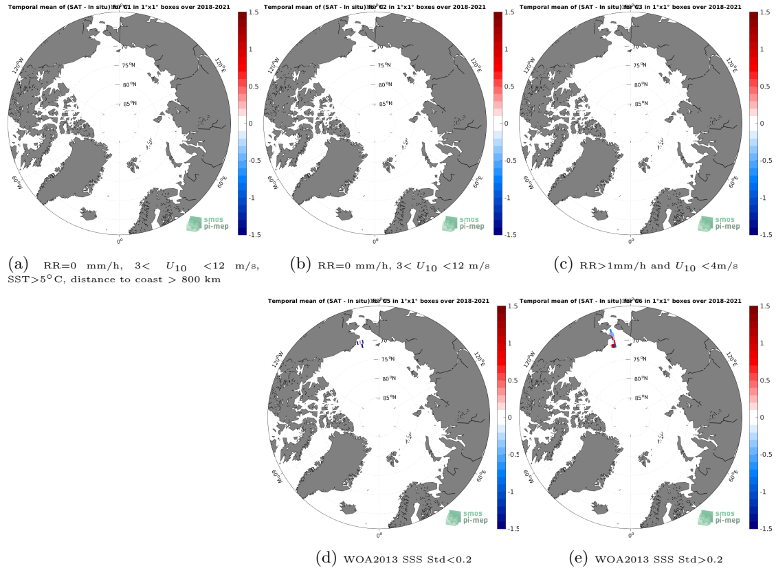
Figure 12: Temporal mean gridded over spatial boxes of size 1^{\circ}\times 1^{\circ} of \Delta\text{SSS} (SMOS SSS L2Q v331 - 0.25 Deg (CATDS-CPDC) - Saildrone) for 5 different subdatasets corresponding to:RR=0 mm/h, 3 < U_{10} < 12 m/s, SST >5^{\circ}\text{C} , distance to coast > 800 km (a), RR=0 mm/h, 3 < U_{10} < 12 m/s (b), RR >1 mm/h and U_{10} < 4 m/s (c), WOA2013 SSS Std <0.2 (d), WOA2013 SSS Std >0.2 (e).
