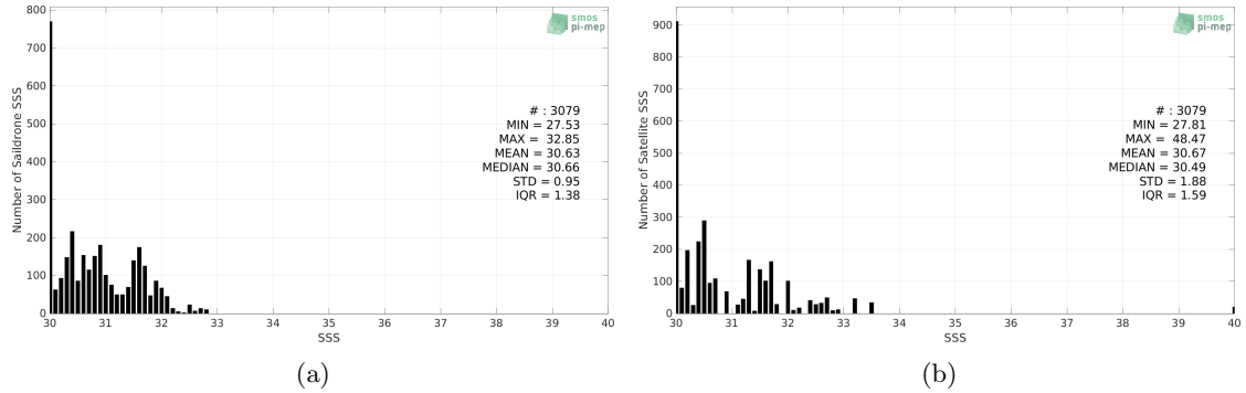
Figure 2: Histograms of SSS from Saildrone (a) and SMOS SSS L2Q v331 - 0.25 Deg (CATDS-CPDC) (b) considering all match-up pairs per bins of 0.1 over the Arctic Ocean Pi-MEP region and for the full satellite product period.
