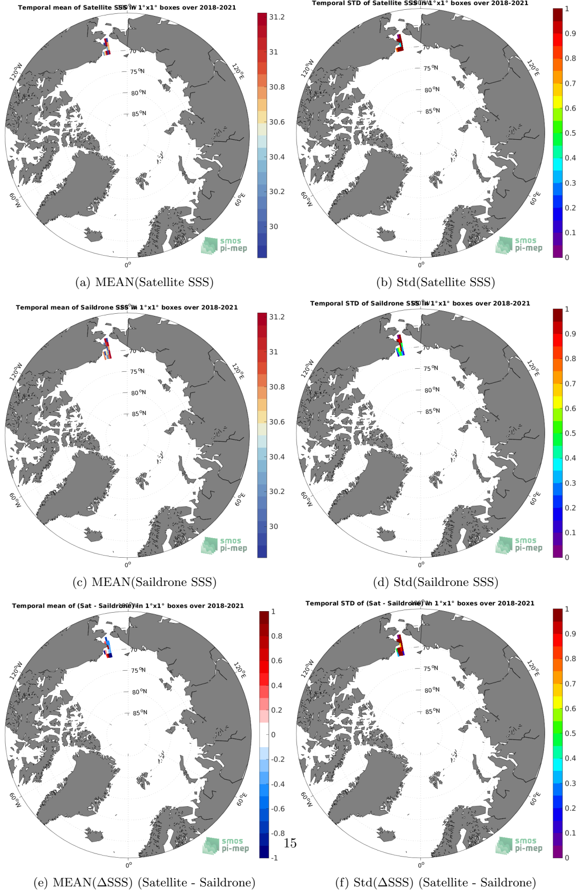
Figure 6: Temporal mean (left) and Std (right) of SSS from SMOS SSS L2Q v331 - 0.25 Deg (CATDS-CPDC) (top), Saildrone (middle), and of \Delta SSS (Satellite - Saildrone). Only match-up pairs are used to generate these maps.
