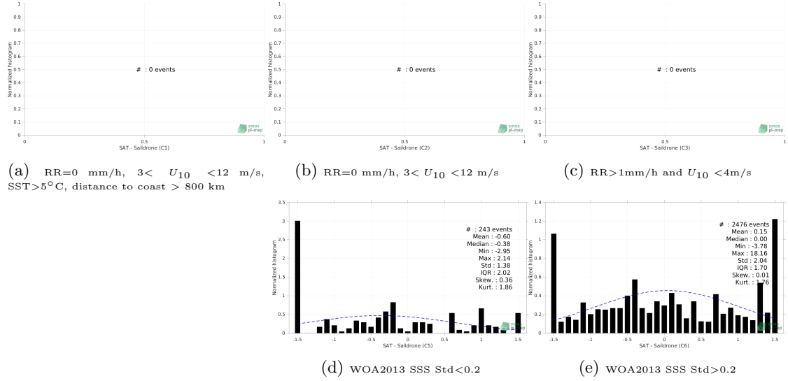
Figure 13: Normalized histogram of \Delta SSS (SMOS SSS L2Q v331 - 0.25 Deg (CATDS-CPDC) - Saildrone) for 5 different subdatasets corresponding to: RR=0 mm/h, 3 < U_{10} < 12 m/s, SST > 5°C, distance to coast > 800 km (a), RR=0 mm/h, 3 < U_{10} < 12 m/s (b), RR > 1mm/h and U_{10} < 4 m/s (c), WOA2013 SSS Std < 0.2 (d), WOA2013 SSS Std > 0.2 (e).
