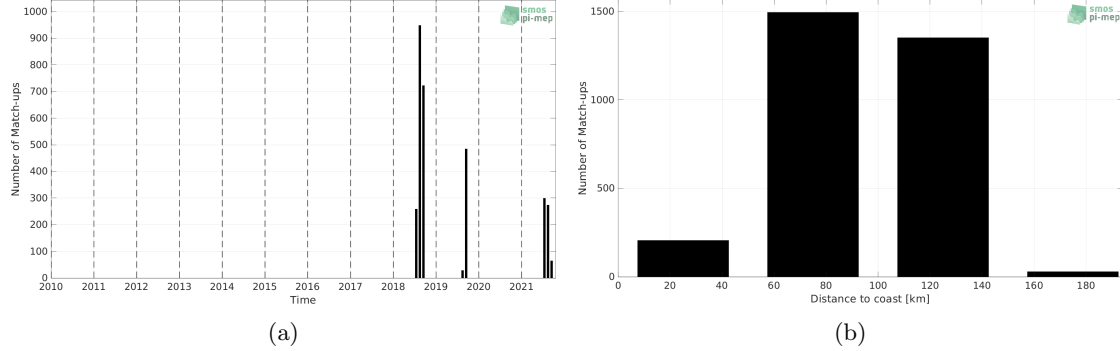
Figure 1: Number of match-ups between Saildrone and SMOS SSS L2Q v331 - 0.25 Deg (CATDS-CPDC) SSS as a function of time (a) and as function of the distance to coast (b) over the Arctic Ocean Pi-MEP region and for the full satellite product period.
