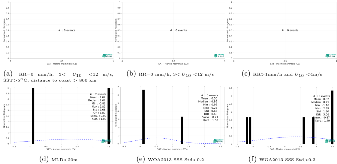
Figure 13: Normalized histogram of \Delta SSS (SMOS SSS L2Q v331 - 0.25 Deg (CATDS-CPDC) - Marine mammals) for 6 different subdatasets corresponding to: RR=0 mm/h, 3 < U_{10} < 12 m/s, SST > 5°C, distance to coast > 800 km (a), RR=0 mm/h, 3 < U_{10} < 12 m/s (b), RR > 1mm/h and U_{10} < 4 m/s (c), MLD < 20m (d), WOA2013 SSS Std < 0.2 (e), WOA2013 SSS Std > 0.2 (f).
