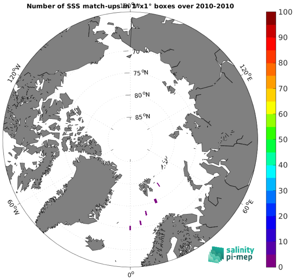
Figure 4: Number of SSS match-ups between Marine mammals SSS and the SMOS SSS L2Q v331 - 0.25 Deg (CATDS-CPDC) SSS product for the Arctic Ocean Pi-MEP region over 1^{\circ} \times 1^{\circ} boxes and for the full satellite product period.
