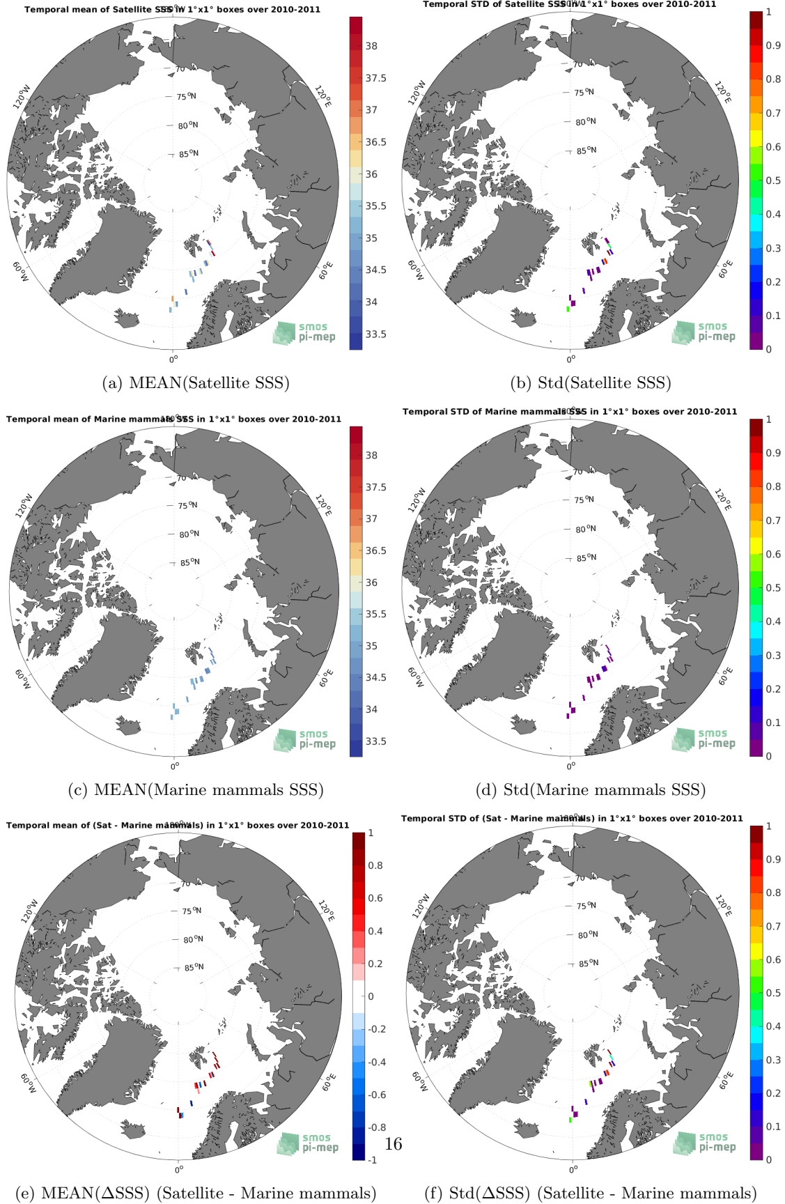
Figure 6: Temporal mean (left) and Std (right) of SSS from SMOS SSS L2Q v331 - 0.25 Deg (CATDS-CPDC) (top), Marine mammals (middle), and of \Delta SSS (Satellite - Marine mammals). Only match-up pairs are used to generate these maps.
