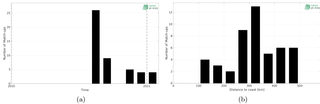
Figure 1: Number of match-ups between Marine mammals and SMOS SSS L2Q v331 - 0.25 Deg (CATDS-CPDC) SSS as a function of time (a) and as function of the distance to coast (b) over the Arctic Ocean Pi-MEP region and for the full satellite product period.
