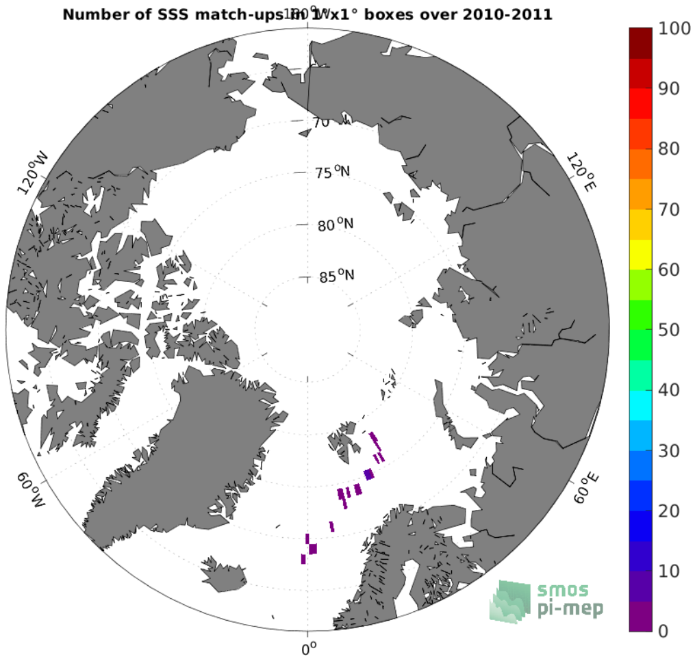
Figure 4: Number of SSS match-ups between Marine mammals SSS and the SMOS SSS L2Q v331 - 0.25 Deg (CATDS-CPDC) SSS product for the Arctic Ocean Pi-MEP region over 1^\circ \times 1^\circ boxes and for the full satellite product period.
