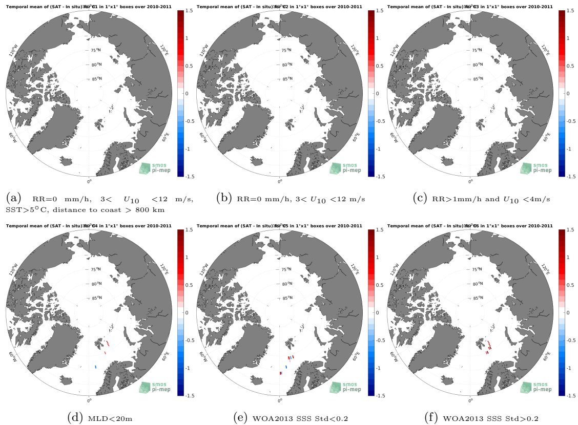
Figure 12: Temporal mean gridded over spatial boxes of size 1^{\circ}\times 1^{\circ} of \Delta\text{SSS} (SMOS SSS L2Q v331 - 0.25 Deg (CATDS-CPDC) - Marine mammals) for 6 different subdatasets corresponding to:RR=0 mm/h, 3 < U_{10} < 12 m/s, SST >5^{\circ}\text{C} , distance to coast > 800 km (a), RR=0 mm/h, 3 < U_{10} < 12 m/s (b), RR >1\text{mm/h} and U_{10} < 4\text{m/s} (c),MLD <20\text{m} (d),WOA2013 SSS Std <0.2 (e),WOA2013 SSS Std >0.2 (f).
