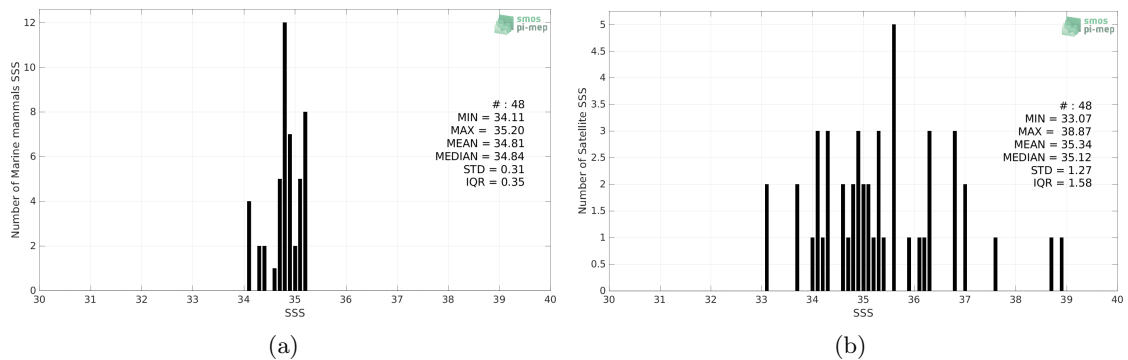
Figure 2: Histograms of SSS from Marine mammals (a) and SMOS SSS L2Q v331 - 0.25 Deg (CATDS-CPDC) (b) considering all match-up pairs per bins of 0.1 over the Arctic Ocean Pi-MEP region and for the full satellite product period.
