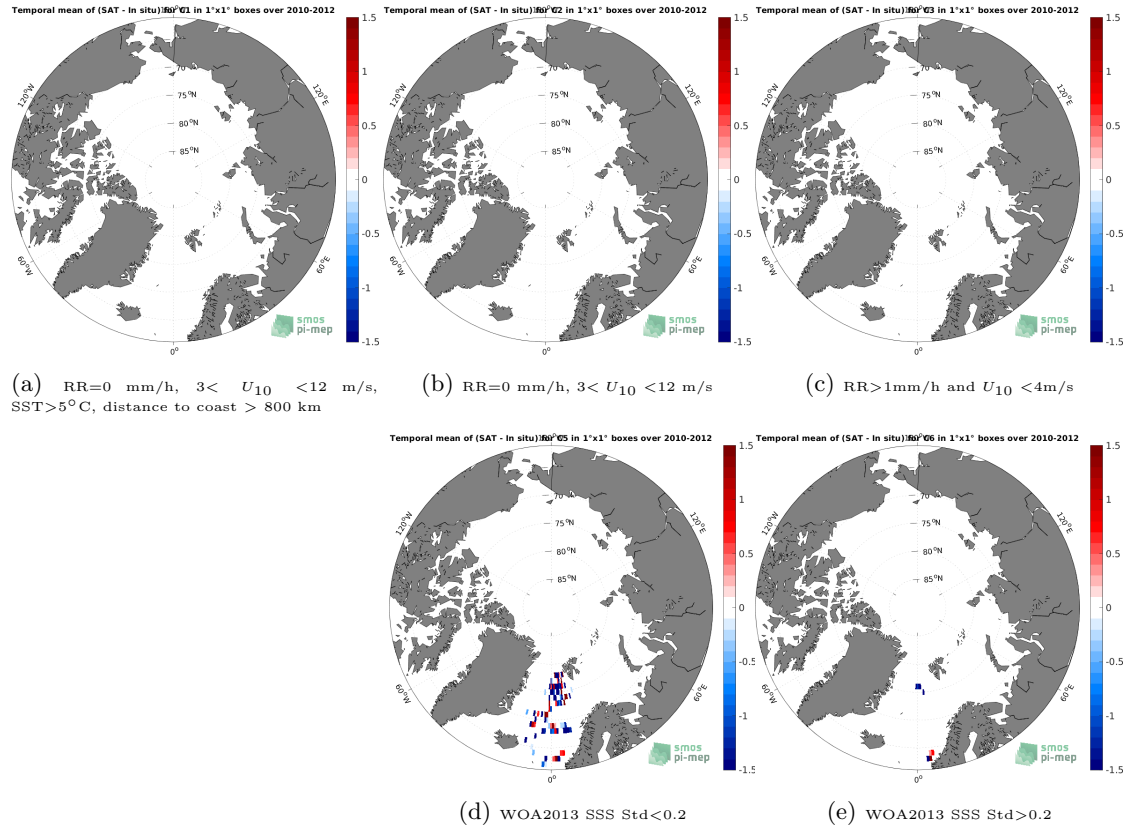
Figure 11: Temporal mean gridded over spatial boxes of size 1^{\circ}\times 1^{\circ} of \Delta\text{SSS} (SMOS SSS L2Q v331 - 0.25 Deg (CATDS-CPDC) - Surface drifters) for 5 different subdatasets corresponding to: RR=0 mm/h, 3 < U_{10} < 12 m/s, SST > 5^{\circ}\text{C} , distance to coast > 800 km (a), RR=0 mm/h, 3 < U_{10} < 12 m/s (b), RR > 1 mm/h and U_{10} < 4 m/s (c), WOA2013 SSS Std < 0.2 (d), WOA2013 SSS Std > 0.2 (e).
