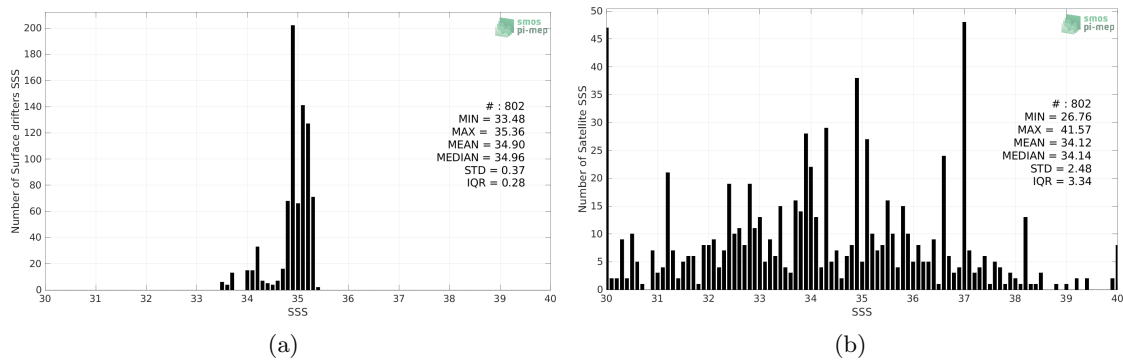
Figure 2: Histograms of SSS from Surface drifters (a) and SMOS SSS L2Q v331 - 0.25 Deg (CATDS-CPDC) (b) considering all match-up pairs per bins of 0.1 over the Arctic Ocean Pi-MEP region and for the full satellite product period.
