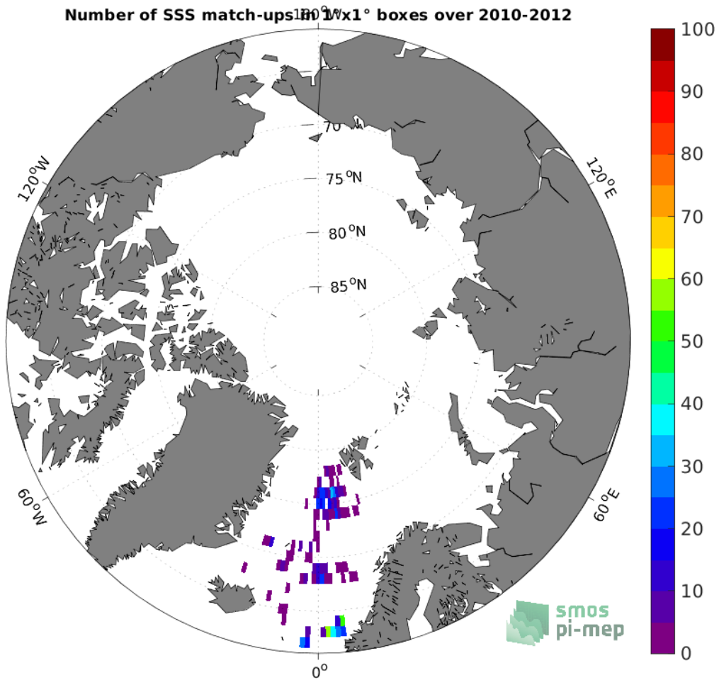
Figure 3: Number of SSS match-ups between Surface drifters SSS and the SMOS SSS L2Q v331 - 0.25 Deg (CATDS-CPDC) SSS product for the Arctic Ocean Pi-MEP region over 1^\circ \times 1^\circ boxes and for the full satellite product period.
