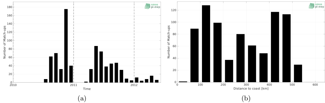
Figure 1: Number of match-ups between Surface drifters and SMOS SSS L2Q v331 - 0.25 Deg (CATDS-CPDC) SSS as a function of time (a) and as function of the distance to coast (b) over the Arctic Ocean Pi-MEP region and for the full satellite product period.
