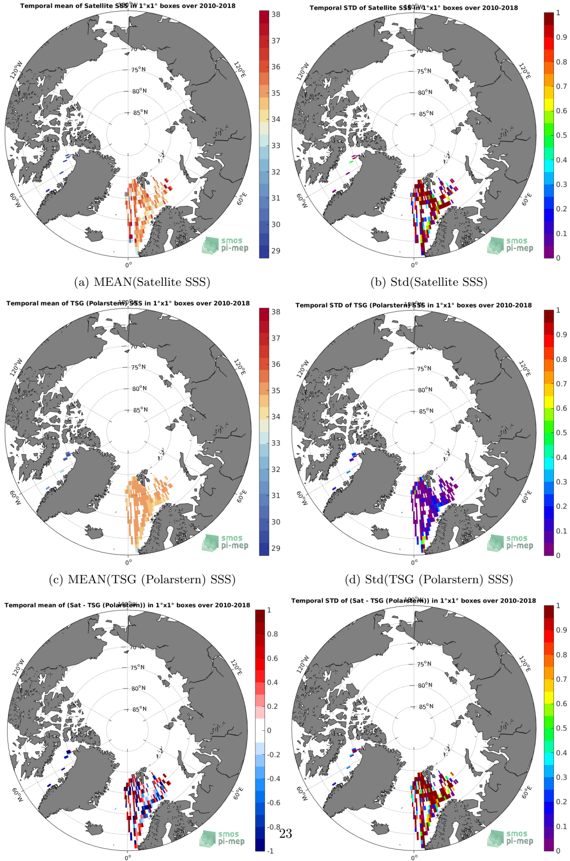
(e) MEAN( \Delta SSS) (Satellite - TSG (Polarstern))
