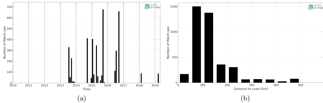
Figure 1: Number of match-ups between TSG (LEGOS-DM) and SMOS SSS L2Q v330 - 0.25 Deg (CATDS-CPDC) SSS as a function of time (a) and as function of the distance to coast (b) over the Arctic Ocean Pi-MEP region and for the full satellite product period.
