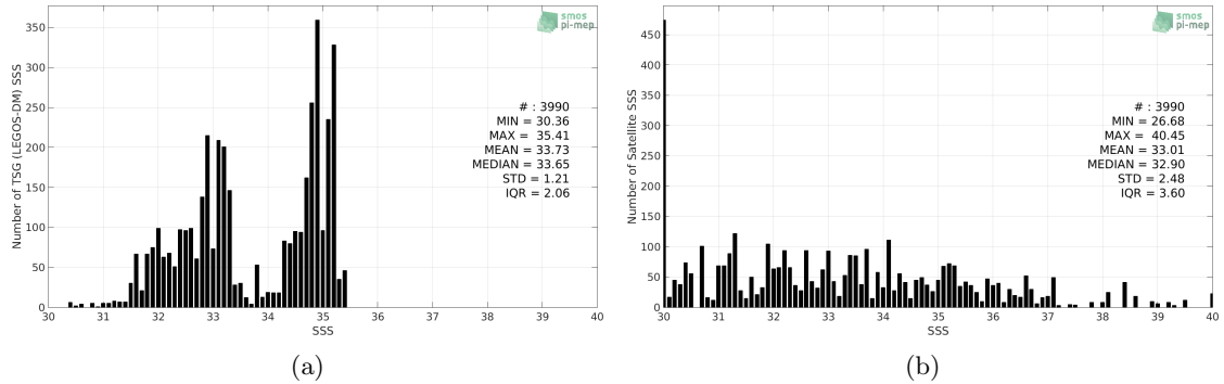
Figure 2: Histograms of SSS from TSG (LEGOS-DM) (a) and SMOS SSS L2Q v330 - 0.25 Deg (CATDS-CPDC) (b) considering all match-up pairs per bins of 0.1 over the Arctic Ocean Pi-MEP region and for the full satellite product period.
