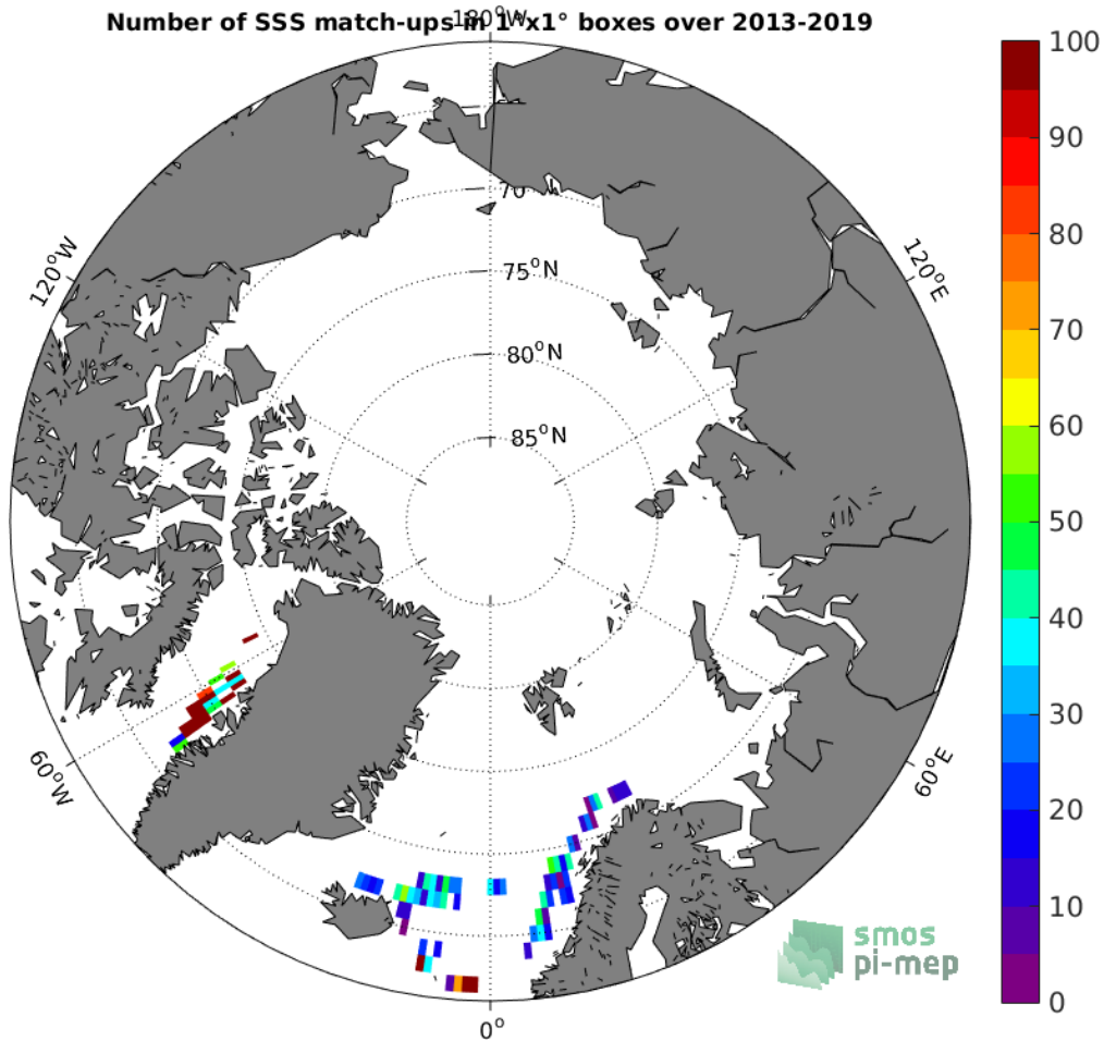
Figure 4: Number of SSS match-ups between TSG (LEGOS-DM) SSS and the SMOS SSS L2Q v330 - 0.25 Deg (CATDS-CPDC) SSS product for the Arctic Ocean Pi-MEP region over 1^\circ \times 1^\circ boxes and for the full satellite product period.
