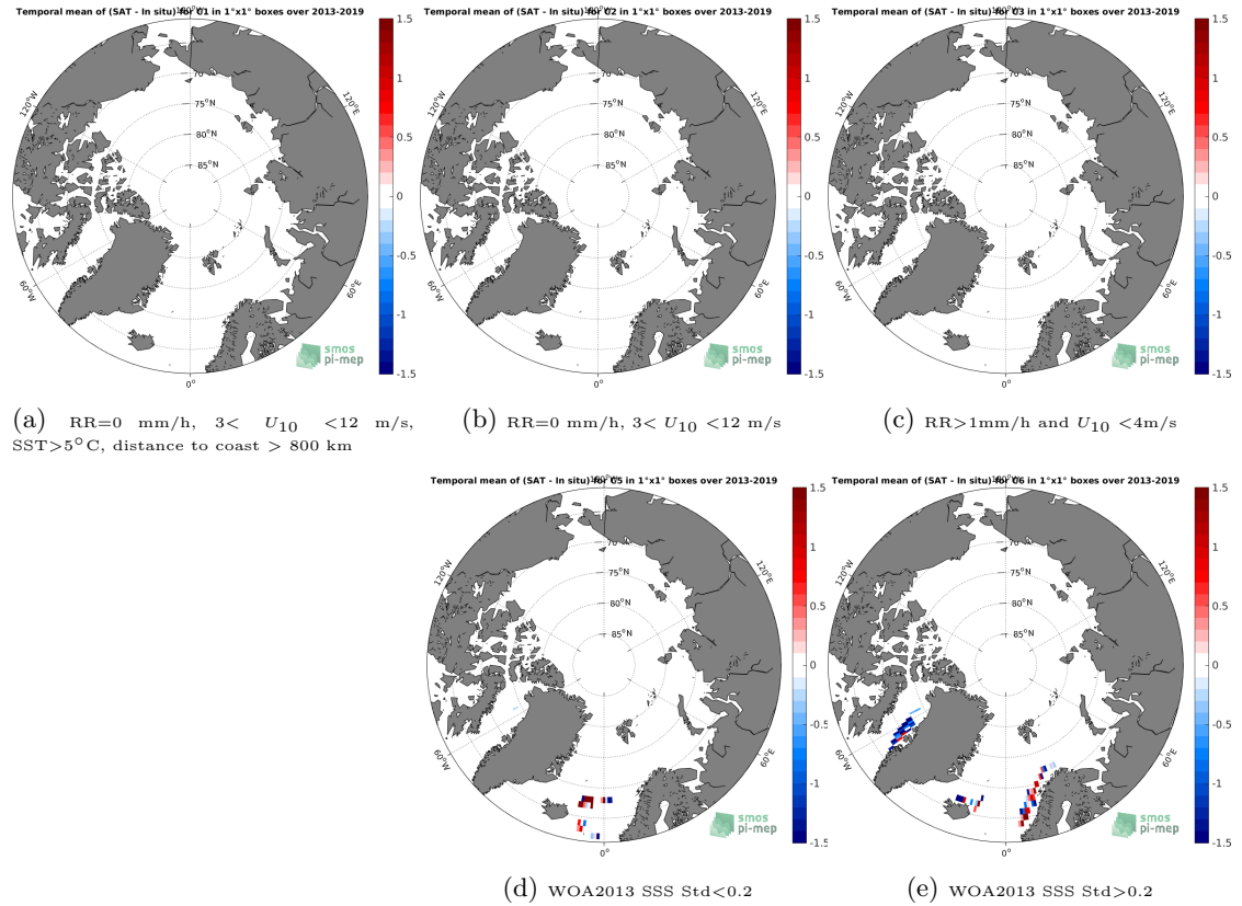
Figure 12: Temporal mean gridded over spatial boxes of size 1^{\circ}\times 1^{\circ} of \Delta\text{SSS} (SMOS SSS L2Q v330 - 0.25 Deg (CATDS-CPDC) - TSG (LEGOS-DM)) for 5 different subdatasets corresponding to:RR=0 mm/h, 3 < U_{10} < 12 m/s, SST >5^{\circ}\text{C} , distance to coast > 800 km (a), RR=0 mm/h, 3 < U_{10} < 12 m/s (b), RR >1 mm/h and U_{10} < 4 m/s (c), WOA2013 SSS Std <0.2 (d), WOA2013 SSS Std >0.2 (e).
