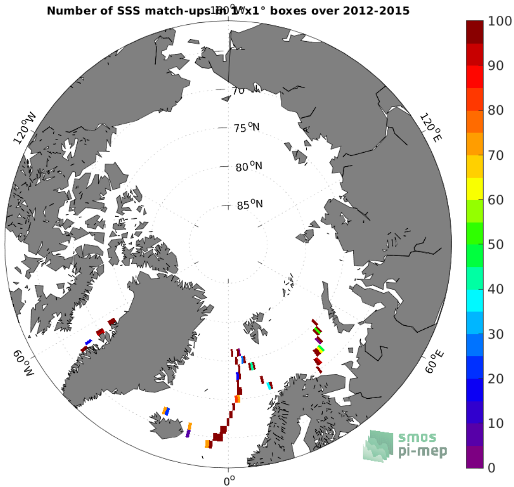
Figure 4: Number of SSS match-ups between TSG (GOSUD-Sailing-ship) SSS and the SMOS SSS L2Q v330 - 0.25 Deg (CATDS-CPDC) SSS product for the Arctic Ocean Pi-MEP region over 1^{\circ} \times 1^{\circ} boxes and for the full satellite product period.
