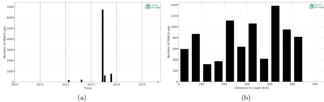
Figure 1: Number of match-ups between TSG (GOSUD-Sailing-ship) and SMOS SSS L2Q v330 - 0.25 Deg (CATDS-CPDC) SSS as a function of time (a) and as function of the distance to coast (b) over the Arctic Ocean Pi-MEP region and for the full satellite product period.
