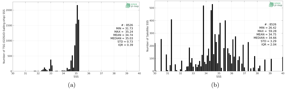
Figure 2: Histograms of SSS from TSG (GOSUD-Sailing-ship) (a) and SMOS SSS L2Q v330 - 0.25 Deg (CATDS-CPDC) (b) considering all match-up pairs per bins of 0.1 over the Arctic Ocean Pi-MEP region and for the full satellite product period.
