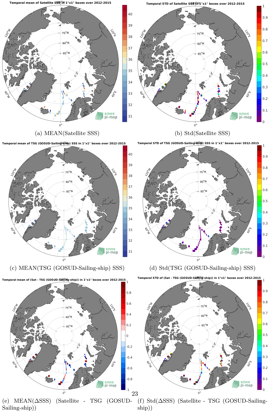
Figure 6: Temporal mean (left) and Std (right) of SSS from SMOS SSS L2Q v330 - 0.25 Deg (CATDS-CPDC) (top), TSG (GOSUD-Sailing-ship) (middle), and of \Delta SSS (Satellite - TSG (GOSUD-Sailing-ship)). Only match-up pairs are used to generate these maps.
