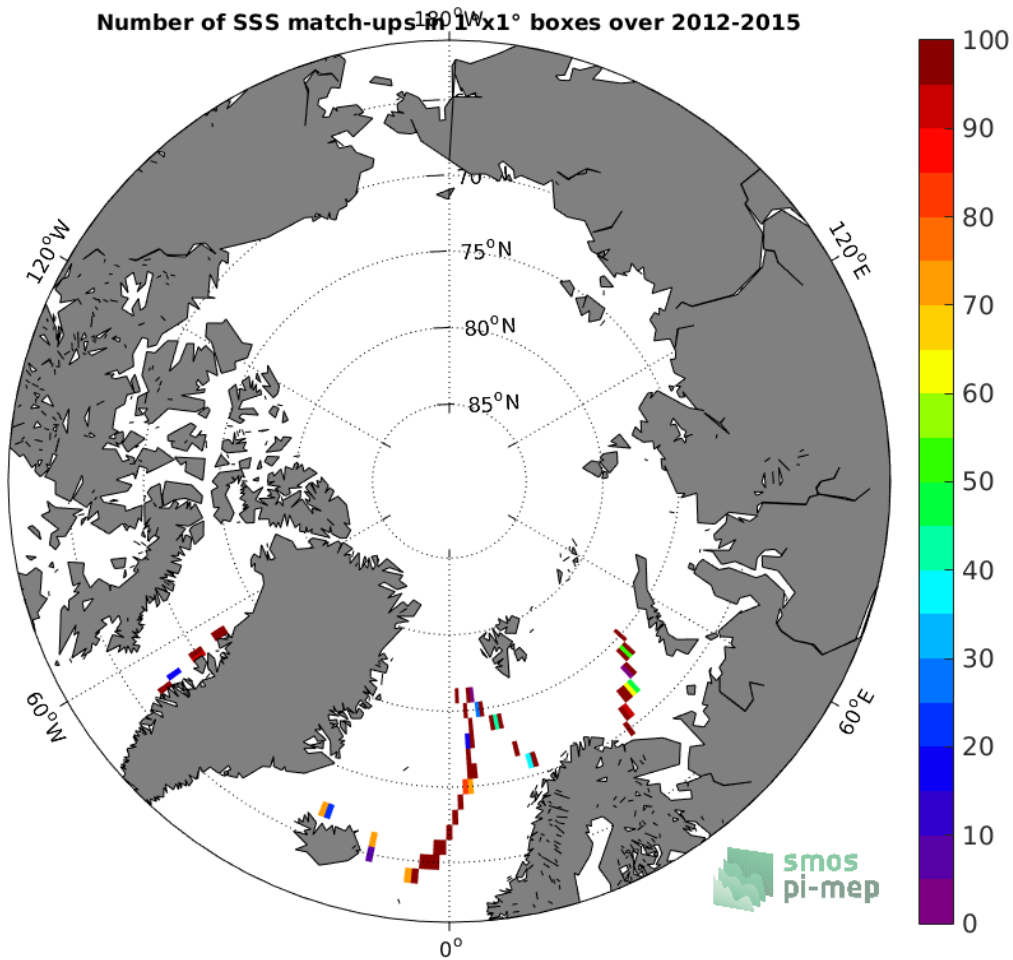
Figure 4: Number of SSS match-ups between TSG (GOSUD-Sailing-ship) SSS and the SMOS SSS L2Q v330 - 0.25 Deg (CATDS-CPDC) SSS product for the Arctic Ocean Pi-MEP region over 1^\circ \times 1^\circ boxes and for the full satellite product period.
