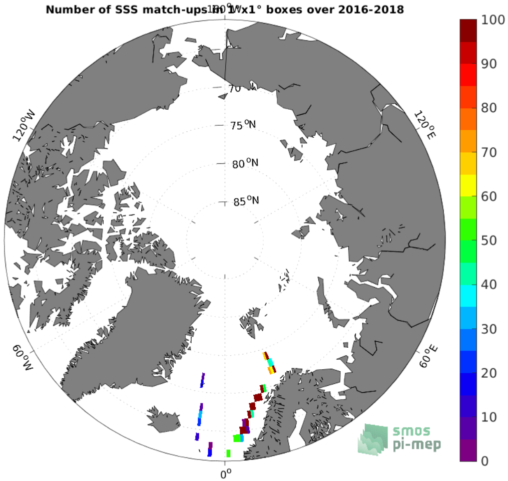
Figure 4: Number of SSS match-ups between TSG (GOSUD-Research-vessel) SSS and the SMOS SSS L2Q v330 - 0.25 Deg (CATDS-CPDC) SSS product for the Arctic Ocean Pi-MEP region over 1^\circ \times 1^\circ boxes and for the full satellite product period.
