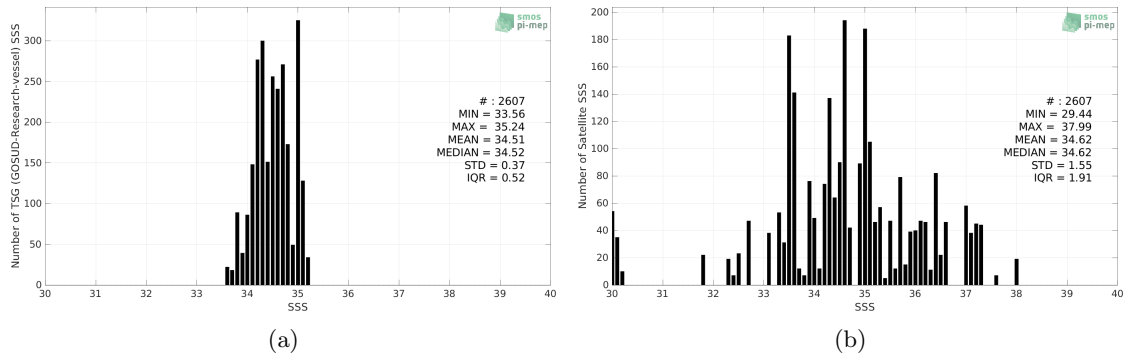
Figure 2: Histograms of SSS from TSG (GOSUD-Research-vessel) (a) and SMOS SSS L2Q v330 - 0.25 Deg (CATDS-CPDC) (b) considering all match-up pairs per bins of 0.1 over the Arctic Ocean Pi-MEP region and for the full satellite product period.
