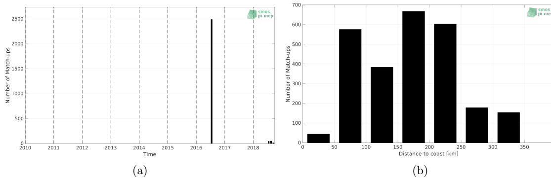
Figure 1: Number of match-ups between TSG (GOSUD-Research-vessel) and SMOS SSS L2Q v330 - 0.25 Deg (CATDS-CPDC) SSS as a function of time (a) and as function of the distance to coast (b) over the Arctic Ocean Pi-MEP region and for the full satellite product period.
