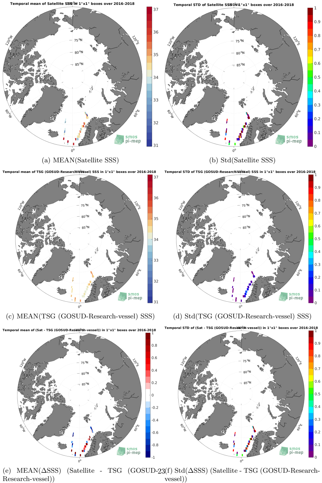
Figure 6: Temporal mean (left) and Std (right) of SSS from SMOS SSS L2Q v330 - 0.25 Deg (CATDS-CPDC) (top), TSG (GOSUD-Research-vessel) (middle), and of \Delta SSS (Satellite - TSG (GOSUD-Research-vessel)). Only match-up pairs are used to generate these maps.
