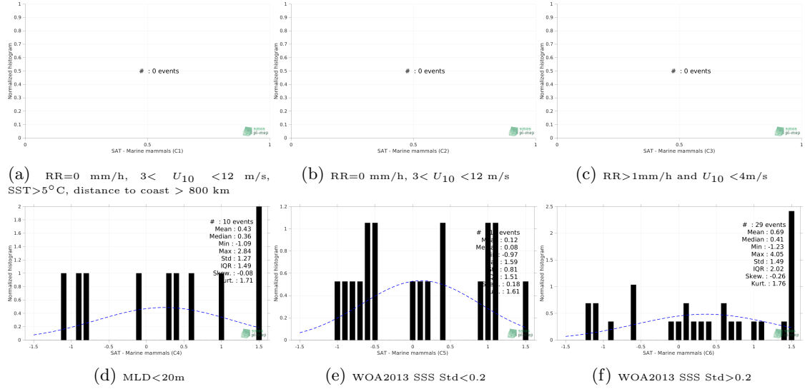
Figure 13: Normalized histogram of \Delta SSS (SMOS SSS L2Q v330 - 0.25 Deg (CATDS-CPDC) - Marine mammals) for 6 different subdatasets corresponding to: RR=0 mm/h, 3 < U_{10} < 12 m/s, SST > 5°C, distance to coast > 800 km (a), RR=0 mm/h, 3 < U_{10} < 12 m/s (b), RR > 1mm/h and U_{10} < 4 m/s (c), MLD < 20m (d), WOA2013 SSS Std < 0.2 (e), WOA2013 SSS Std > 0.2 (f).
