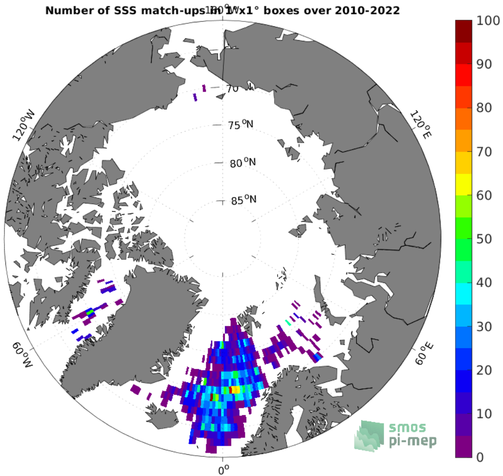
Figure 4: Number of SSS match-ups between Argo SSS and the SMOS SSS L2Q v330 - 0.25 Deg (CATDS-CPDC) SSS product for the Arctic Ocean Pi-MEP region over 1^\circ \times 1^\circ boxes and for the full satellite product period.
