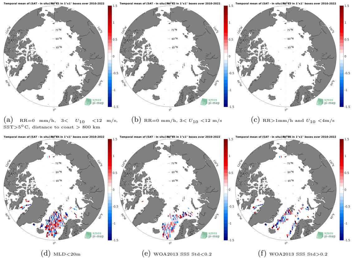
Figure 12: Temporal mean gridded over spatial boxes of size 1^{\circ}\times 1^{\circ} of \Delta\text{SSS} (SMOS SSS L2Q v330 - 0.25 Deg (CATDS-CPDC) - Argo) for 6 different subdatasets corresponding to:RR=0 mm/h, 3 < U_{10} < 12 m/s, SST >5^{\circ}\text{C} , distance to coast > 800 km (a), RR=0 mm/h, 3 < U_{10} < 12 m/s (b), RR >1 mm/h and U_{10} < 4 m/s (c),MLD <20 m (d),WOA2013 SSS Std <0.2 (e),WOA2013 SSS Std >0.2 (f).
