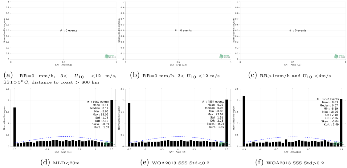
Figure 13: Normalized histogram of \Delta SSS (SMOS SSS L2Q v330 - 0.25 Deg (CATDS-CPDC) - Argo) for 6 different subdatasets corresponding to: RR=0 mm/h, 3 < U_{10} < 12 m/s, SST > 5°C, distance to coast > 800 km (a), RR=0 mm/h, 3 < U_{10} < 12 m/s (b), RR > 1mm/h and U_{10} < 4 m/s (c), MLD < 20m (d), WOA2013 SSS Std < 0.2 (e), WOA2013 SSS Std > 0.2 (f).
