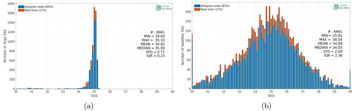
Figure 2: Histograms of SSS from Argo (a) and SMOS SSS L2Q v330 - 0.25 Deg (CATDS-CPDC) (b) considering all match-up pairs per bins of 0.1 over the Arctic Ocean Pi-MEP region and for the full satellite product period.
