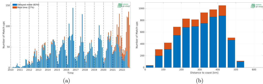
Figure 1: Number of match-ups between Argo and SMOS SSS L2Q v330 - 0.25 Deg (CATDS-CPDC) SSS as a function of time (a) and as function of the distance to coast (b) over the Arctic Ocean Pi-MEP region and for the full satellite product period.
