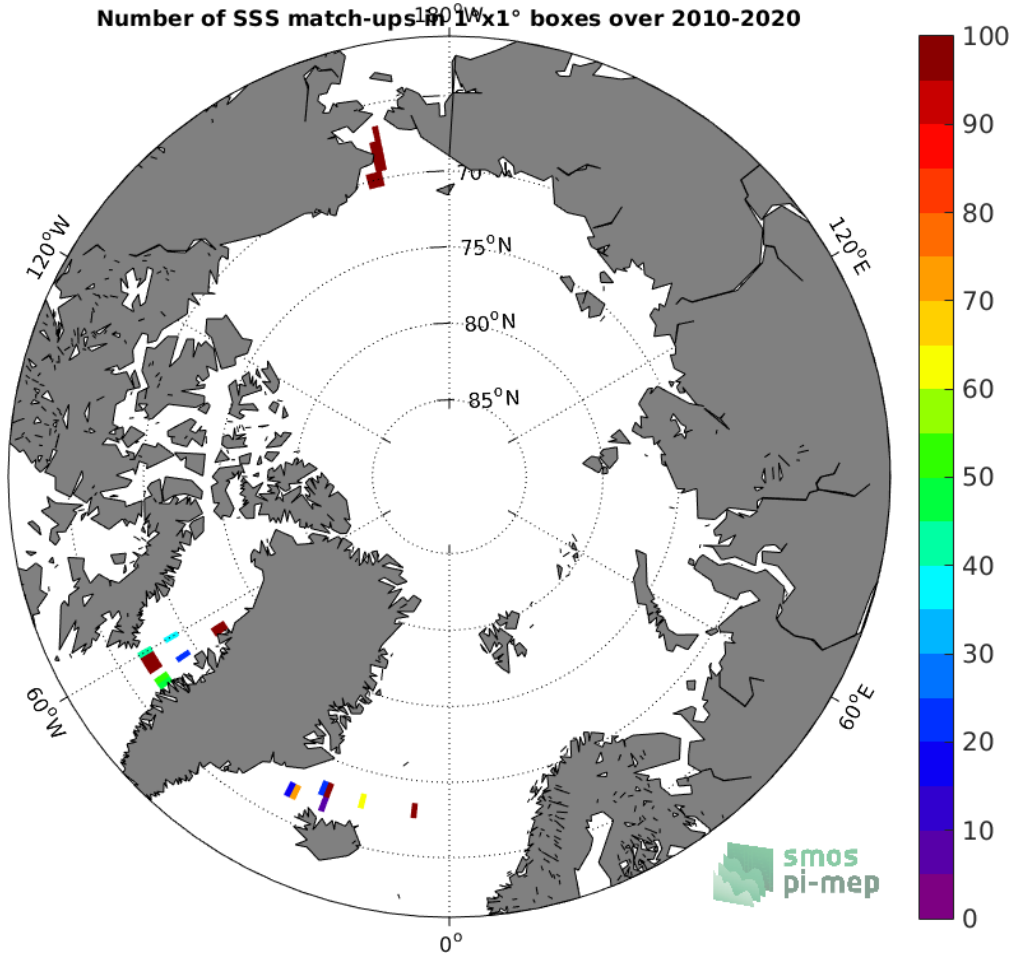
Figure 4: Number of SSS match-ups between TSG (SAMOS) SSS and the SMOS SSS L2Q v321 - 0.25 Deg (CATDS-CPDC) SSS product for the Arctic Ocean Pi-MEP region over 1^\circ \times 1^\circ boxes and for the full satellite product period.
