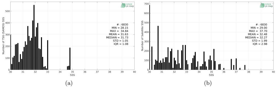
Figure 2: Histograms of SSS from TSG (SAMOS) (a) and SMOS SSS L2Q v321 - 0.25 Deg (CATDS-CPDC) (b) considering all match-up pairs per bins of 0.1 over the Arctic Ocean Pi-MEP region and for the full satellite product period.
