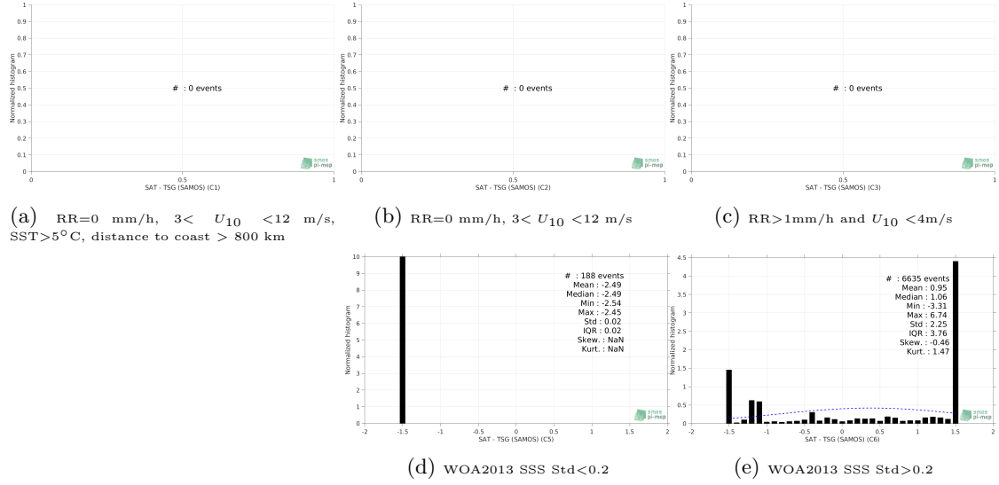
Figure 13: Normalized histogram of \Delta\text{SSS} (SMOS SSS L2Q v321 - 0.25 Deg (CATDS-CPDC) - TSG (SAMOS)) for 5 different subdatasets corresponding to: RR=0 mm/h, 3 < U_{10} < 12 m/s, SST > 5^\circ\text{C} , distance to coast > 800 km (a), RR=0 mm/h, 3 < U_{10} < 12 m/s (b), RR > 1 mm/h and U_{10} < 4 m/s (c), WOA2013 SSS Std < 0.2 (d), WOA2013 SSS Std > 0.2 (e).
