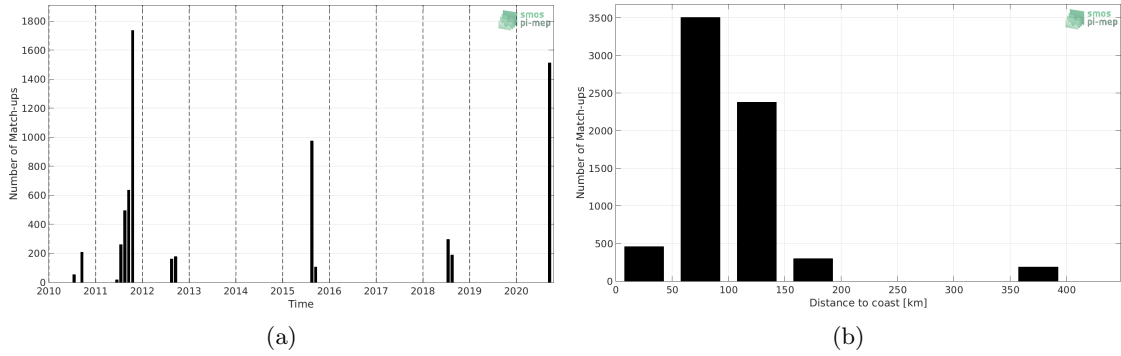
Figure 1: Number of match-ups between TSG (SAMOS) and SMOS SSS L2Q v321 - 0.25 Deg (CATDS-CPDC) SSS as a function of time (a) and as function of the distance to coast (b) over the Arctic Ocean Pi-MEP region and for the full satellite product period.
