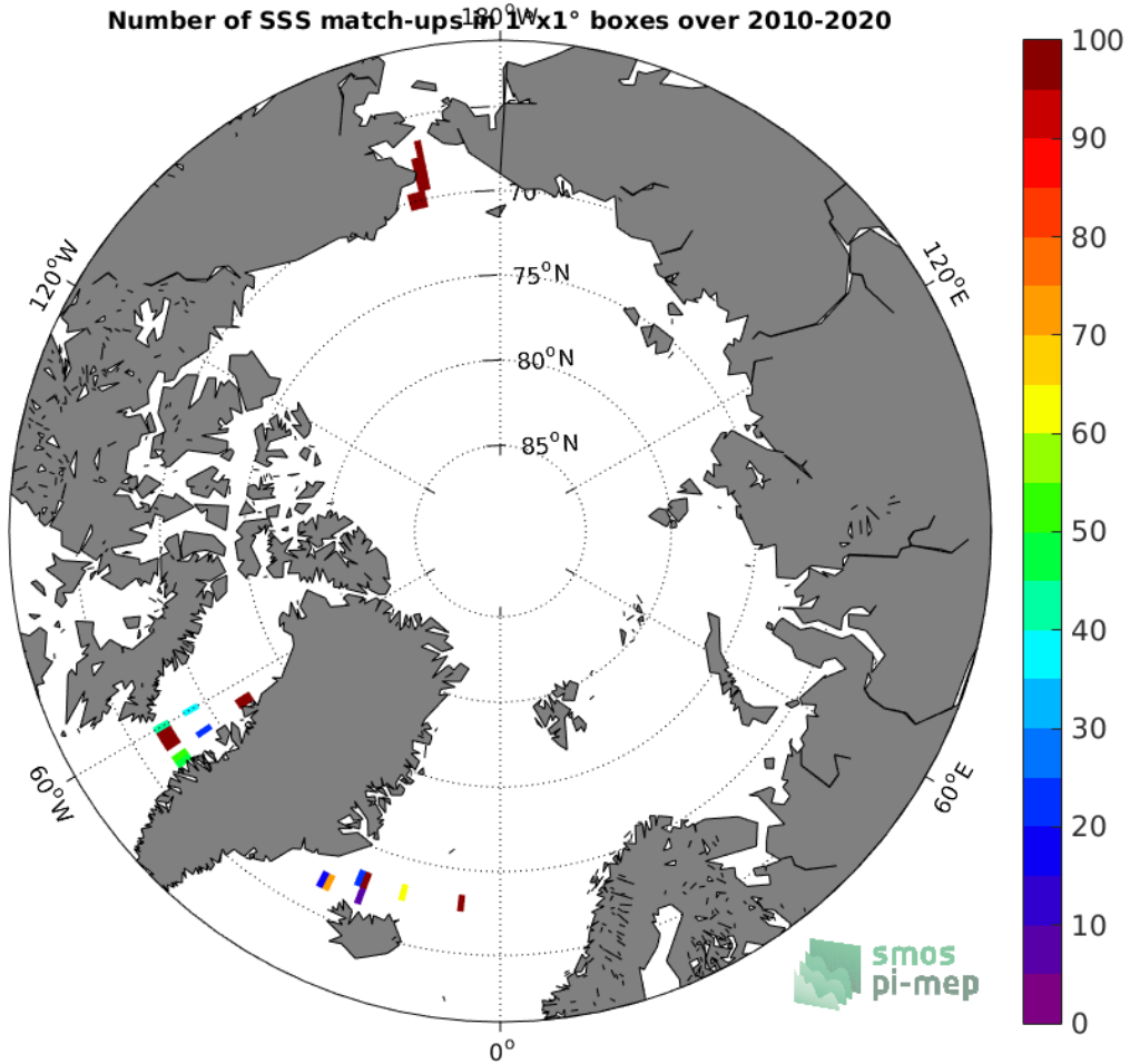
Figure 4: Number of SSS match-ups between TSG (SAMOS) SSS and the SMOS SSS L2Q v321 - 0.25 Deg (CATDS-CPDC) SSS product for the Arctic Ocean Pi-MEP region over 1°x1° boxes and for the full satellite product period.
