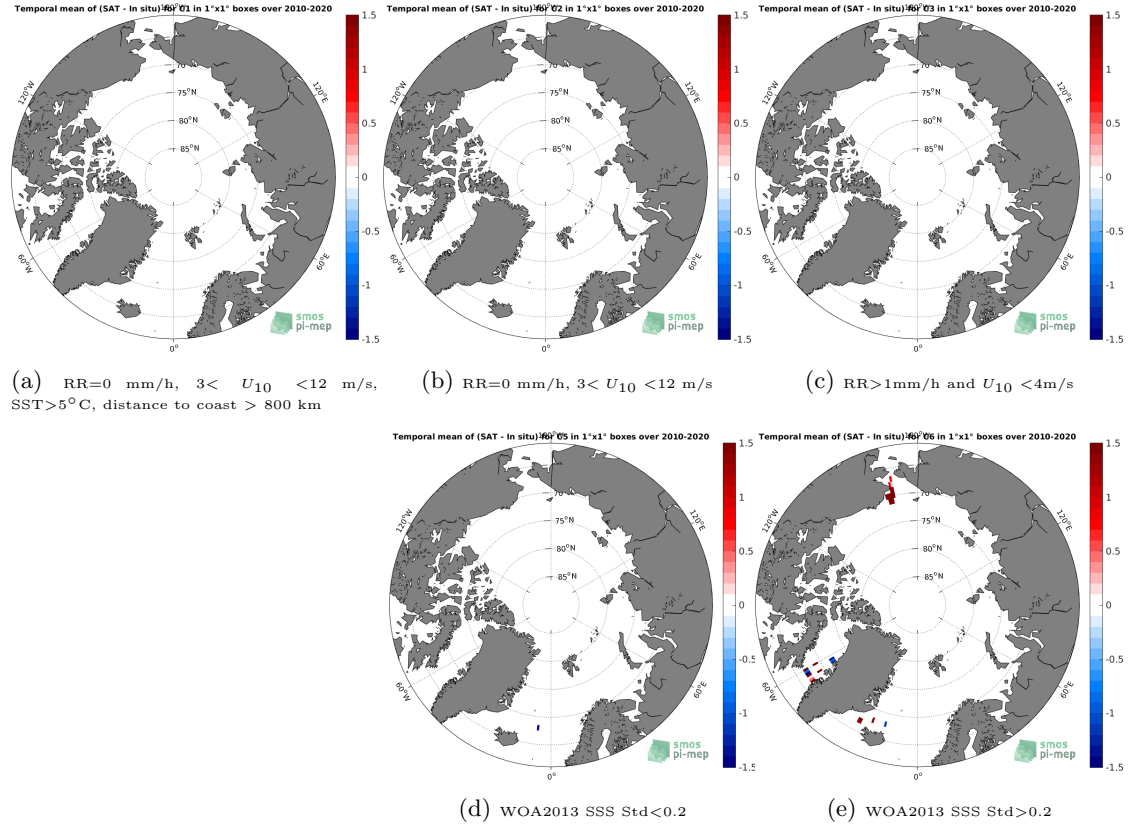
Figure 12: Temporal mean gridded over spatial boxes of size 1^{\circ}\times 1^{\circ} of \Delta\text{SSS} (SMOS SSS L2Q v321 - 0.25 Deg (CATDS-CPDC) - TSG (SAMOS)) for 5 different subdatasets corresponding to:RR=0 mm/h, 3 < U_{10} < 12 m/s, SST >5^{\circ}\text{C} , distance to coast > 800 km (a), RR=0 mm/h, 3 < U_{10} < 12 m/s (b), RR >1 mm/h and U_{10} < 4 m/s (c), WOA2013 SSS Std <0.2 (d), WOA2013 SSS Std >0.2 (e).
