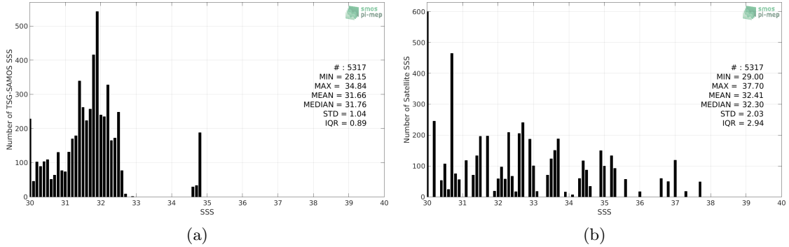
Figure 2: Histograms of SSS from TSG-SAMOS (a) and SMOS L2Q v321 - 0.25 Deg (CATDS-CPDC) (b) considering all match-up pairs per bins of 0.1 over the Arctic Ocean Pi-MEP region and for the full satellite product period.
