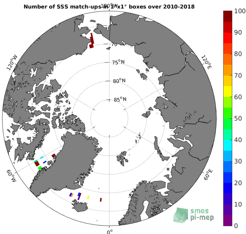
Figure 4: Number of SSS match-ups between TSG-SAMOS SSS and the SMOS L2Q v321 - 0.25 Deg (CATDS-CPDC) SSS product for the Arctic Ocean Pi-MEP region over 1^\circ \times 1^\circ boxes and for the full satellite product period.
