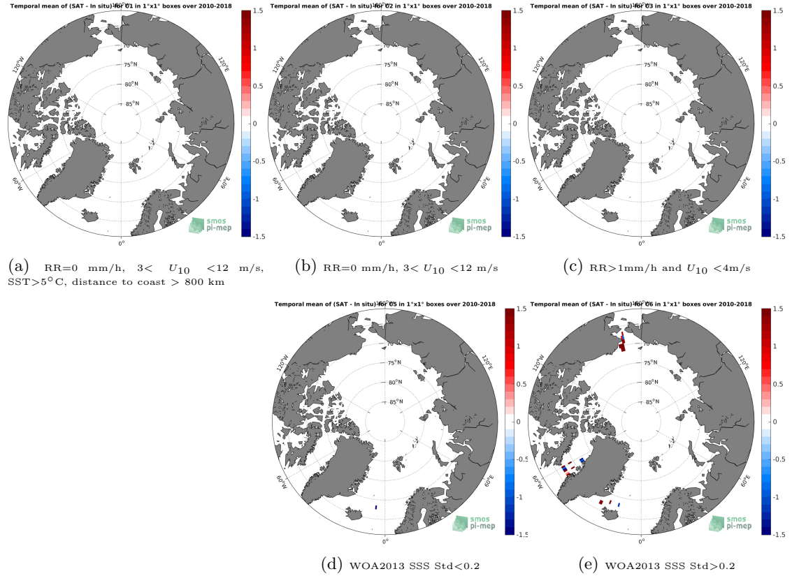
Figure 12: Temporal mean gridded over spatial boxes of size 1^{\circ}\times 1^{\circ} of \Delta\text{SSS} (SMOS L2Q v321 - 0.25 Deg (CATDS-CPDC) - TSG-SAMOS) for 5 different subdatasets corresponding to: \text{RR}=0 mm/h, 3 < U_{10} < 12 m/s, \text{SST} > 5^{\circ}\text{C} , distance to coast > 800 km (a), \text{RR}=0 mm/h, 3 < U_{10} < 12 m/s (b), \text{RR} > 1 mm/h and U_{10} < 4 m/s (c), WOA2013 SSS Std < 0.2 (d), WOA2013 SSS Std > 0.2 (e).
