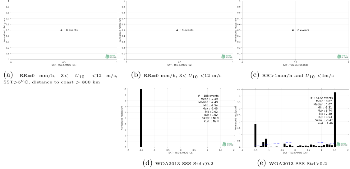
Figure 13: Normalized histogram of \Delta\text{SSS} (SMOS L2Q v321 - 0.25 Deg (CATDS-CPDC) - TSG-SAMOS) for 5 different subdatasets corresponding to: RR=0 mm/h, 3 < U_{10} < 12 m/s, SST > 5^{\circ}\text{C} , distance to coast > 800 km (a), RR=0 mm/h, 3 < U_{10} < 12 m/s (b), RR > 1\text{mm/h} and U_{10} < 4\text{m/s} (c), WOA2013 SSS Std<0.2 (d), WOA2013 SSS Std>0.2 (e).
