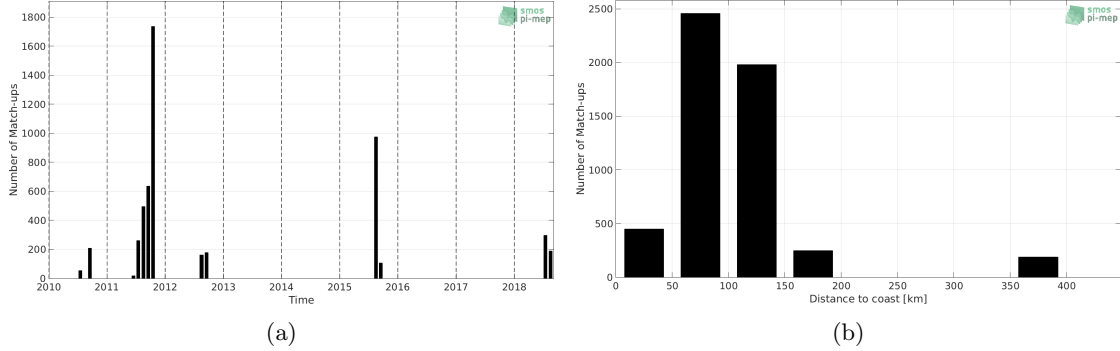
Figure 1: Number of match-ups between TSG-SAMOS and SMOS L2Q v321 - 0.25 Deg (CATDS-CPDC) SSS as a function of time (a) and as function of the distance to coast (b) over the Arctic Ocean Pi-MEP region and for the full satellite product period.
