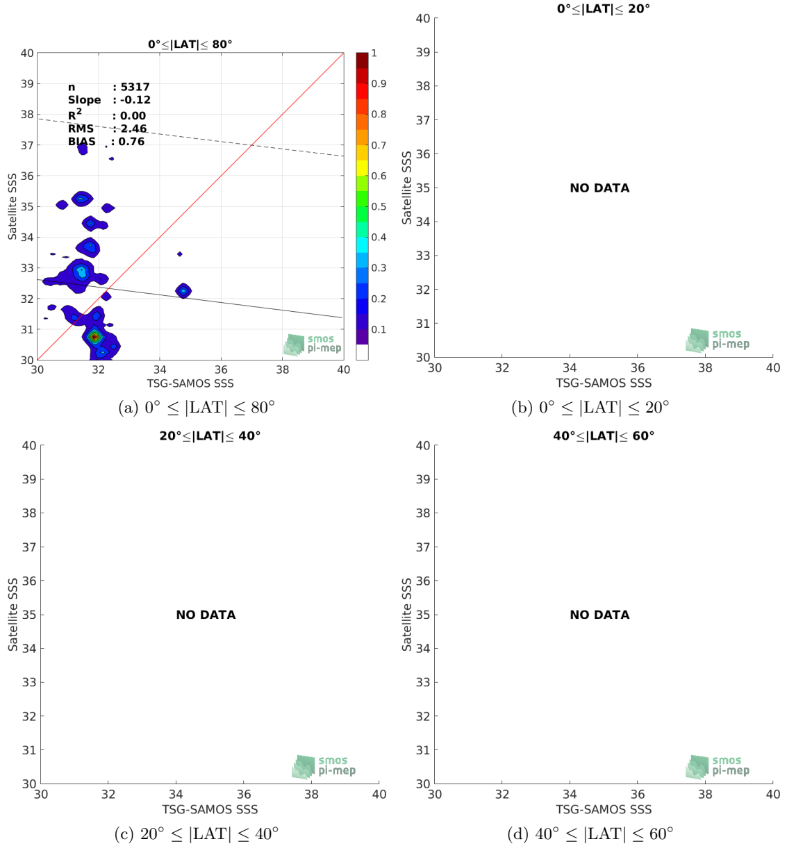
Figure 9: Contour maps of the concentration of SMOS L2Q v321 - 0.25 Deg (CATDS-CPDC') SSS (y-axis) versus TSG-SAMOS SSS (x-axis) at match-up pairs for different latitude bands. For each plot, the red line shows x=y . The black thin and dashed lines indicate a linear fit through the data cloud and the \pm 95\% confidence levels, respectively. The number match-up pairs n , the slope and R^2 coefficient of the linear fit, the root mean square (RMS) and the mean bias between satellite and in situ data are indicated for each latitude band in each plots.
