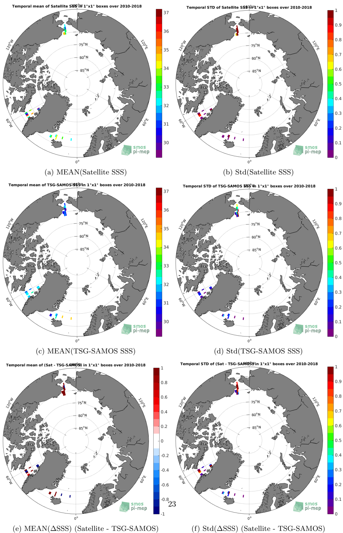
Figure 6: Temporal mean (left) and Std (right) of SSS from SMOS L2Q v321 - 0.25 Deg (CATDS-CPDC) (top), TSG-SAMOS (middle), and of \Delta SSS (Satellite - TSG-SAMOS). Only match-up pairs are used to generate these maps.
