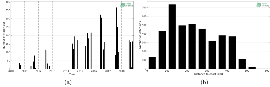
Figure 1: Number of match-ups between TSG (Polarstern) and SMOS SSS L2Q v321 - 0.25 Deg (CATDS-CPDC) SSS as a function of time (a) and as function of the distance to coast (b) over the Arctic Ocean Pi-MEP region and for the full satellite product period.
