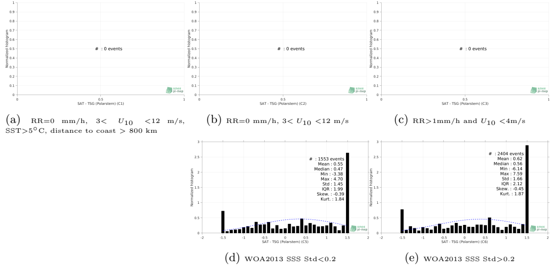
Figure 13: Normalized histogram of \Delta SSS (SMOS SSS L2Q v321 - 0.25 Deg (CATDS-CPDC) - TSG (Polarstern)) for 5 different subdatasets corresponding to: RR=0 mm/h, 3 < U_{10} < 12 m/s, SST>5°C, distance to coast > 800 km (a), RR=0 mm/h, 3 < U_{10} < 12 m/s (b), RR>1 mm/h and U_{10} < 4 m/s (c), WOA2013 SSS Std<0.2 (d), WOA2013 SSS Std>0.2 (e).
