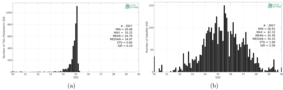
Figure 2: Histograms of SSS from TSG (Polarstern) (a) and SMOS SSS L2Q v321 - 0.25 Deg (CATDS-CPDC) (b) considering all match-up pairs per bins of 0.1 over the Arctic Ocean Pi-MEP region and for the full satellite product period.
