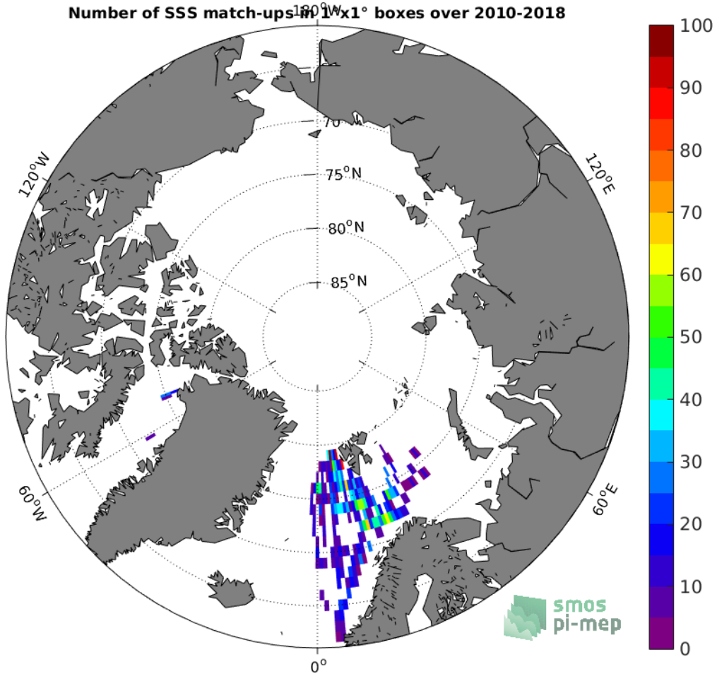
Figure 4: Number of SSS match-ups between TSG (Polarstern) SSS and the SMOS SSS L2Q v321 - 0.25 Deg (CATDS-CPDC) SSS product for the Arctic Ocean Pi-MEP region over 1°x1° boxes and for the full satellite product period.
