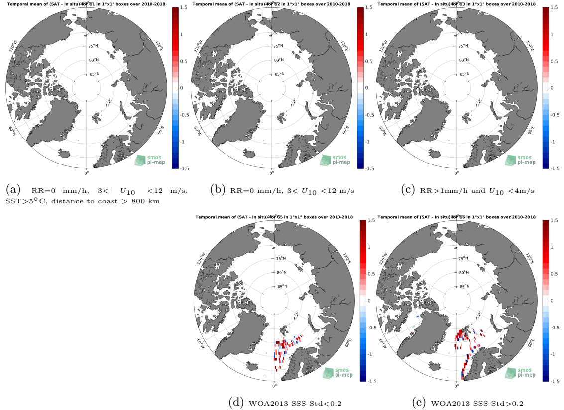
Figure 12: Temporal mean gridded over spatial boxes of size 1^{\circ}\times 1^{\circ} of \Delta\text{SSS} (SMOS SSS L2Q v321 - 0.25 Deg (CATDS-CPDC) - TSG (Polarstern)) for 5 different subdatasets corresponding to: RR=0 mm/h, 3 < U_{10} < 12 m/s, SST > 5^{\circ}\text{C} , distance to coast > 800 km (a), RR=0 mm/h, 3 < U_{10} < 12 m/s (b), RR > 1 mm/h and U_{10} < 4 m/s (c), WOA2013 SSS Std < 0.2 (d), WOA2013 SSS Std > 0.2 (e).
