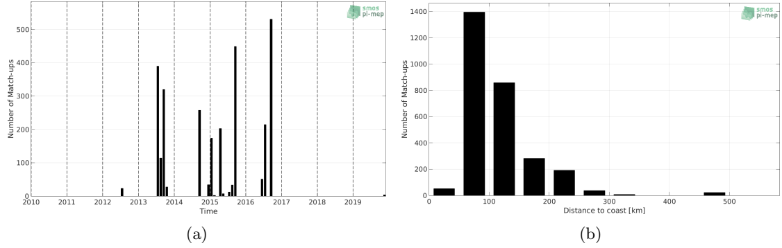
Figure 1: Number of match-ups between TSG (LEGOS-DM) and SMOS SSS L2Q v321 - 0.25 Deg (CATDS-CPDC) SSS as a function of time (a) and as function of the distance to coast (b) over the Arctic Ocean Pi-MEP region and for the full satellite product period.
