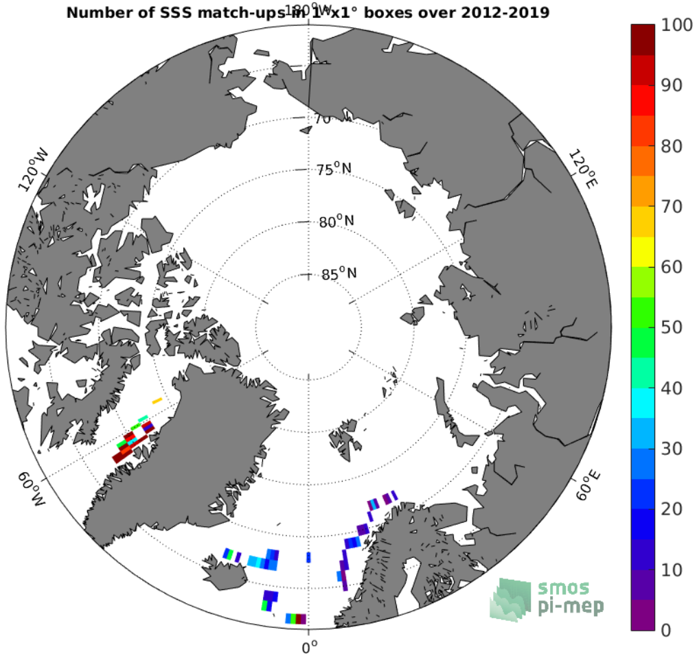
Figure 4: Number of SSS match-ups between TSG (LEGOS-DM) SSS and the SMOS SSS L2Q v321 - 0.25 Deg (CATDS-CPDC) SSS product for the Arctic Ocean Pi-MEP region over 1^\circ \times 1^\circ boxes and for the full satellite product period.
