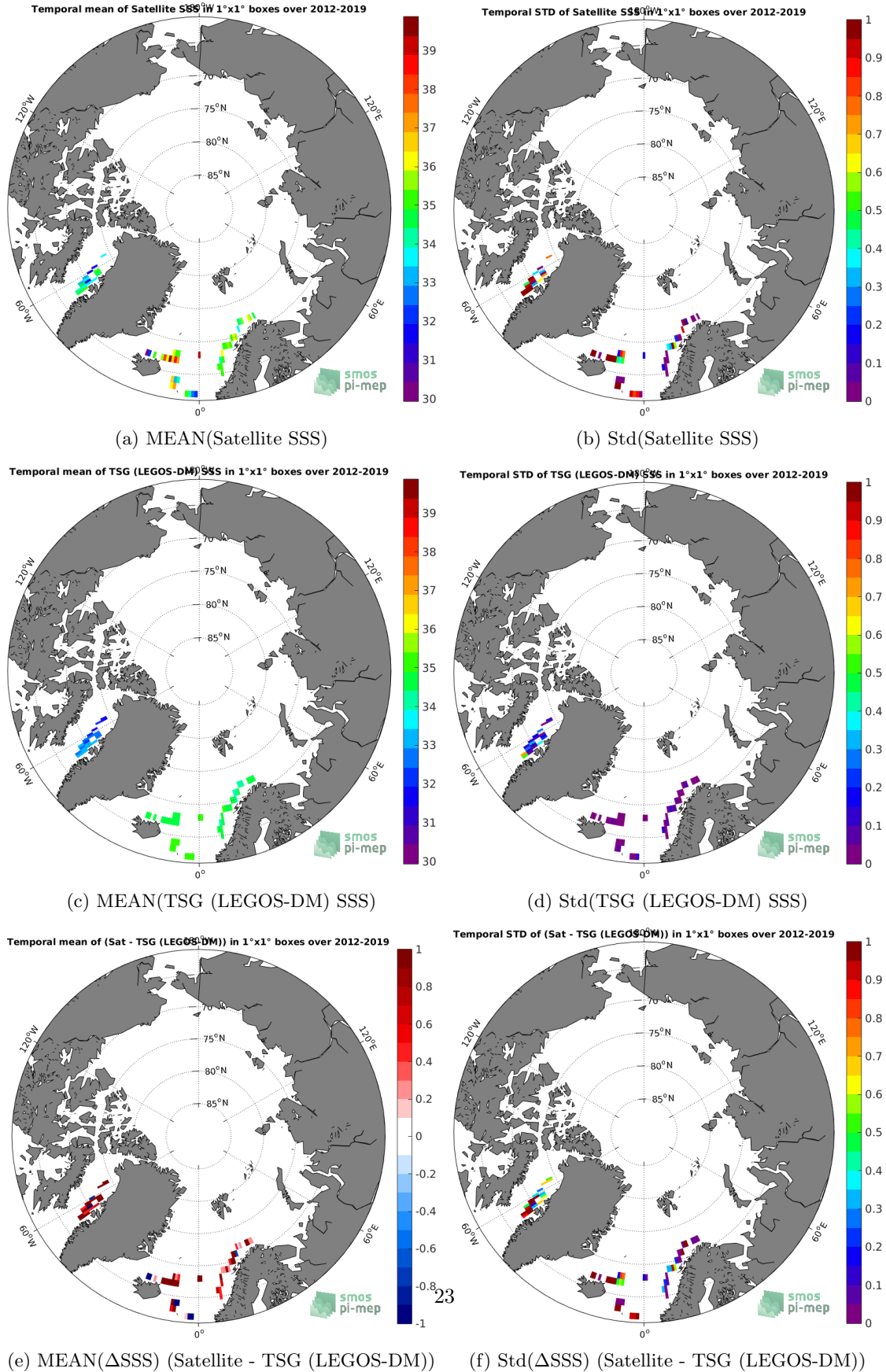
Figure 6: Temporal mean (left) and Std (right) of SSS from SMOS SSS L2Q v321 - 0.25 Deg (CATDS-CPDC) (top), TSG (LEGOS-DM) (middle), and of \Delta SSS (Satellite - TSG (LEGOS-DM)). Only match-up pairs are used to generate these maps.
