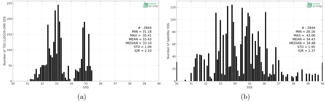
Figure 2: Histograms of SSS from TSG (LEGOS-DM) (a) and SMOS SSS L2Q v321 - 0.25 Deg (CATDS-CPDC) (b) considering all match-up pairs per bins of 0.1 over the Arctic Ocean Pi-MEP region and for the full satellite product period.
